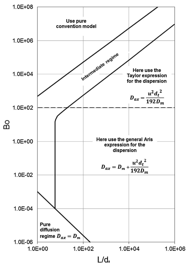
Fig. 1 – Map reporting which flow model to adopt for straight pipes. The operational point can be found on the map knowing the values of the aspect ratio of the pipe and of the Bodenstein number.
