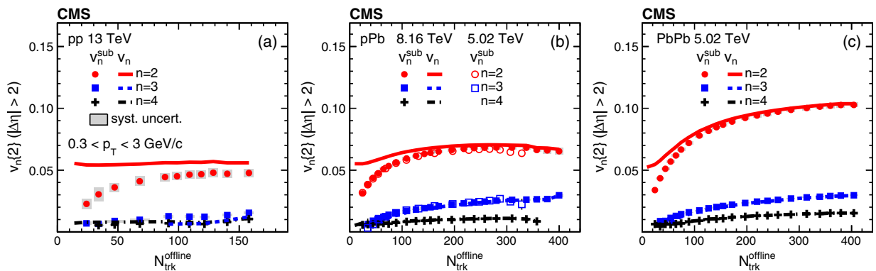
FIG. 1. The v_2 , v_3 [25], and v_4 coefficients from long-range two-particle correlations as a function of N_{\text{trk}}^{\text{offline}} in 13 TeV pp (a), 5.02 [32] and 8.16 TeV p + \text{Pb} (b), and 5.02 TeV PbPb collisions (c). The results corrected by low-multiplicity subtraction are denoted as v_n^{\text{sub}} . The lines show the v_n results before the subtraction of low-multiplicity correlations. The gray boxes represent systematic uncertainties.
