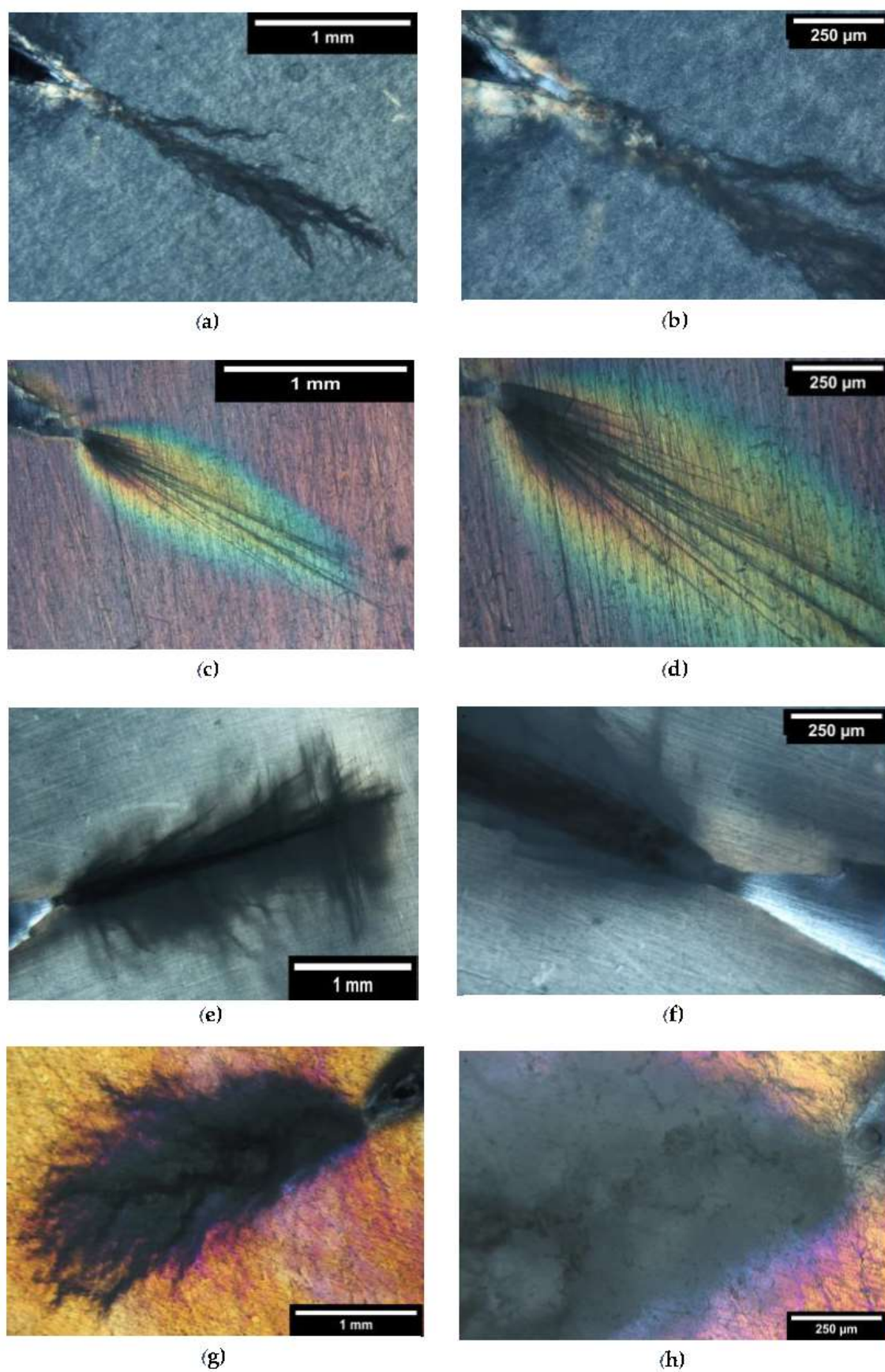
Figure 6. Cross-polarized TOM micrographs of the subcritical crack tip section after deformation for (a,b) P10, (c,d) P20, (e,f) S10, and (g,h) S20.
