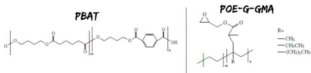
Figure 2. Chemical structure of the monomeric units of PBAT and POE-g-GMA.
