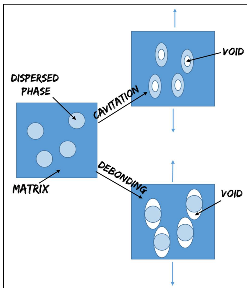
Figure 1. Cavitation and debonding mechanisms.
