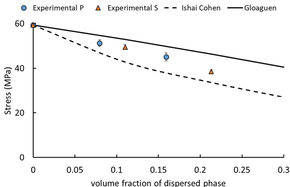
Figure 9. Stress at the yield variation with increasing of the volume percentage of PBAT: experimental data compared with predictive analytical models.
