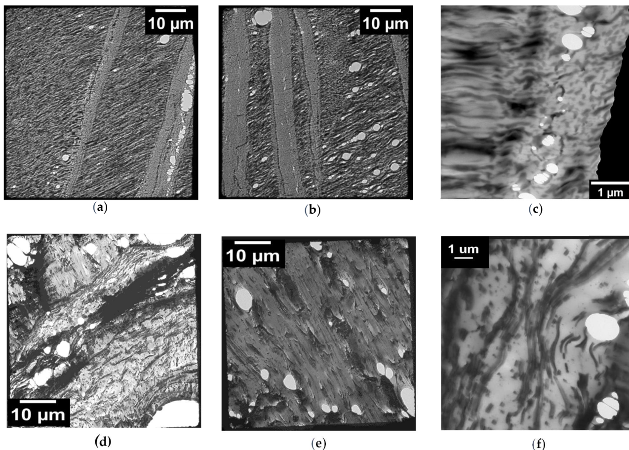
Figure 8. TEM micrographs of the subcritical crack tip section after deformation for the (a–c) P20 and (d–f) S20 blend.
