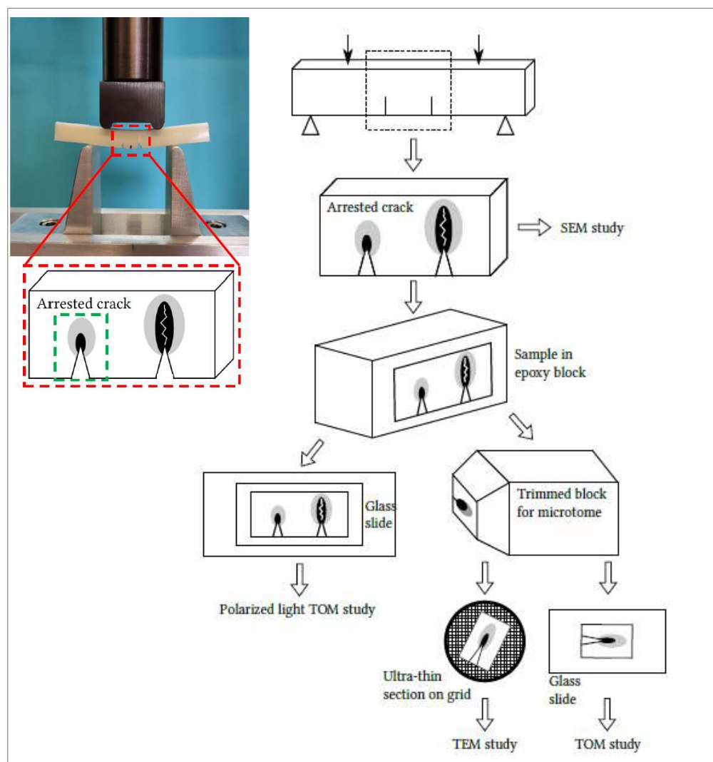
Figure 3. Schematization of SEDN-4PB configuration and of the sampling process for the different microscopy techniques.
