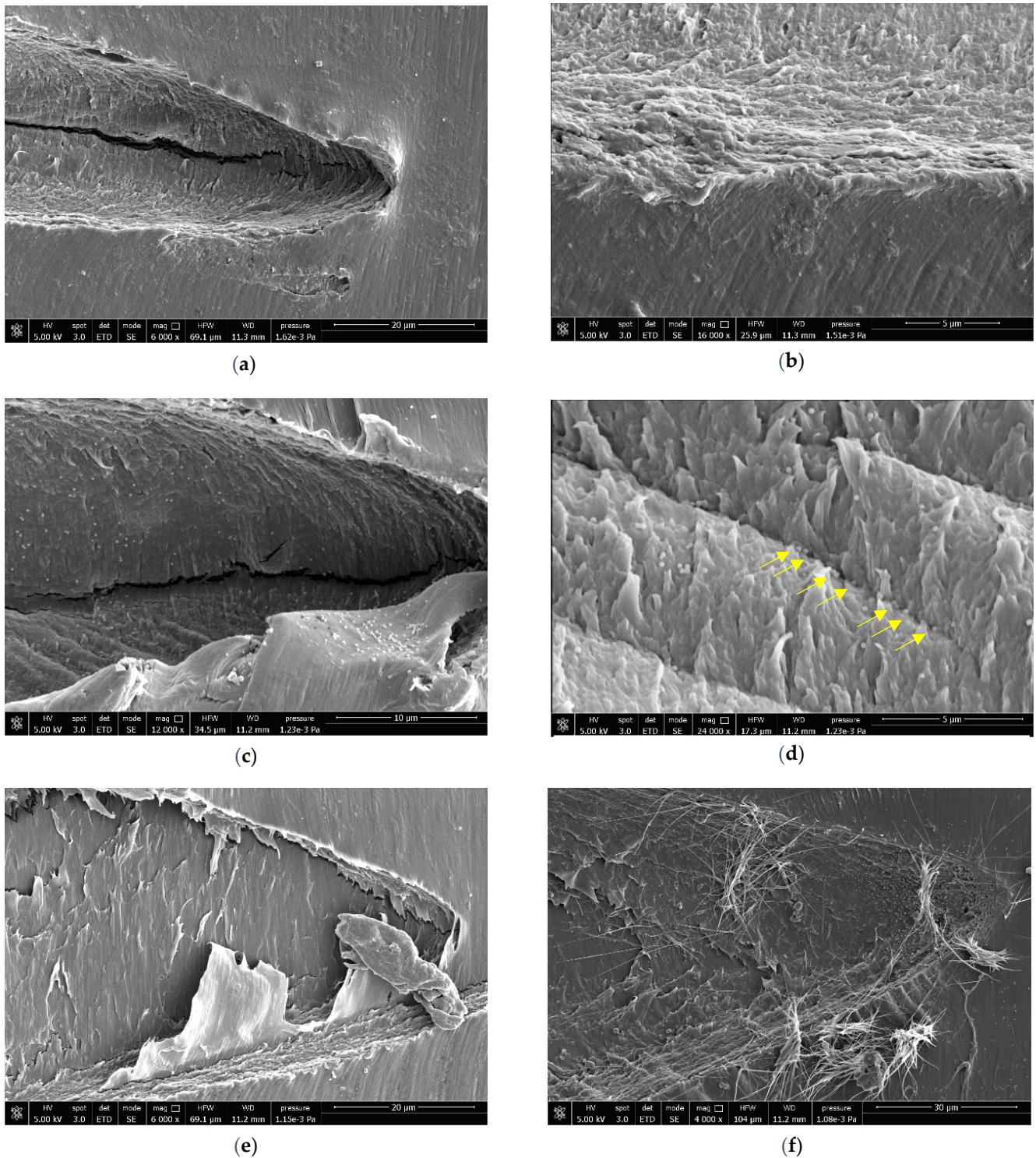
Figure 5. SEM micrographs of the arrested crack surface of the SEDN-4PB: (a,b) P10, (c,d) P20, (e) S10, and (f) S20.
