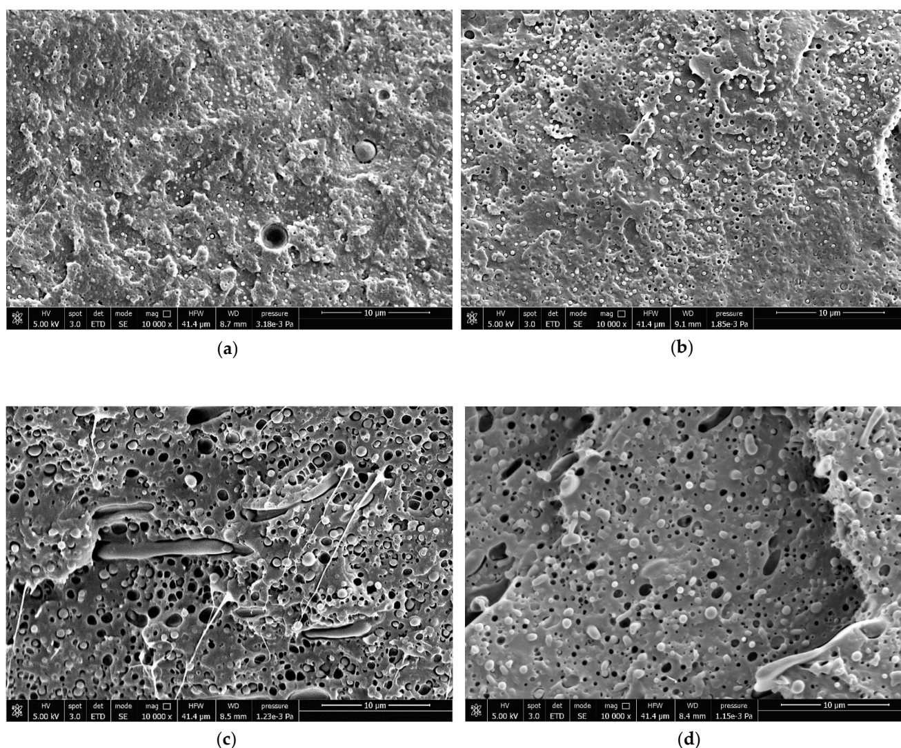
Figure 4. SEM micrographs of: (a) P10, (b) P20, (c) S10, and (d) S20.
