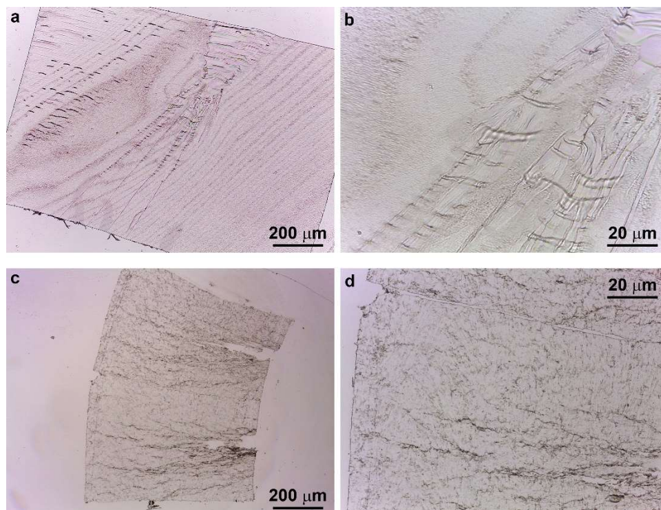
Figure 7. TOM images of the subcritical crack tip section after deformation for the (a,b) P20 and (c,d) S20 samples.
