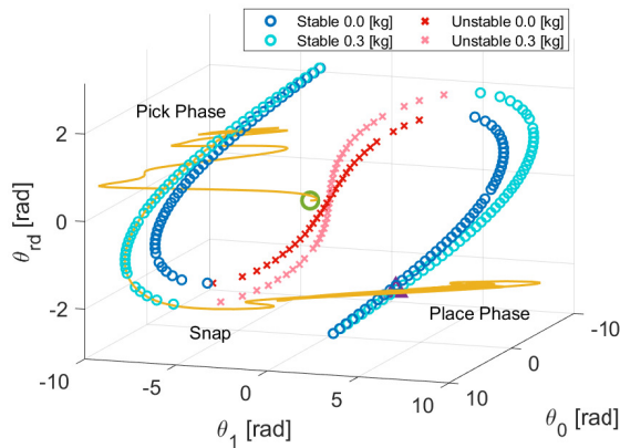
Fig. 7: Evolution of the R-SIP controlled with the pick and place planner, represented in the phase space. In this figure are also shown the equilibria of zero dynamics with \Delta m = 0 and \Delta m = m_{obj} , to visualize the pick and place strategy. The green circle shows the initial state q(0) and the purple triangle the final state q(t_f) .
