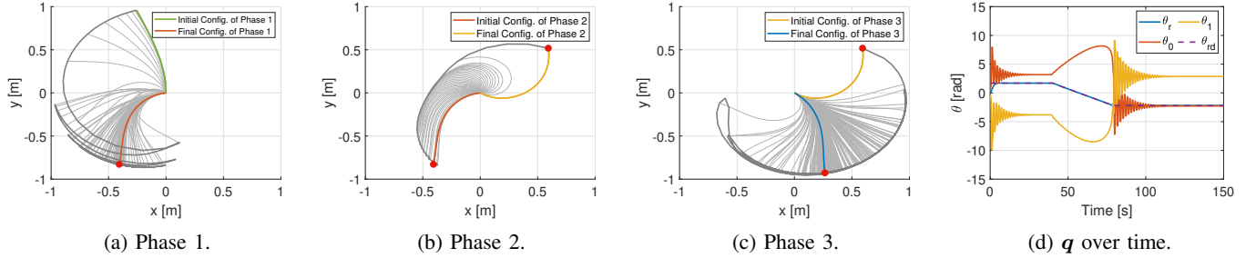
Fig. 6: Pick and place planner applied on R-SIP. (a-c) show snapshots of the catapult trajectory, where the red circle represents the object. In particular, (a) is the "pick" point and (c) the "place" point. In (d), the evolution over the time of q .
