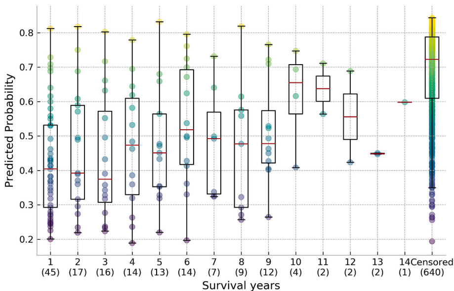
Fig. 2. Calibration analysis for the ensemble model.
