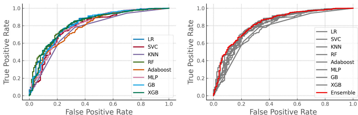
Fig. 1. AUROC Curves for all the ML Models.
