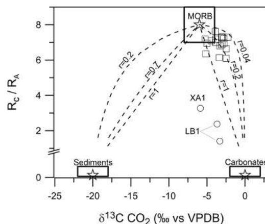
Fig. 11. Correlation diagram R c /R a vs δ 13 C-CO 2 for gas samples collected from natural manifestations in LHGF (modified after Richard et al., 2019). Data from geothermal wells of LHGF are also included. Symbols as in Fig. 10. Labels “r” are the curvature factors of the binary mixed trends, as given by the ratios of the CO 2 /He quotient of the two components considered (i.e., (CO 2 /He) MANTLE /(CO 2 /He) SEDIMENT and (CO 2 /He) MANTLE /(CO 2 /He) CARBONATE ).
