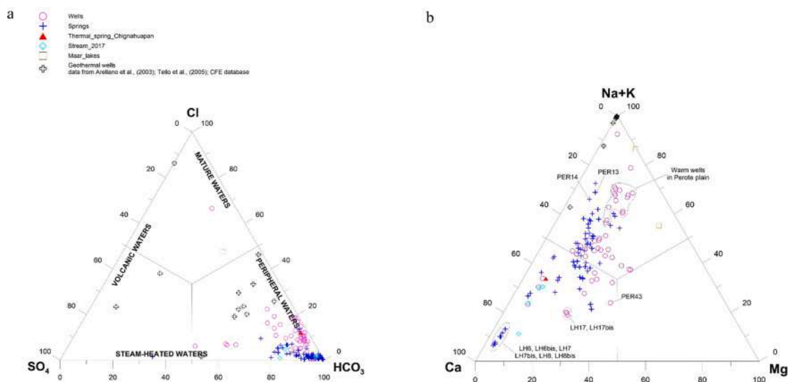
Fig. 3. (a) Classification triangular plot \text{HCO}_3 -Cl- \text{SO}_4 for water samples collected. (b) Classification triangular plot (Na + K)-Ca-Mg for water samples collected. Symbols as in Fig. 3a.
