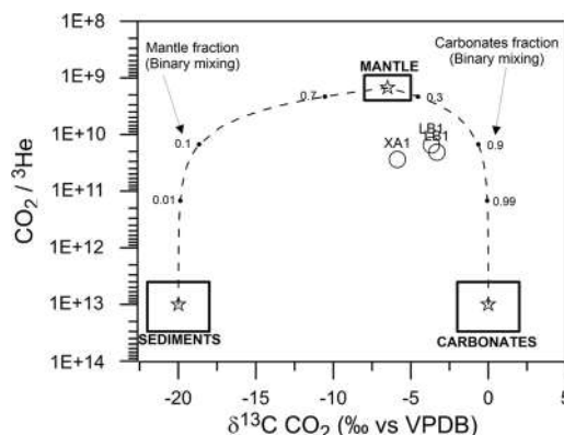
Fig. 12. Correlation diagram CO 2 / 3 He vs δ 13 C-CO 2 for gas samples collected from natural manifestations in LHGF (modified after Sano and Marty, 1995). By applying a three components mass balance approach, we estimate the following relative Mantle (MORB)-Sediments-Carbonates proportions (%): LB1 8.6-15.8-75.6; LB1 8.1-14.2-77.7; XA1 5.6-27.7-66.7.
