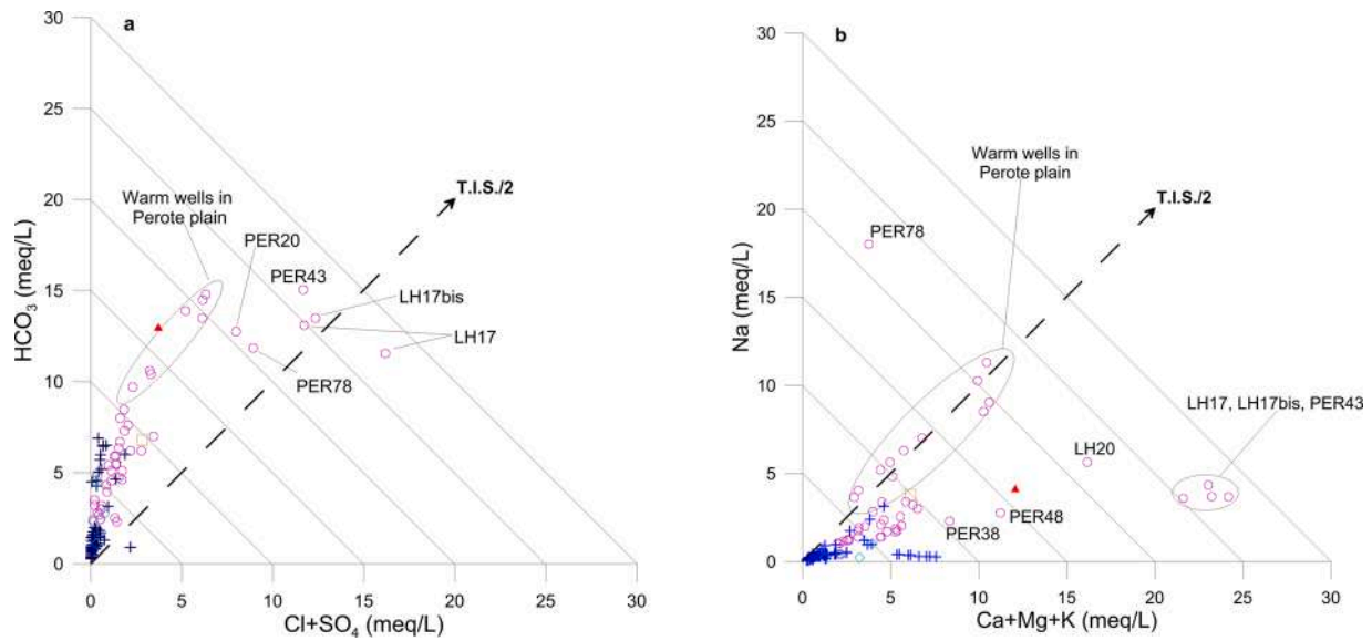
Fig. 4. Correlation plots (a) \text{HCO}_3^- vs. (\text{Cl} + \text{SO}_4) and (b) \text{Na} vs. (\text{Ca} + \text{Mg} + \text{K}) for water samples collected. The iso-salinity lines are also reported. Symbols as in Figure 3a.
