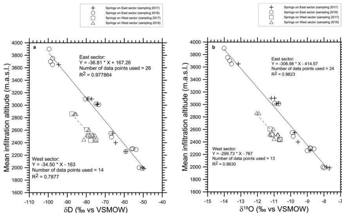
Fig. 7. Correlation of mean infiltration altitude with stable isotopic composition of water samples collected. (a) \delta D ‰ vs mean infiltration altitude; (b) \delta^{18}O ‰ vs mean infiltration altitude.
