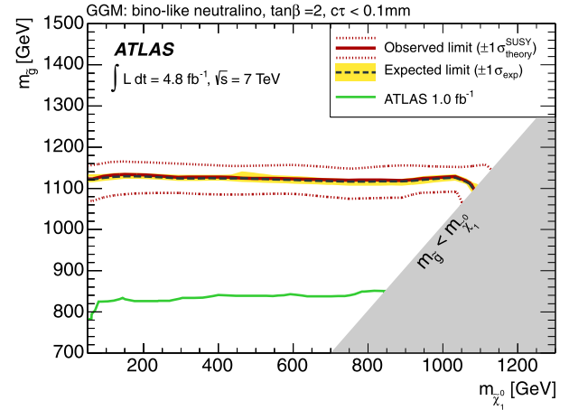
Fig. 6. Expected and observed 95% CL lower limits on the gluino mass as a function of the neutralino mass in the GGM model with a bino-like lightest neutralino NLSP (the grey area indicates the region for which the gluino mass is less than the bino mass, which is not considered here). The other sparticle masses are assumed to be decoupled. Further model parameters are \tan\beta = 2 and c\tau_{\text{NLSP}} < 0.1 mm. The previous ATLAS limit [1] is also shown.
