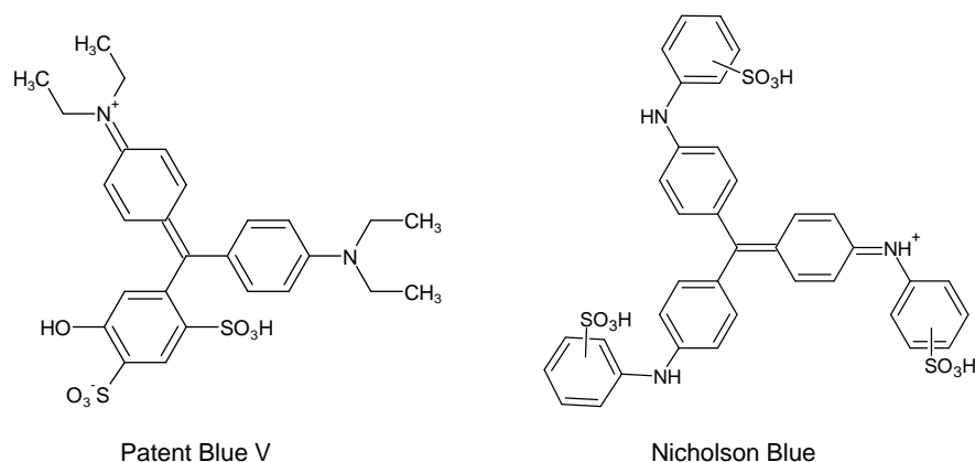
Figure 7. Molecular structures of the sulphonated triarylmethane dyes Patent Blue V (Acid Blue 3, C.I. 42051) and Nicholson Blue (Acid Blue 93, C.I. 42780).
