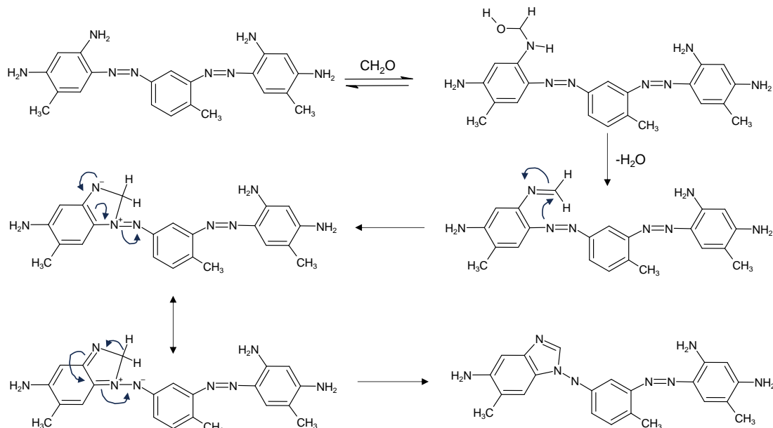
Figure 16. Reaction scheme showing the addition of formaldehyde to Bismark Brown R (C.I. 21020; Basic Brown 4) and leading to the formation of degradation products. The reaction can occur on both sides of the molecule.
