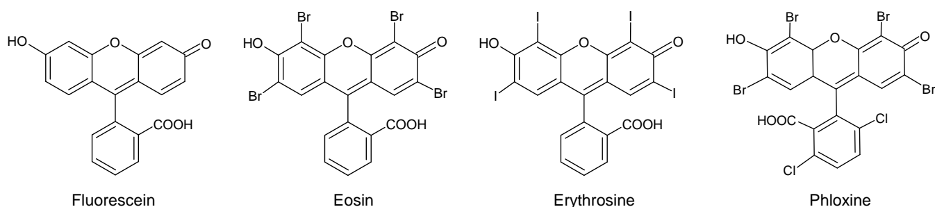
Figure 9. Molecular structures of the xanthene dyes Fluorescein (Acid Yellow 73, C.I. 45350), Eosin (Acid Red 87, C.I. 45380), Erythrosine (Acid Red 51, C.I. 45430) and Phloxine (Acid Red 98, C.I. 45405).
