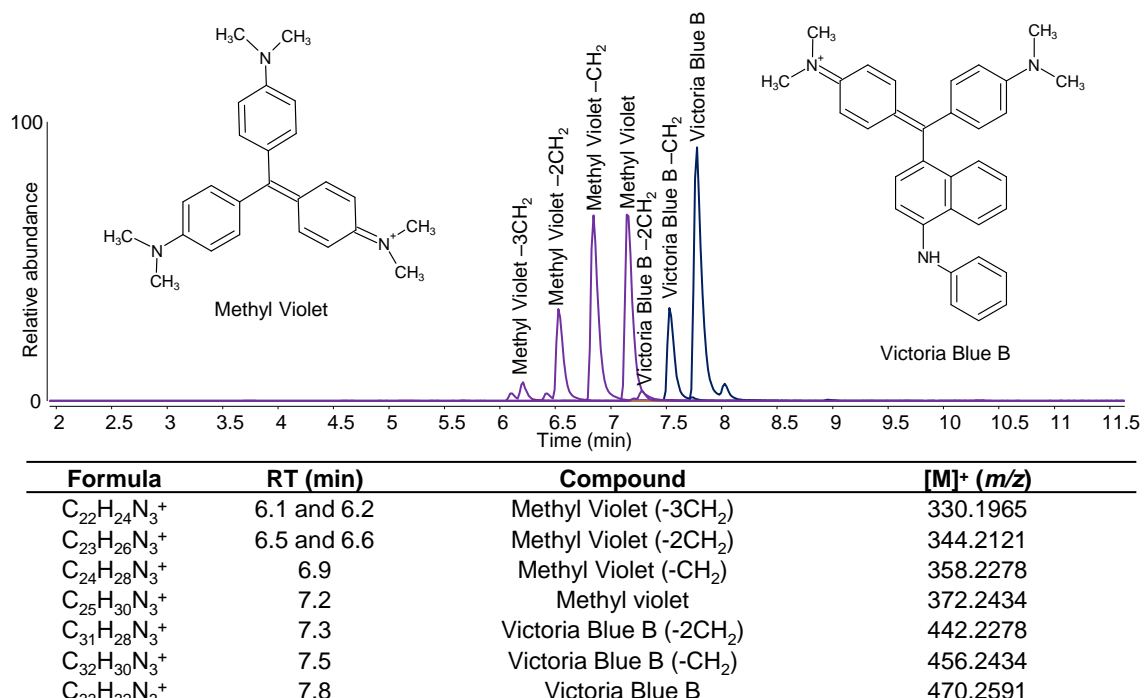
Figure 19. Extracted ion chromatograms obtained by HPLC-ESI-Q-ToF analysis (positive ionisation mode) of a sample taken from textile 2011,6003.46 from the British Museum's collection. The molecular components of Methyl Violet (Basic Violet 1, C.I. 42535) and Victoria Blue B (Basic Blue 26, C.I. 44045) are listed in the legend along with their chemical formula, retention times (RTs) and accurate masses of the corresponding molecular ions [M] + . ©The Trustees of the British Museum. Shared under a Creative Commons Attribution-NonCommercial-ShareAlike 4.0 International (CC BY-NC-SA 4.0) licence.
