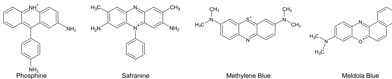
Figure 13. Molecular structures of the dyes Phosphine (Basic Orange 15, C.I. 46045), Safranin (Basic Red 2, C.I. 50240), Methylene Blue (Basic Blue 9, C.I. 52015) and Meldola Blue (Basic Blue 6, C.I. 51175).
