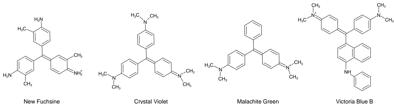
Figure 6. Molecular structures of the triarylmethane dyes New Fuchsine (Basic Violet 2, C.I. 42520), Crystal Violet (Basic Violet 3, C.I. 42555), Malachite Green (Basic Green 4, C.I. 42000) and Victoria Blue B (Basic Blue 26, C.I. 44045).
