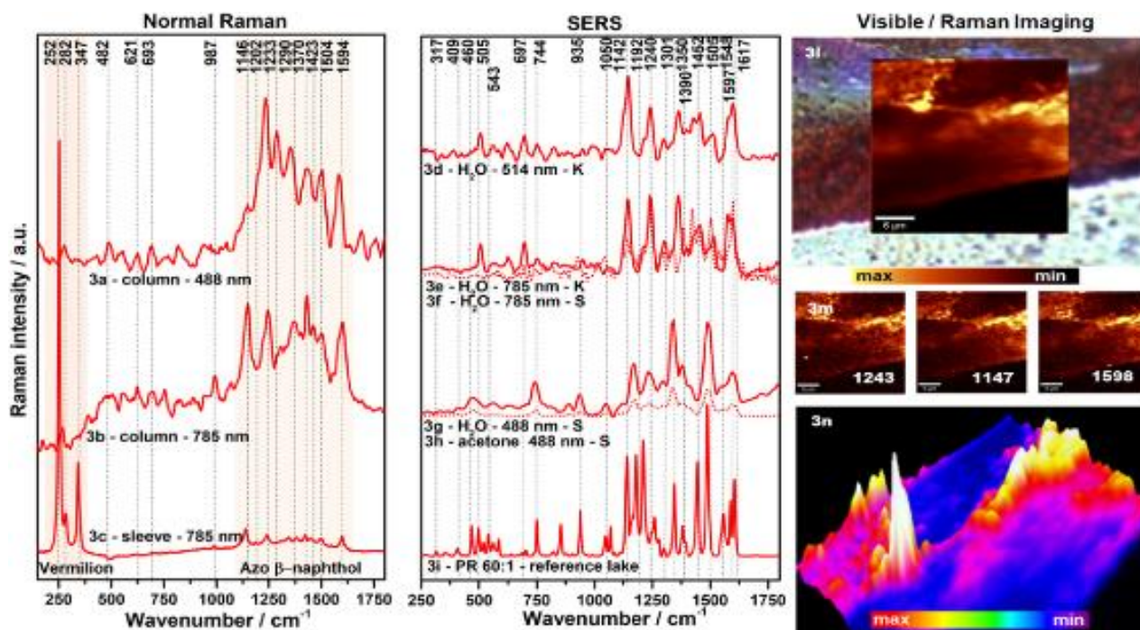
Figure 22. Raman spectra (3a–3c); SERS micro-extracts (3d–3h) with water and acetone transferred to KLARITE® and SOKEN® replicas. Reference spectrum (3i) from SOPRANO Spectral library, PR 60:1, Sunbrite Red, C.I. 16105, naphthalene sulphonic acid (Ba-salt); visible and 3D mapping micro-graphs (3l–3n) on SOKEN® replica, inset overall Raman map (3l), band extraction mode with main bands of an azo \beta -naphthol dye (3m) and 3D SERS mapping (3n) with WITec software ( https://raman.oxinst.com/products/software/WITec-software-suite ). Reprinted from [124] with permissions from Elsevier.
