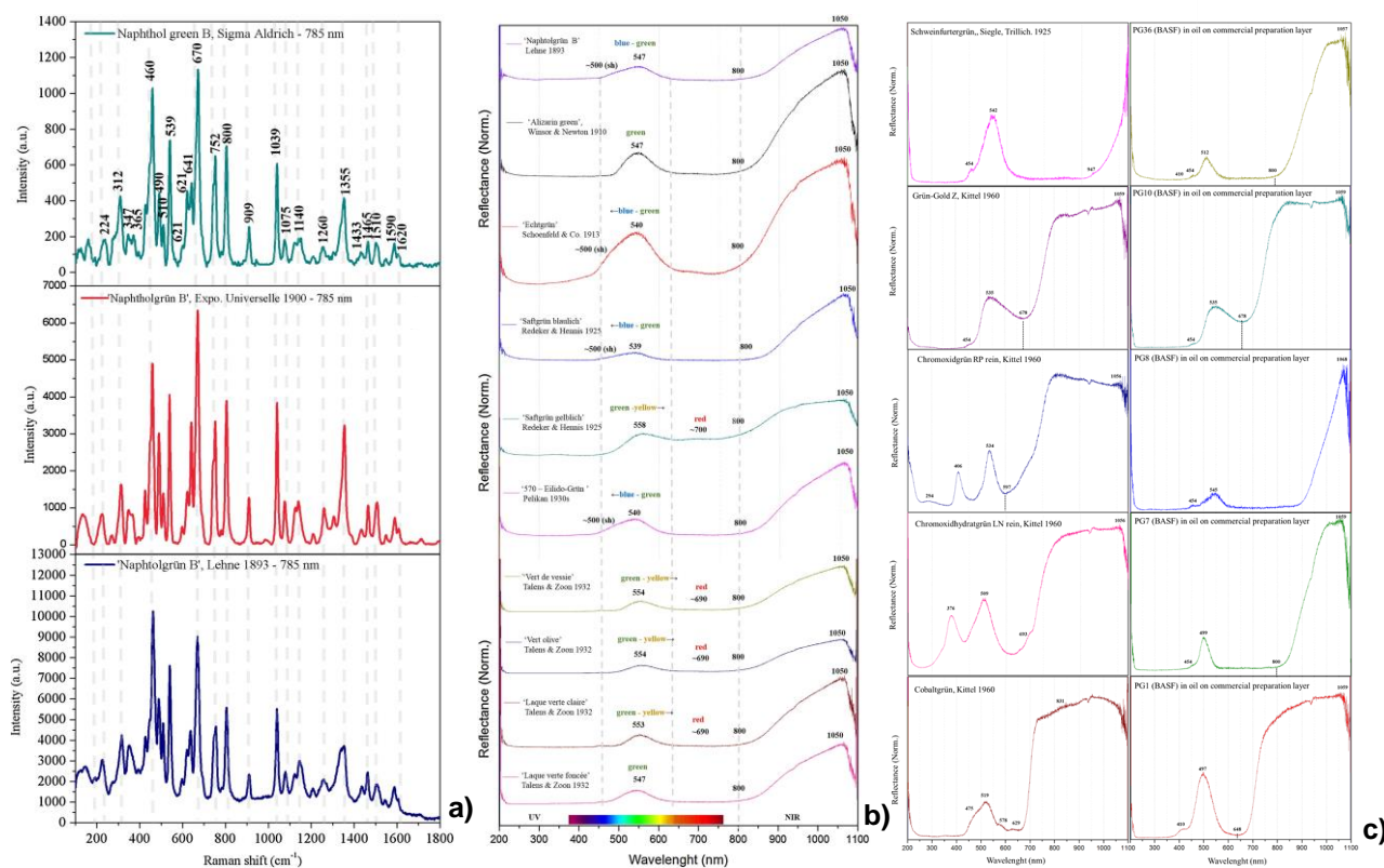
Figure 20. (a) Raman spectra of a modern Naphthol Green B powder (top), a naturally aged powder dye dated 1900 and labelled 'Naphtholgrün B' (middle) and a naturally aged lake pigment on paper
