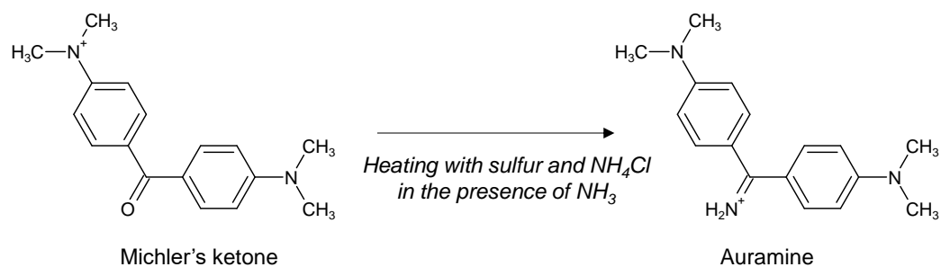
Figure 8. Schematic reaction of the reduction of Michler's ketone to Auramine (Basic Yellow 2, C.I. 41000).
