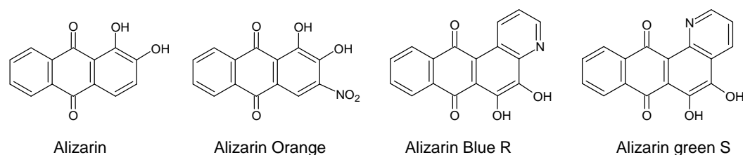
Figure 12. Molecular structures of the anthraquinone dyes Alizarin (Mordant Red 11, C.I. 58000), Alizarin Orange (Mordant Orange 14, C.I. 58015), Alizarin Blue R (C.I. 67410) and Alizarin Green S (C.I. 67405).
