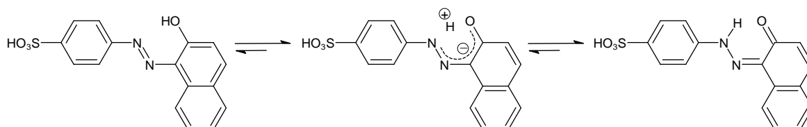
Figure 5. Tautomeric equilibrium between the azoenol form and keto-hydrazone form of orange II (Acid Orange 7, C.I. 15510).
