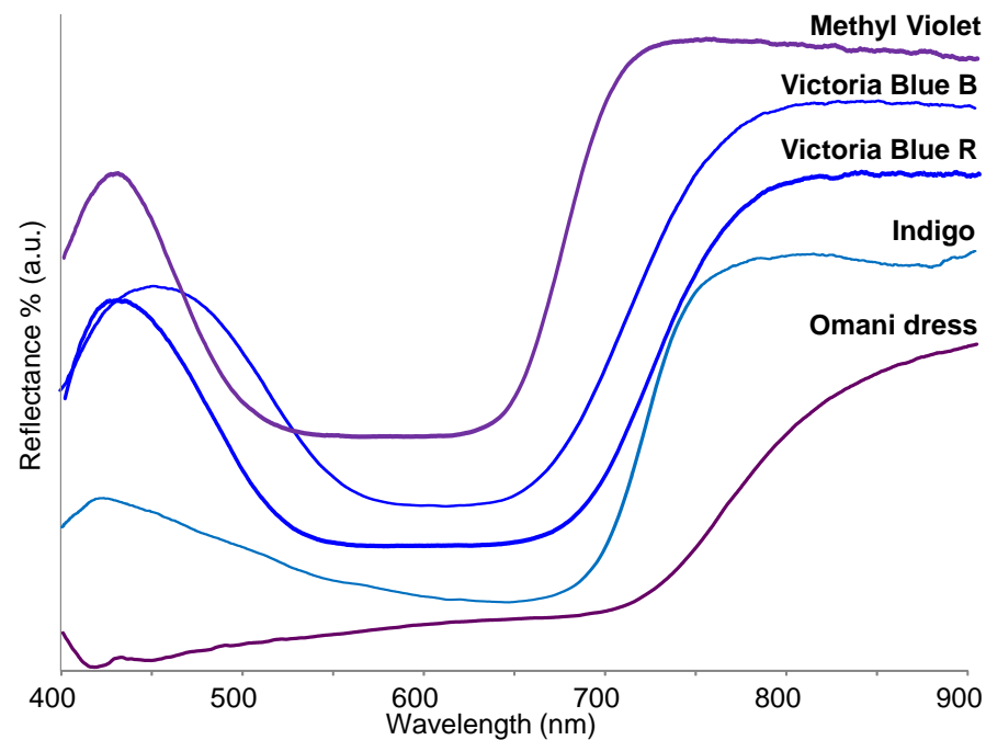
Figure 18. Reflectance spectra acquired by FORS for one of the Omani textiles (representative of the four textiles investigated) and the reference samples of fabrics dyed with indigo, Methyl Violet (Basic Violet 1, C.I. 42535), Victoria Blue B (Basic Blue 26, C.I. 44045) and Victoria Blue R (Basic Blue 11, C.I. 44040). ©The Trustees of the British Museum. Shared under a Creative Commons Attribution-NonCommercial-ShareAlike 4.0 International (CC BY-NC-SA 4.0) licence.
