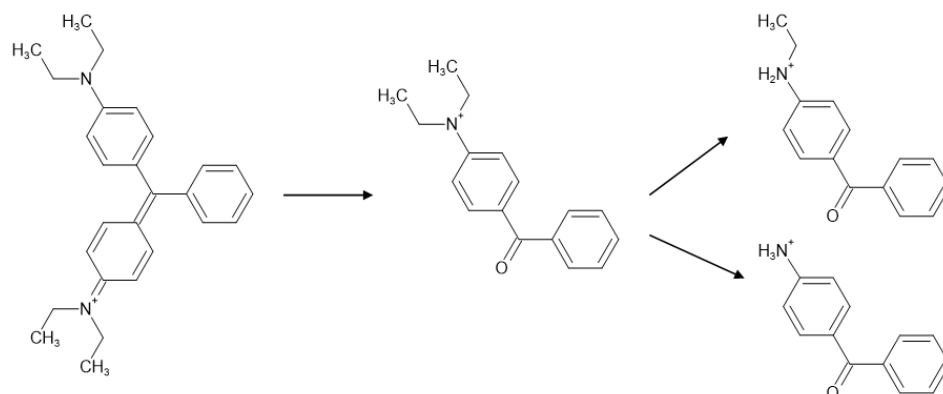
Figure 15. Degradation pathway observed for Brilliant Green (C.I. 42040; Basic Green 1), leading to the formation of benzophenone degradation products.
