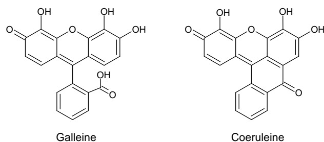
Figure 11. Molecular structures of the xanthene dyes Galleine (Mordant Violet 25, C.I. 45445) and Coeruleine (Mordant Green 22, C.I. 45510).
