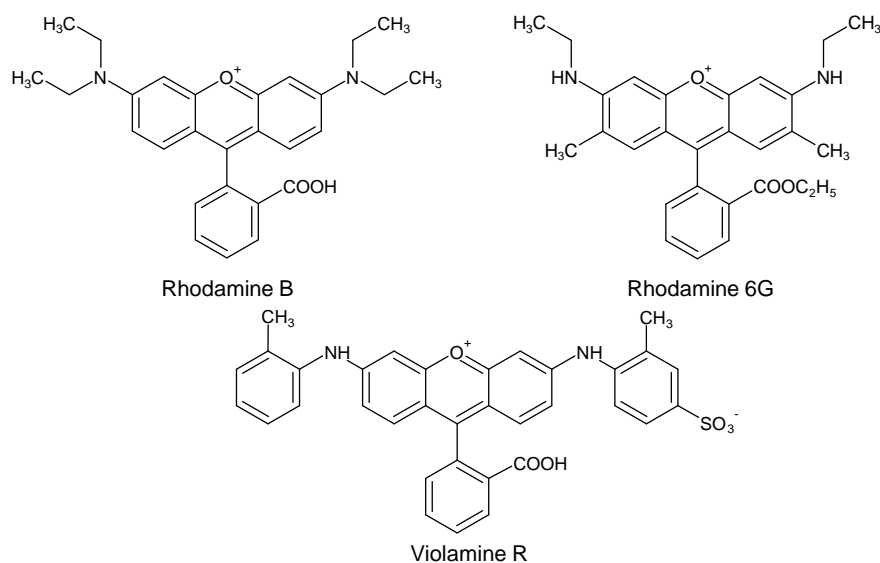
Figure 10. Molecular structures of the xanthene dyes Rhodamine B (Basic Violet 10, C.I. 45170), Rhodamine 6G (Basic Red 1, C.I. 45160) and Violamine R (Acid Violet 9, C.I. 45190).
