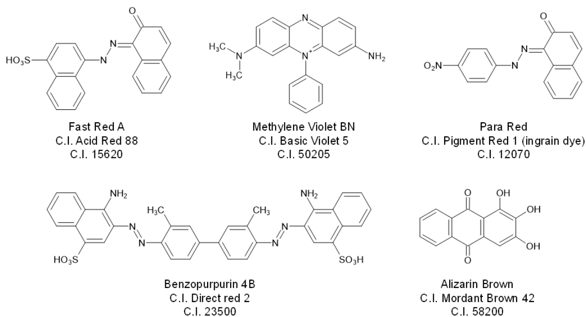
Figure 1. Examples of colourants belonging to different application categories with their respective most common commercial names, C.I. Generic Names and C.I. Constitution Numbers.
