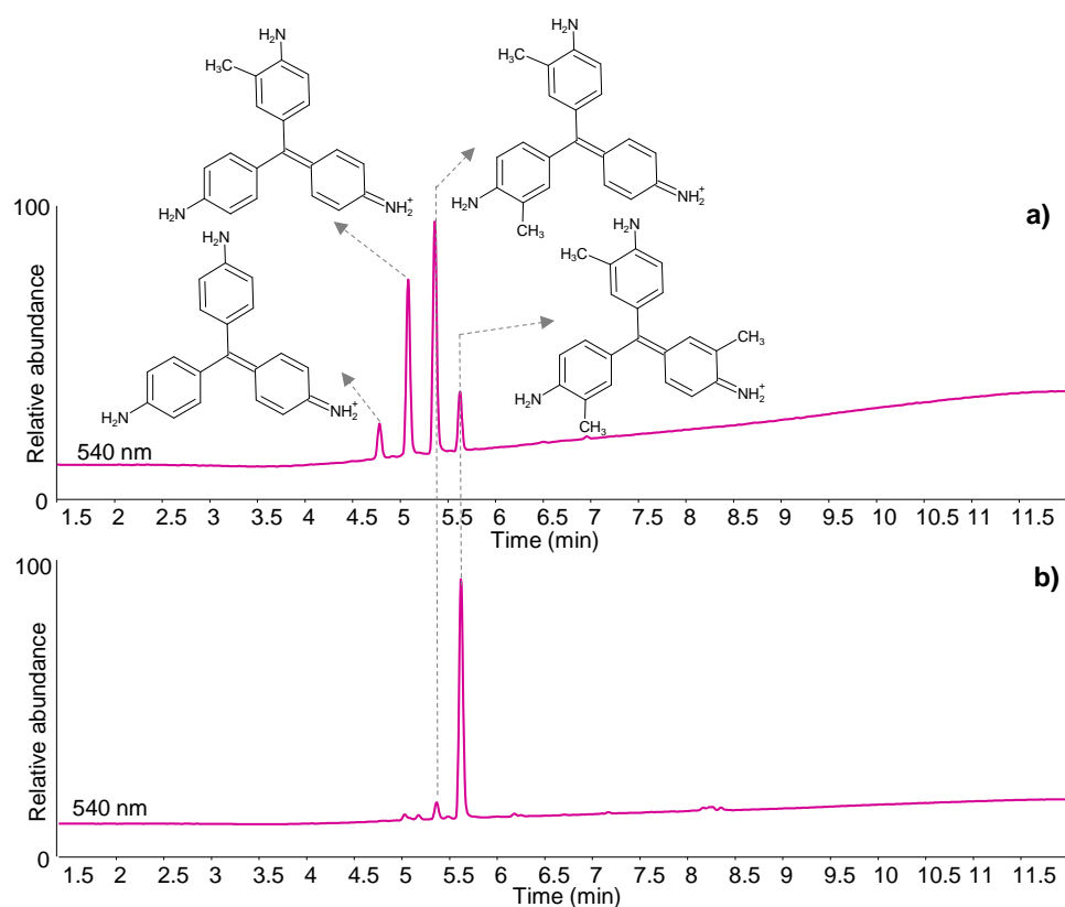
Figure 14. Chromatographic profiles obtained by HPLC-DAD at 540 nm of Fuchsin samples produced with (a) the early synthetic process and (b) the later synthetic process.
