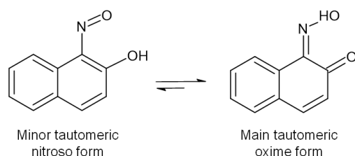
Figure 2. Tautomeric forms of the nitroso dye Mordant Green 4 (C.I. 10005).
