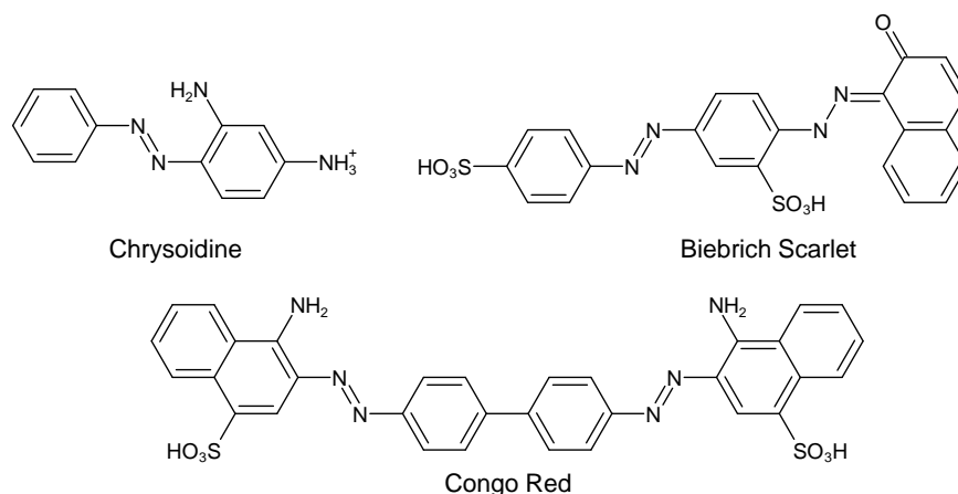
Figure 4. Molecular structures of the monoazo dye Chrysoidine (Basic Orange 2, C.I. 11270) and the disazo dyes Biebrich Scarlet (Acid Red 66, C.I. 26905) and Congo Red (Direct Red 28, C.I. 22120).
