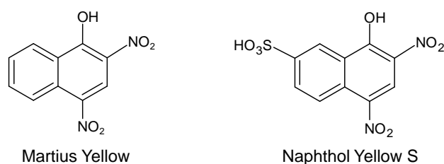
Figure 3. Molecular structures of the nitro dyes Martius Yellow (Acid Yellow 24, C.I. 10315) and Naphthol Yellow S (Acid Yellow 1, C.I. 10316).
