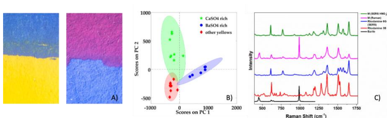
Figure 21. (A) Details of Jazz plates examined under the optical microscope (10× magnification); (B) results of PCA analysis carried out on the p-XRF spectra taken on 23 yellow areas across the 20 MoMA Jazz plates; (C) confocal Raman and SERS spectra of the “magenta” colour (M) alongside reference spectra for Rhodamine 6G (SERS; 612, 775, 1090, 1179, 1310, 1363, 1510, 1574 and 1679 \text{cm}^{-1} ), Rhodamine 3B (confocal Raman; 271, 365, 620, 633, 662, 1082, 1187, 1199, 1362, 1510, 1530, 1599 and 1650 \text{cm}^{-1} ) and barite (sulphate band at 988 \text{cm}^{-1} ). Image rearranged from [33].
