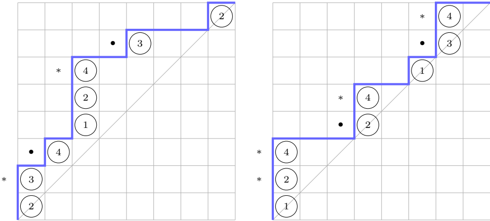
Fig. 1. An element of LD(8)^{*2, \bullet 2} (left) and an element of LD_0(8)^{*4, \bullet 2} (right).
