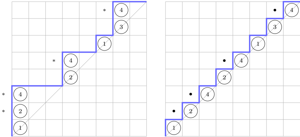
Fig. 2. The images of the ordered set partition 34|1|24|124 (or 43|1|42|421) via the two bijections.
