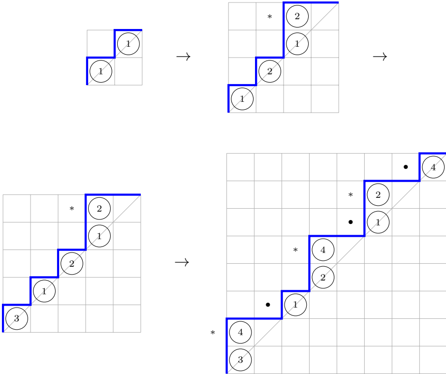
Fig. 4. The steps of Theorem 4.8 for w = 41242|143 .
