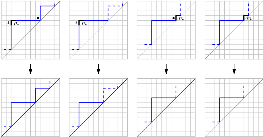
Fig. 3. Four cases for the occurrence of the maximal label m , and how to delete it.
