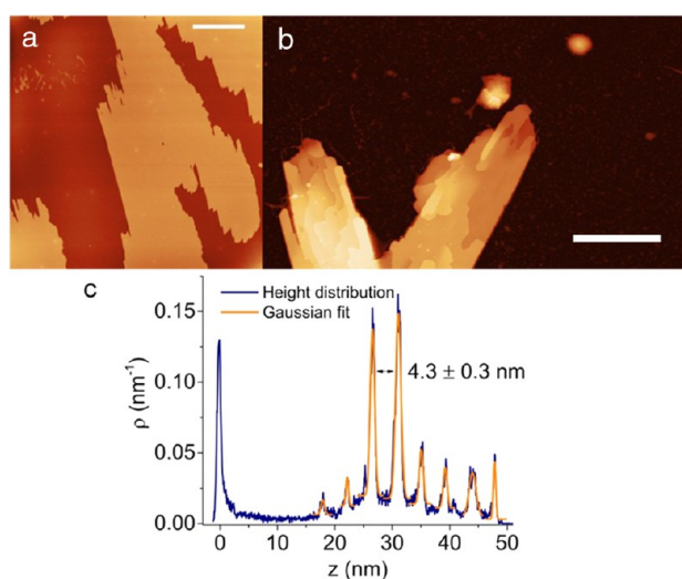
Figure 2. AFM height image of (a) a single-layer flake and (b) a multilayered flake, obtained through electrospray. (c) Height distribution of the multilayered flake as extracted from image (b). Scale bar: (a) 30 \mu\text{m} ; (b) 5 \mu\text{m} . Vertical scales: (a) -10 – 20 nm; (b) -5 – 55 nm.
