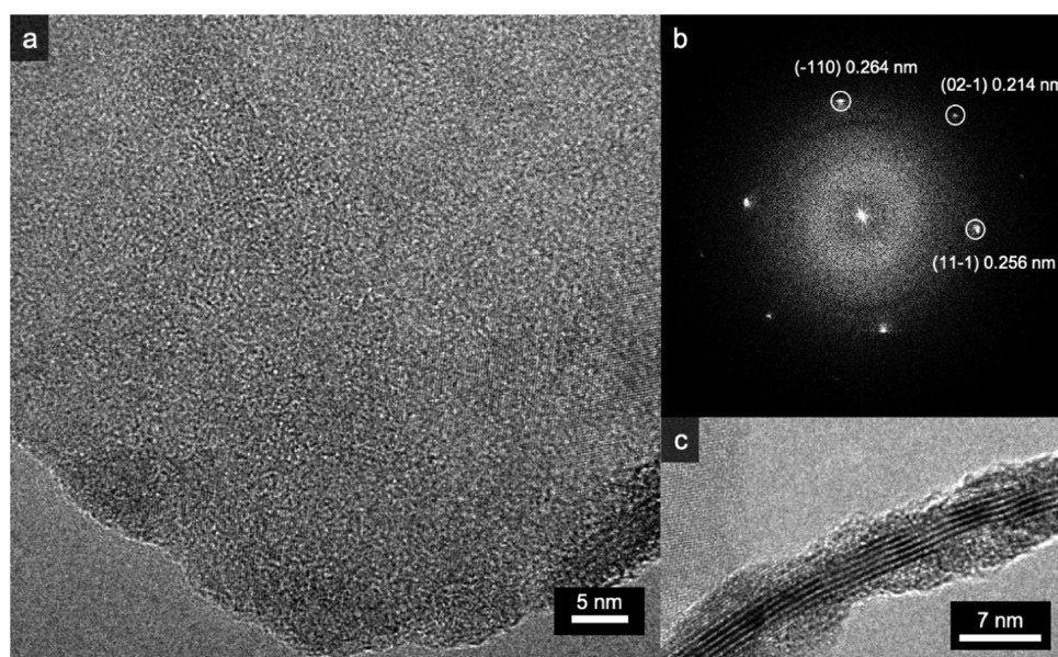
Figure 7. TEM characterization of liquid-phase-exfoliated bP. (a) High-resolution TEM (HRTEM) image of a black phosphorous flake edge. (b) FFT of the image, showing black phosphorous ( \bar{1}10 ), (02\bar{1}) , and (11\bar{1}) reflections. (c) Details of the flake folded edge, showing (002) lattice fringes.
