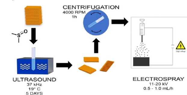
Scheme 1. Schematic Illustration of the Deposition of 2D \text{PO}_x Flakes Using the Electrospaying Technique, Starting from Liquid-Phase-Exfoliated bP
