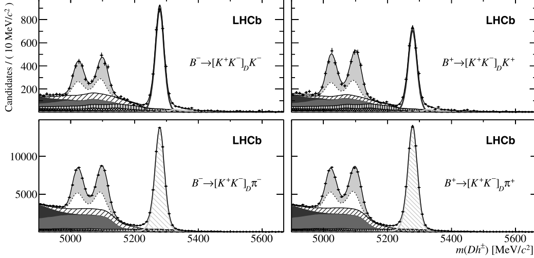
Fig. 2. Invariant mass distributions of selected B^\pm \rightarrow [K^+K^-]_D h^\pm candidates, separated by charge. See Fig. 1 for details of each component.
