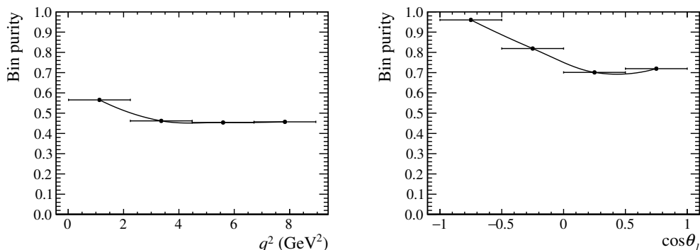
Figure 1. Purity as a function of q^2 and \cos \theta_l , defined as the fraction of candidates which belong in a particular kinematic bin. The purity for \cos \theta_l is better than for q^2 due to the better resolution.
