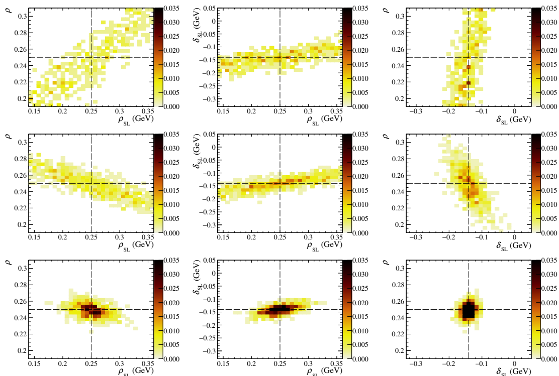
Figure 6. Two-dimensional distributions of the Isgur-Wise parameters as fitted from an ensemble of pseudoexperiments. Both q^2 and \cos\theta_l are fitted simultaneously. Only simulated \Lambda_c(2595)^+ and \Lambda_c(2625)^+ data are used for the pseudoexperiments shown in the first and second row, respectively. Both states are fitted in the pseudoexperiments shown in the third row. The dashed lines indicate the numerical values of the parameters used to generate the pseudoexperiments.
