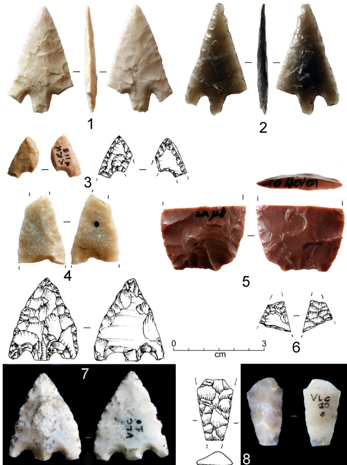
Figure 7. Triangular, barbed-and-tanged arrowheads with flat invasive or covering bifacial retouch from Kirkuri (Krk-28, n. 1), Sam-8 (n. 2), Mirmindia Pass (VLC-1, n. 7); hollow-based arrowhead from Kirkuri (Krk-118, n. 3); fragments of arrowheads from Kirkuri (Krk-14, n. 4; Krk-92, n. 6) and the Mirmindia Pass (VLC-10, n. 8); proximal fragment of dagger obtained by flat, covering bifacial retouch from Sam-8 (n. 5) (photographs by E. Starnini; drawings by P. Biagi; inking by G. Almerigogna).
