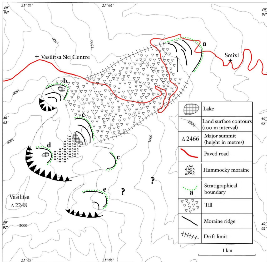
Figure 13. Geomorphological map of the Mount Vasilitsa area. The stratigraphical units marked a–d represent the Vasilitsa Formation: (a) Smixi Member, (b) North Vasilitsa Member, (c) Central Vasilitsa Member, (d) Vasilitsa Summit Member. The stratigraphic unit marked (e) represents the East Vasilitsa Member, the sole unit of the East Vasilitsa Formation (drawing by P. Hughes).
