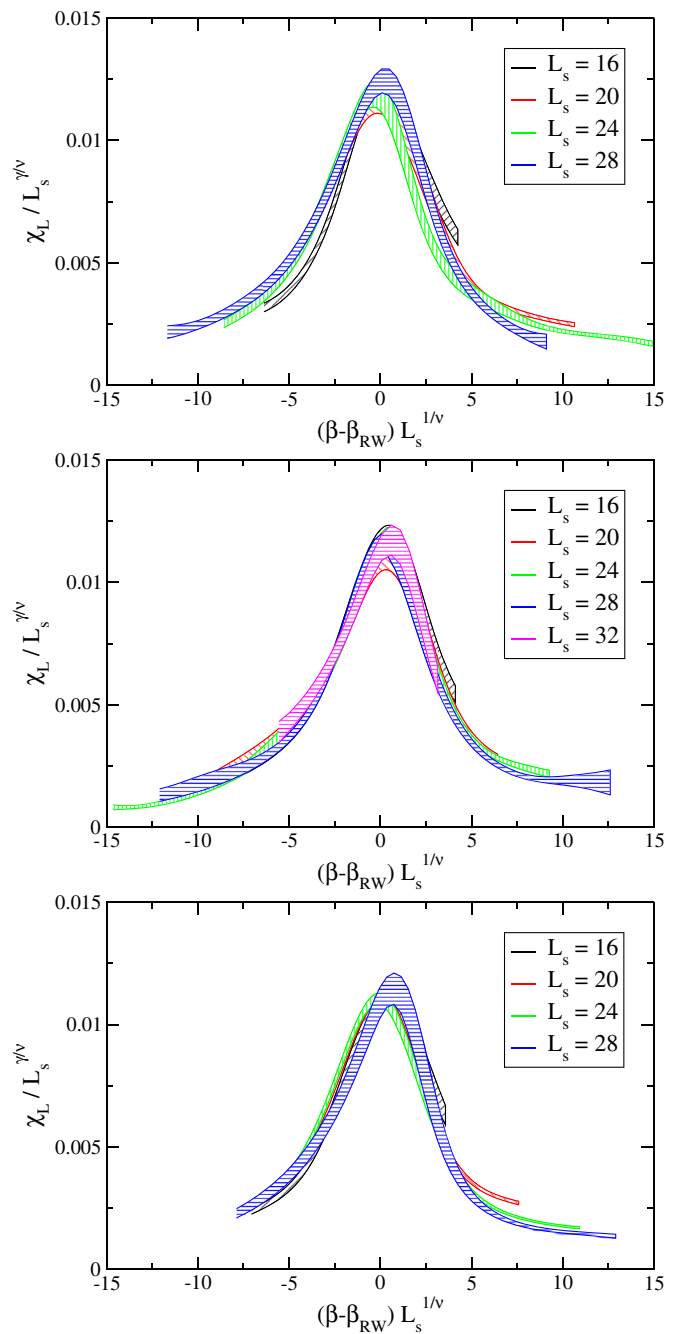
FIG. 5. Finite size scaling for the susceptibility of the Polyakov loop according to tricritical indices. From top to bottom: am_l = 0.003 , am_l = 0.0015 and am_l = 0.00075 .
