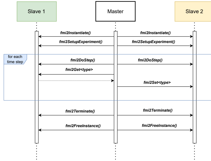
Fig. 2. Example of Simulation FMI-compliant.
