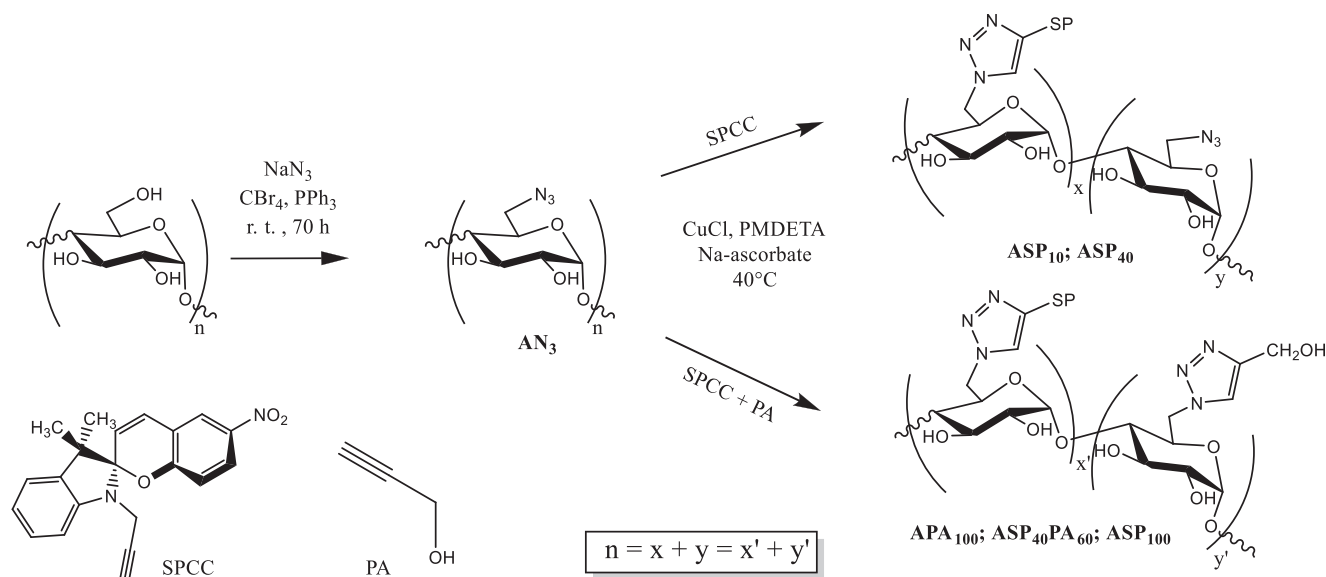
Scheme 2. Structures and synthesis of spirocyclic amylose derivatives. [37]
