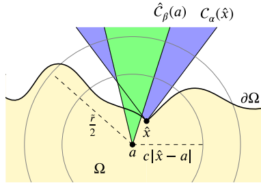
Fig. 1. Sketch of \Omega and the cones C_\alpha(\hat{x}) and \hat{C}_\beta(a)
