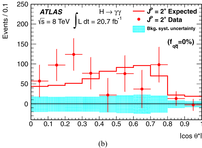
Fig. 2. Distributions of background-subtracted data in the signal region as a function of |\cos\theta^*| . The expected distributions for (a) spin-0 and (b) spin-2 signals produced by gluon fusion, normalised to the fitted number of signal events, are overlaid as solid lines. The cyan/grey bands around the horizontal lines at zero show the systematic uncertainties on the background modelling before the fits, which include the statistical uncertainties on the data sidebands.
