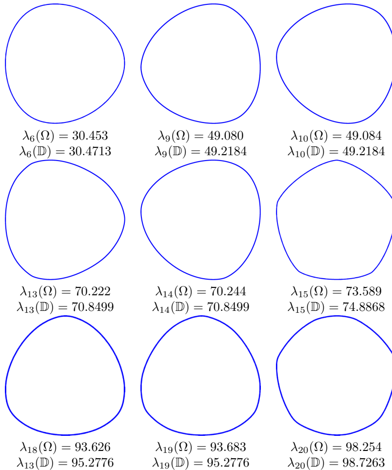
FIG. 1. Noncircular shapes of constant width 2 which are candidates to be the minimizers of \lambda_h for h = 6, 9, 10, 13, 14, 15, 18, 20 .
