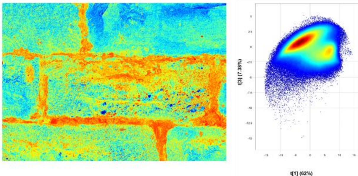
Figure 3_ Detail of the inner wall of Carcassonne acquired with the NEO HySpex-320m-e camera system. On the right the PCA model shows all the pixel values distributed in the multivariate space, on the left the same pixels in the image are colored according to the intensity value (t1). It is easy to spot the compositional difference between the building materials, in this case sandstone, and the architectural mortar. Moreover the hyperspectral image highlights some inclusion in the sandstone (blue dots in the center on the image) that can be used to establish the quarry of origin.
