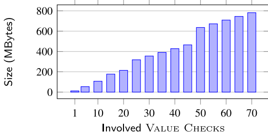
(a) Proving key size in MB.
