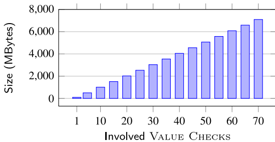
(b) Circuit size in MB.
