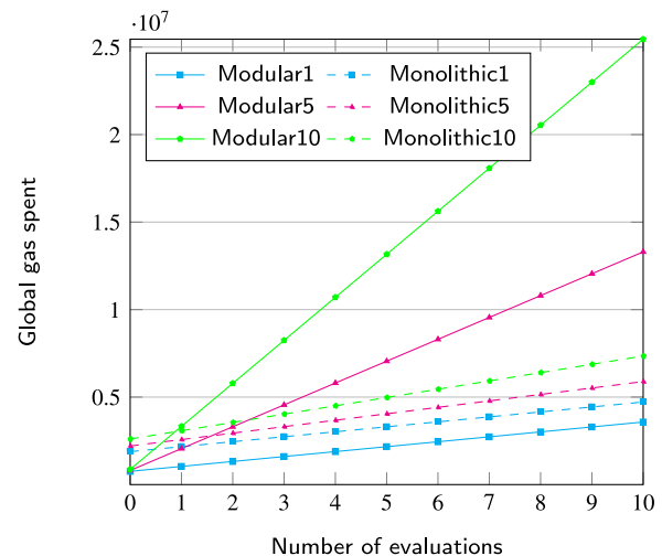
Fig. 12. Global cost of a SMARTPOLICY life cycle, including initial deployment cost and subsequent evaluation costs, for an increasing number of policy evaluations. For the Monolithic approach the initial deployment of the needed zkVERIFIER is counted as well. We consider both Modular and Monolithic models for 1, 5, and 10 VALUE CHECKS.
