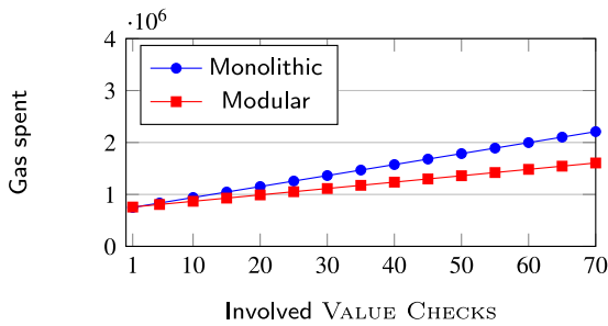
(a) SMARTPOLICY deployment cost.
