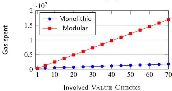
(b) SMARTPOLICY evaluation cost.
