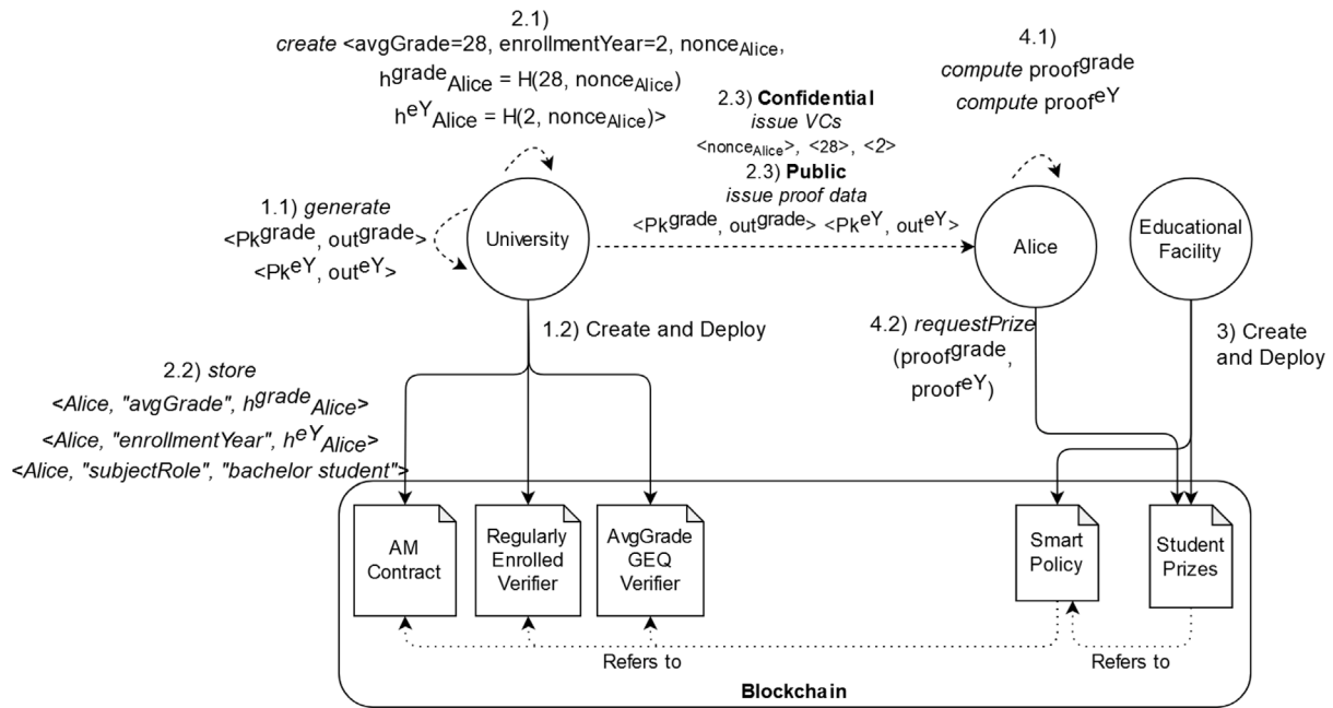
Fig. 7. Workflow overview.
