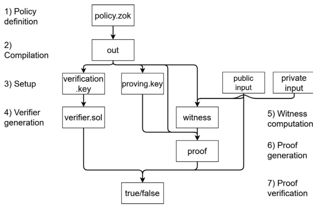
Fig. 3. ZoKrates workflow.
