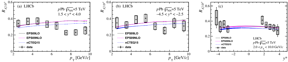
Fig. 3. The cross-section ratio R_{\Lambda_c^+ / D^0} between \Lambda_c^+ baryons and D^0 mesons as a function of p_T in (a) the forward rapidity region, (b) the backward rapidity region, and (c) as a function of y^* integrated over 2 < p_T < 10 GeV/c. The error bars represent the sum in quadrature of the statistical and the systematic uncertainties. The coloured curves represent HELAC-Onia calculations with nPDFs EPS09LO/NLO and nCTEQ15.
