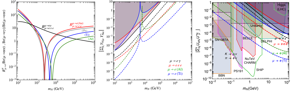
Figure 4.14: Left panel: Br(\mu \rightarrow e\gamma)/Br(\mu \rightarrow eee) and R_{\mu \rightarrow eee}^{\mu} = R_{\mu \rightarrow eee}^N / Br(\mu \rightarrow eee) as a function of the right-handed neutrino mass scale m_N , for \mu \rightarrow e conversion in various nuclei, from Ref. [392, 612]. Middle panel: from Ref. [392], present bounds and future sensitivity on |\sum_i^k Y_{\Sigma_{i\mu}} Y_{\Sigma_{ie}}^*| for scenarios characterized by one right-handed neutrino mass scale. The solid lines are obtained from present experimental upper bounds: from R_{\mu \rightarrow e}^{Ti} < 4.3 \cdot 10^{-12} [613] and Br(\mu \rightarrow e\gamma) < 5.7 \cdot 10^{-13} [614], Br(\mu \rightarrow eee) < 10^{-12} [615]. The dashed lines are obtained from the expected experimental sensitivities: from R_{\mu \rightarrow e}^{Ti} \lesssim 10^{-18} [605, 616], R_{\mu \rightarrow e}^{Al} \lesssim 10^{-16} [605]-[606] and Br(\mu \rightarrow e\gamma) < 10^{-14} [607], Br(\mu \rightarrow eee) < 10^{-16} [604]. Right panel: from [392], |\sum_i U_{eN_i} U_{\mu N_i}^*| (with U_{jN_i} \equiv Y_{N_{ji}}^\dagger v / M_{N_i} the mixing angles with v = 174 GeV) versus mass sensitivity regions for present (continuous curves) and future (dashed curves) e - \mu flavour experiments. Black, red, green and blue curves result from Br(\mu \rightarrow e\gamma) , Br(\mu \rightarrow eee) , R_{\mu \rightarrow e}^{Ti} and R_{\mu \rightarrow e}^{Al} , respectively. The regions already excluded by non-unitarity limits, \pi and K peak searches, \pi , K , D , Z decay searches, BBN, SN1987A and LHC collider searches (dotted lines) are also indicated. Shaded areas signal the regions already excluded experimentally. The right panel shows the nice future complementarity between CLFV experiments and SHiP.
