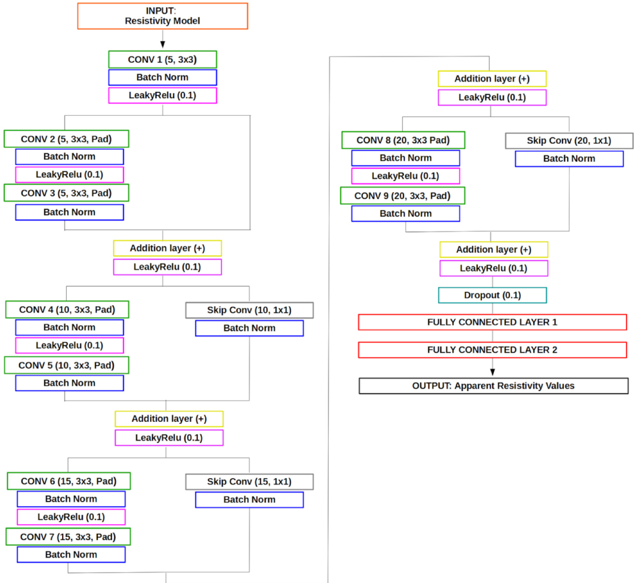
Figure 2 Representation of the employed ResNet architecture annotated with key parameters. For example, in the second convolutional layer ‘CONV 2’ the term within bracket (5, 3 × 3, Pad) indicates that we employ 5 convolutional filters with size 3 × 3 and that zero-padding is applied. The only difference in the synthetic and field data applications concerns the dimension of input and output response. See the text for details.
