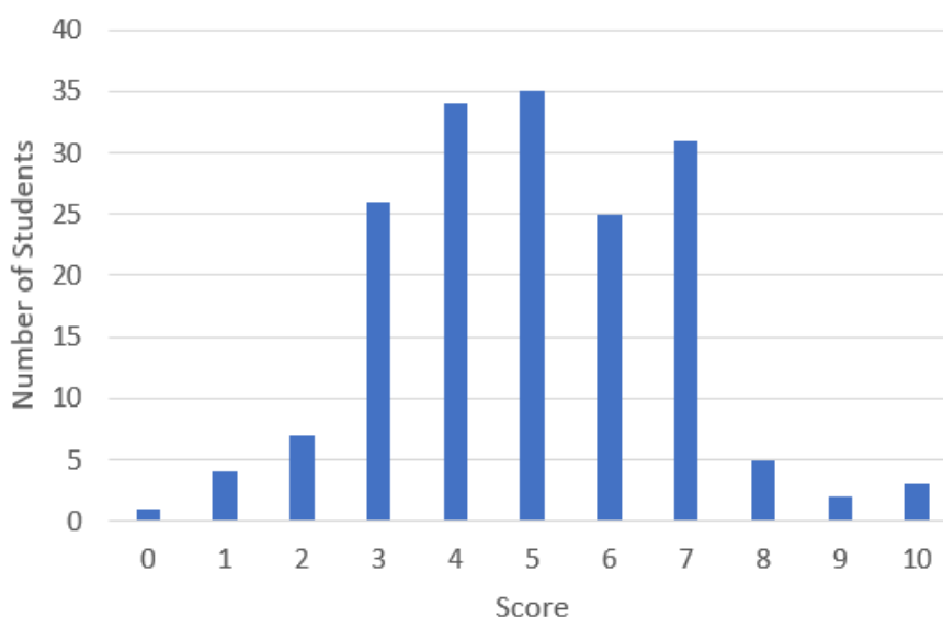
Figure 7. Distribution of students' scores in the quantum technologies inventory (QTI). See text for details.
