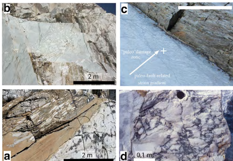
Figure 4. (a) Paleokarst and related marble breccias (Morlungho quarry); (b) Fault-related neptunian-dyke, Pianza quarry; (c) Veined marble interpreted as paleo-fault damage zone and related paleo-fault breccias; (d) marble variety of “Paonazzo” a breccia-variety characterized by Fe- and Mn-rich mineralized matrix.
