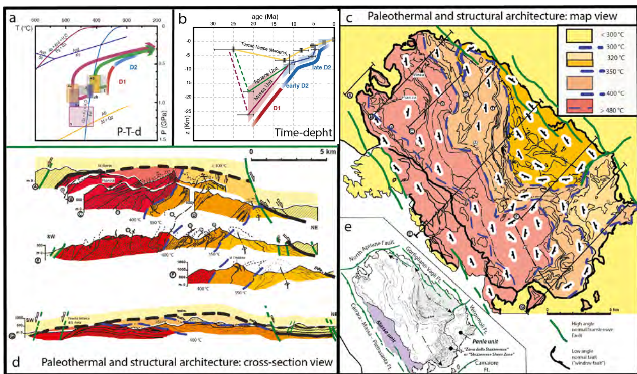
Figure 7. (a) P-T estimates and paths for the Apuane and Massa units. Data used for boxes 1-4 are derived from quantitative classical thermo-barometry as well as pseudosections (Franceschelli et al. , 1986; Jolivet et al. , 1998; Molli et al. , 2000; Papeschi et al. , 2023). Data used to define box 4 also include temperatures based on Raman spectroscopy on carbonaceous material (RSCM) (Molli et al. , 2018). Red and blue lines outline the relative timing of deformation for D1 and D2 with changing metamorphic conditions. For more details see Di Vincenzo et al. , 2022; (b) Time-depth paths of the Massa and Apuane units and of the overlying Tuscan nappe (Macigno) modified after Fellin et al. , 2007 including data in Di Vincenzo et al. , 2022; (c) Paleothermal architecture of the Alpi Apuane metamorphic core complex in map view; (d) paleothermal architecture at window-scale in cross-sections view; (e) overall structural architecture of the Alpi Apuane metamorphic core. Also indicated and named the main boundary faults around the metamorphic core.
