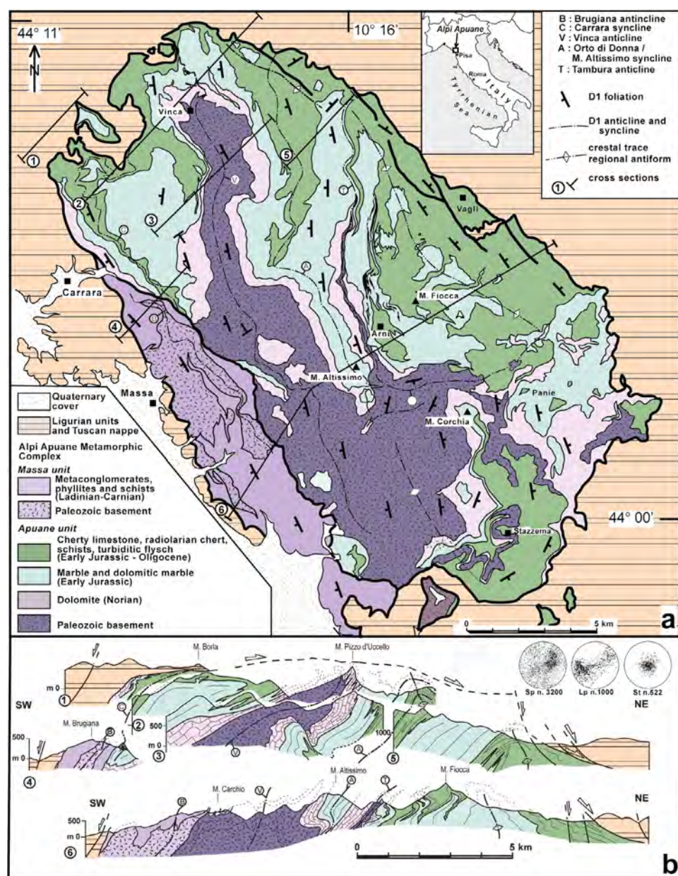
Figure 2. (a) Simplified geological-structural map and (b) composite cross sections across the Alpi Apuane. The dashed lines show the axial traces of the major D1 and D2 folds. Equal area lower hemisphere stereograms show the poles to the main foliation (Sp), stretching lineation (Lp), and the poles of late crenulation cleavage (St).
