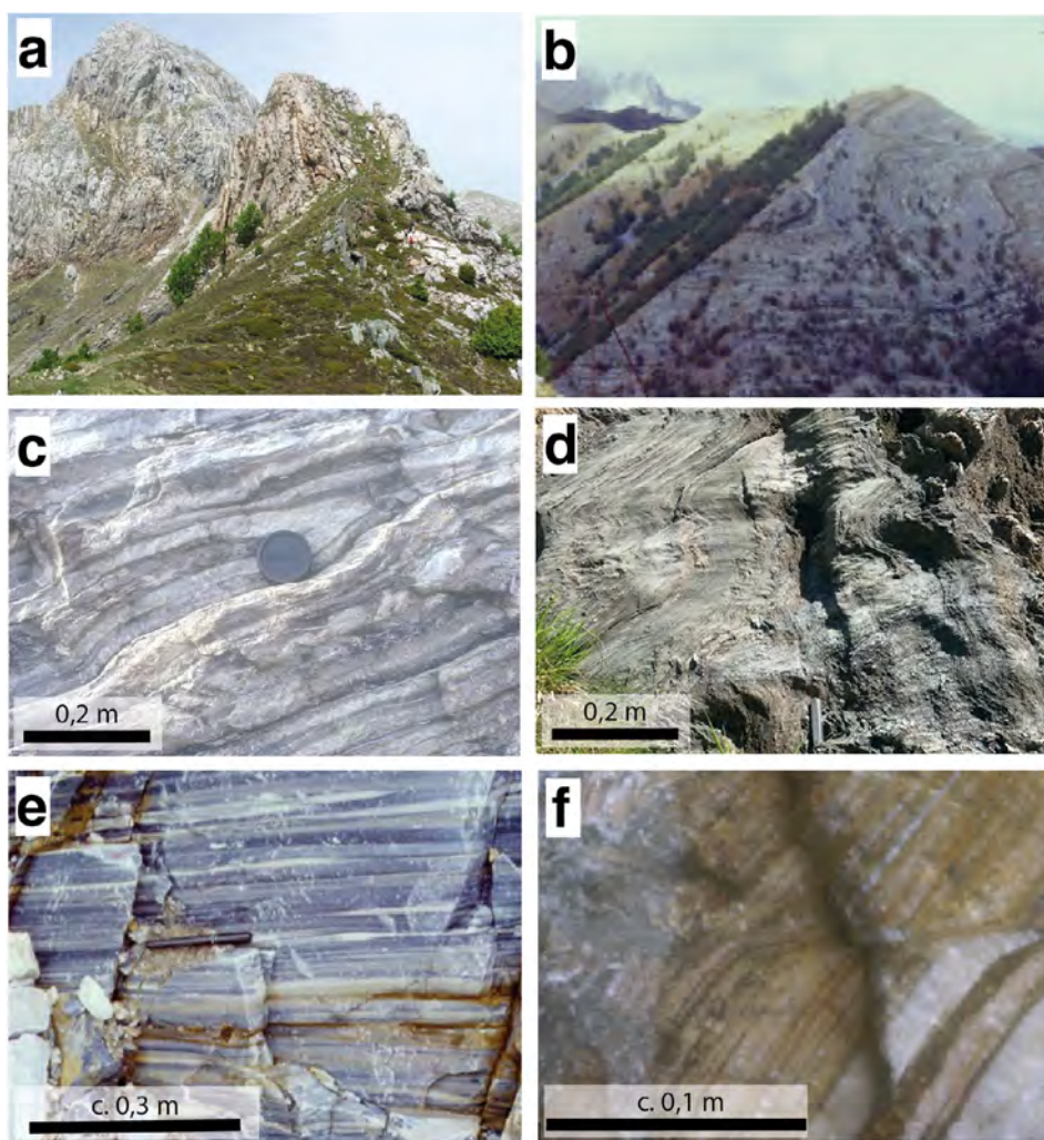
Figure 5. (a) Panoramic view, looking north, from Foce di Giovo, northern Alpi Apuane. Two plurihctometer-scale folds in the hinge zone of the km-scale D1 Vinca-Forno Anticline are visible. D1 folds are refolded by D2 folds with a horizontal fold axial plane. Dark green Paleozoic schists making cusps within the metadolstones of the Grezzoni Fm.; (b) D2 west-vergent cascade-folds affecting the Grezzoni metadolstone in the normal limb of Vinca-Forno Anticline (Cima D'Uomo, Colonnata). (c) D1 meter-scale isoclinal fold and related axial planar foliation, overprint by D2 cleavage (Cherty metalimestone of Mt.Uccelliera); (d) meter-scale open D2 folds associated with a sub-horizontal crenulation cleavage (Scisti Sericitici Fm., Arni valley, eastern Alpi Apuane); (e) calc-mylonites derived from cherty metalimestones within a Late D1 shear zone. Colonnata valley, Carrara western Alpi Apuane; (f) decimeter-scale D2 shear zone in impure marble, Forno valley inland of Massa (for detailed microstructural description and fabric-types evolution see Oesterling et al. , 2007).
