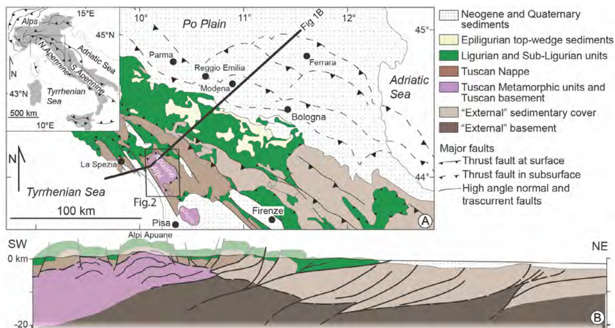
Figure 1. Tectonic map of the Northern Apennines, with crustal scale (b) cross section (modified after Molli, 2008).
