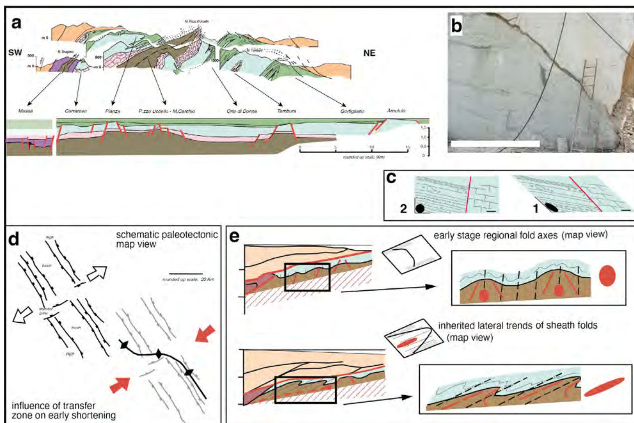
Figure 6. (a) General cross-section of the Alpi Apuane showing the regional-scale structures and their relationships with the original paleogeography modified after Carmignani et al. (1987) and Carmignani & Kligfield (1990); (b) White marble thrust above stratified impure pale greenish marble, scale bar ca. 2.5 m. Figured are details of thrust plane and meter-scale east-vergent folds developed in the footwall of the thrust; (c): c1 schematic line drawing showing the present-day geometry and lithology of the outcrop. Based on the local finite strain data and a simple shear strain path the original geometry can be reconstructed (c2); (d) schematic paleotectonic map view showing the possible segmentation of the former basin and transfer zones as well as their influence during the early “inversion”-related shortening; (e) regional tectonic frame with close up of vertical profiles and map views of early normal fault-controlled buckling during underthrusting of the external Tuscan Domain (Alpi Apuane zone) and later modification by shearing to produce the recumbent Alpi Apuane D1-fold structures.
