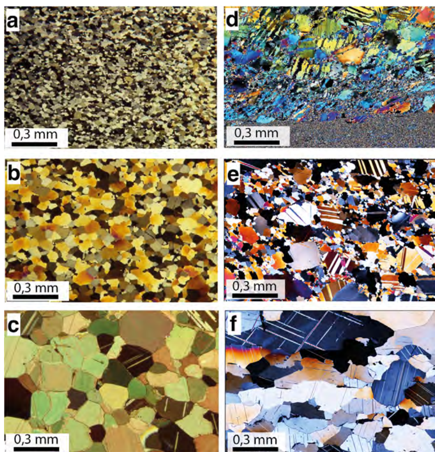
Figure 8. Marbles microstructures a,b,c: Statically recrystallized or annealed microstructure (Type A). Sample (a) from the Pania unit, southern Alpi Apuane, structural domain characterized by RSCM temperature of 320 °C; sample (b) from the eastern Alpi Apuane, domain characterized by RSCM of 360 °C; sample (c) from the western Alpi Apuane, domain characterized RSCM of 480 °C. Dynamic recrystallized microstructures (Type B): (d) sample coming from a millimeter-scale rim tapering the main slip surface of an High Angle Normal Fault (Late D2 history); (e) Type B2-microstructure related to D2 shear zones, localized deformation during the switch from crustal-scale contraction to crustal-scale extension (early D2); (f) Type B1-microstructure related to a Late D1 shear zone, localized deformation during the antiformal stacking.
