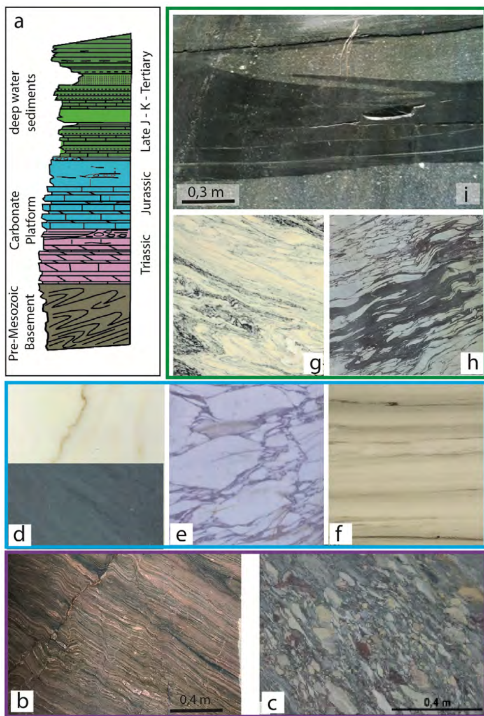
Figure 3. (a) General stratigraphic sequence of the Apuane unit with some characteristic rock-types quarried as ornamental stones. In particular: b) Carnian impure marble part of the Vinca Fm. quarried as “Rosso Rubino”; (c) Breccia di Seravezza, Late Rhaetian scree-breccia also known with the historical name of “Breccia Medicea”; (d) “Carrara marble”: variety “Statuario” (upper part) and “Bardiglio” (grey marble) in the lowermost part; (e) marble breccia variety of “Arabescato”; (f) impure marble quarried with the name of “Zembrino”. This rock types occupy the stratigraphic position of the “Rosso Ammonitico” between Massiccio and Calcare Selcifero in the un-metamorphic Tuscan succession; (g) impure marble “Cipollino”; (h) Breccia Rossa, characteristic rock-units of the eastern Alpi Apuane, typical of “condensed” stratigraphic sequences; (i) Pseudomacigno Fm. quarried in the southernmost Alpi Apuane with the name of “Pietra del Cardoso”.
