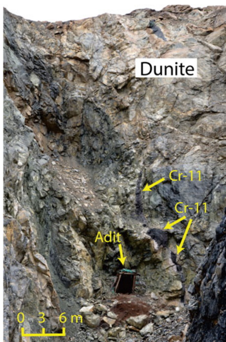
Fig. 3. Exposure showing the Cr-11 chromitite orebody from which wodegongjieite was recovered, Luobusa ophiolite, Tibet, China. The chromitite is enveloped by dunite. From Xiong et al. (2020, figure S1(a)).
