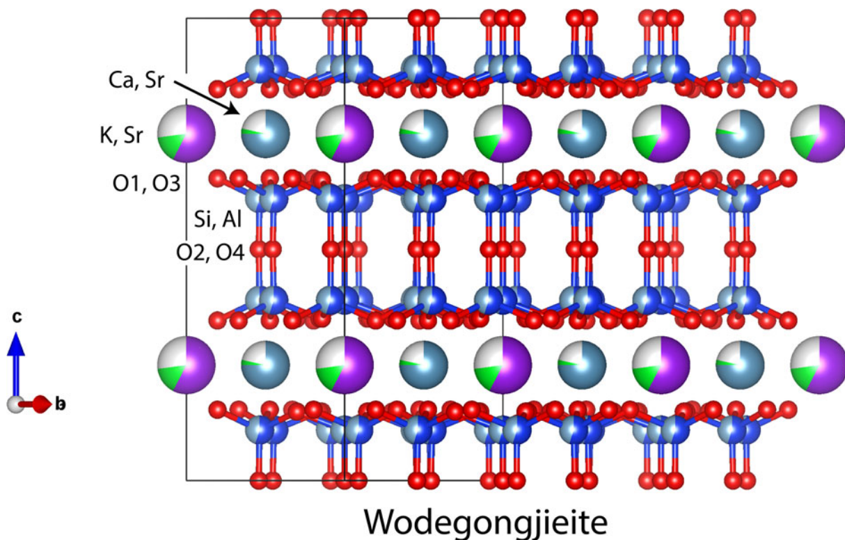
Fig. 8. View of the wodegongjieite structure along [1\bar{1}0] . Drawn using Vesta (Momma and Izumi, 2011).
