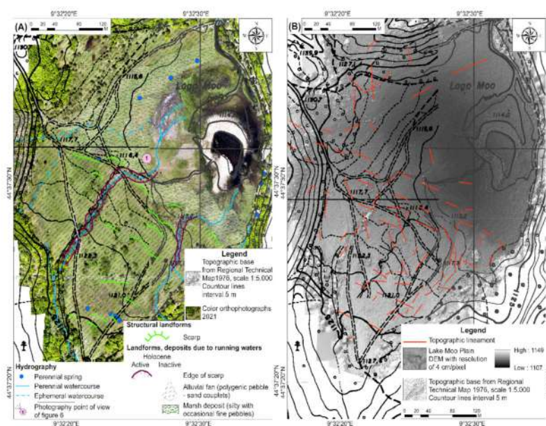
Figure 7. The main structural landforms and topographic lineament recognized in the lake Moo plain extracted from (A) high-resolution orthophotograph and (B) DEM, respectively.
