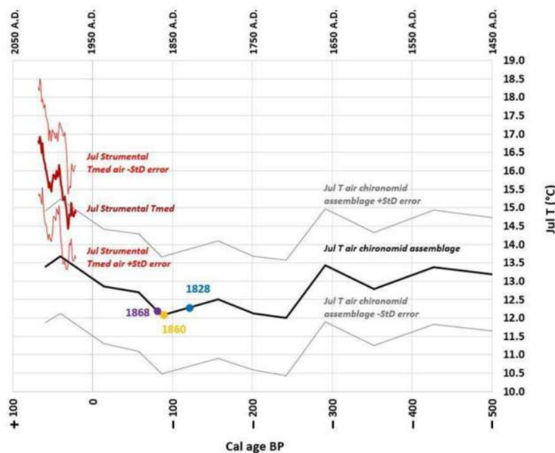
Figure 10. The black line shows the reconstructed temperature, while the gray lines are the sample-specific estimated standard error associated with the temperature reconstruction based on chironomid assemblages from [24]. The dark red line represents the July mean temperature (1971–2018) retrieved for the Verdarolo meteorological station of ARP Ae-SIMC network Emilia-Romagna Region (11-year running average). The light red lines are standard deviation error.
