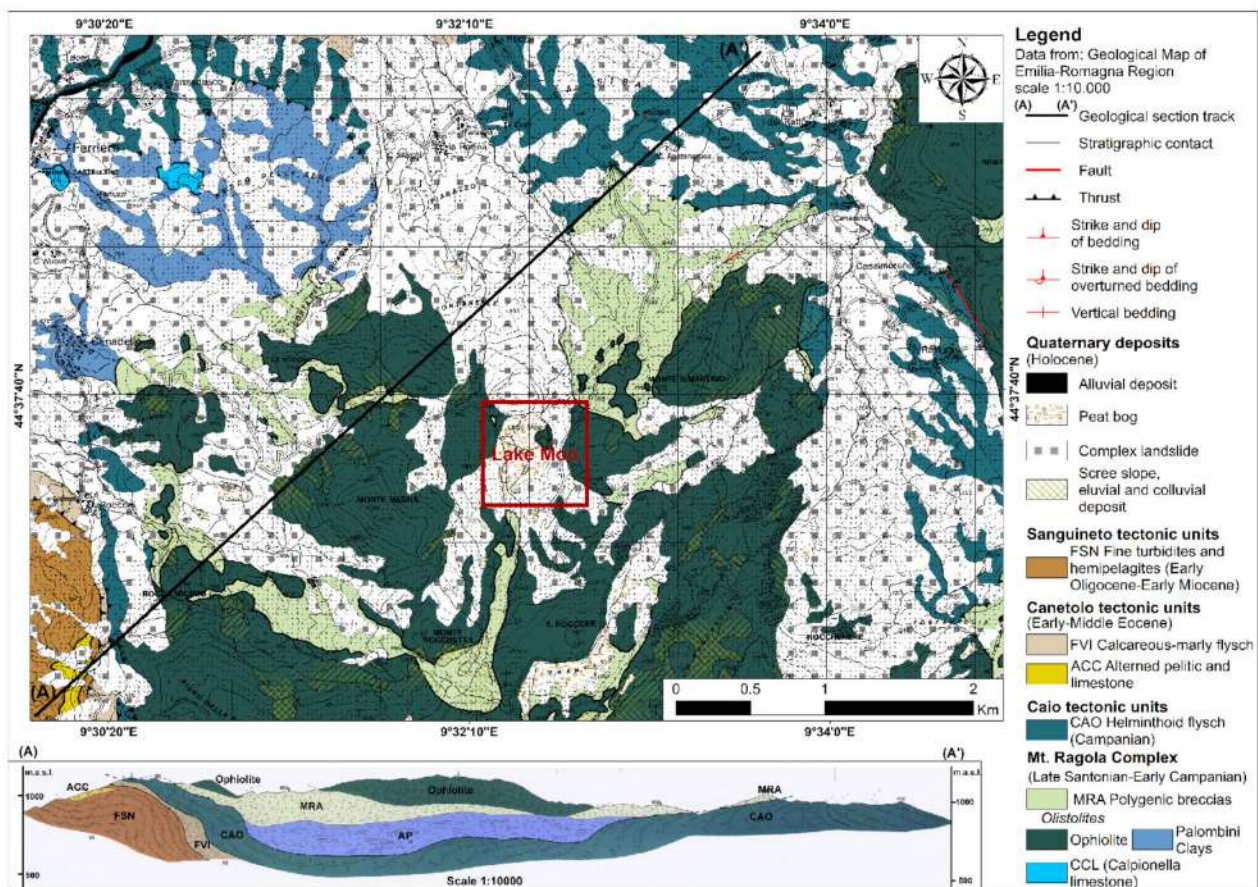
Figure 3. Map and geological cross-section of the Mt. Ragola ophiolitic massif with location of the study area. Modified from [11].
