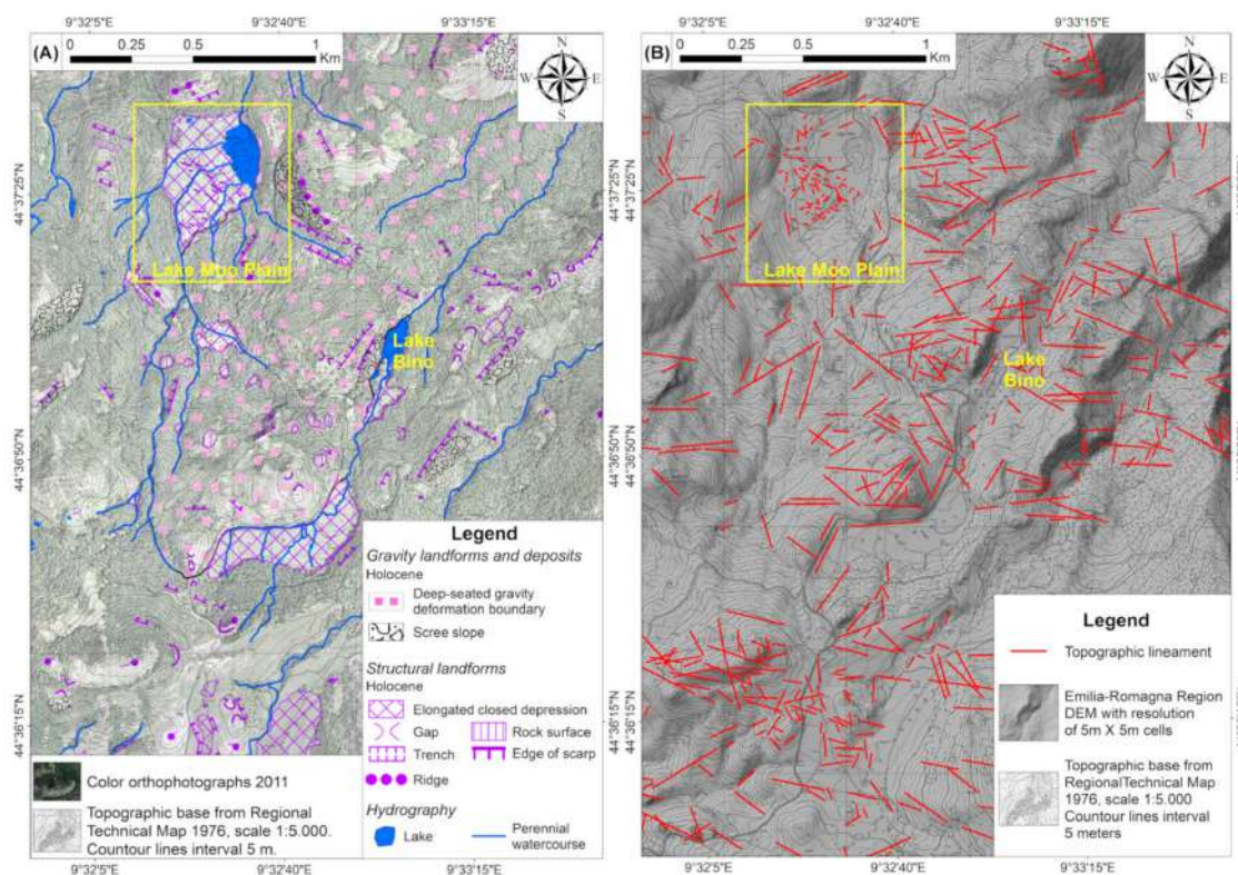
Figure 9. Main geomorphological features surrounding the study area. (A) Map of geomorphic structures. (B) Map of topographic lineaments.
