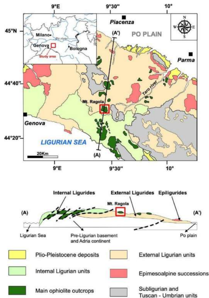
Figure 1. Tectonic sketch map and geological cross-section of the Northern Apennines (modified from [2]) with location of the study area (red box).
