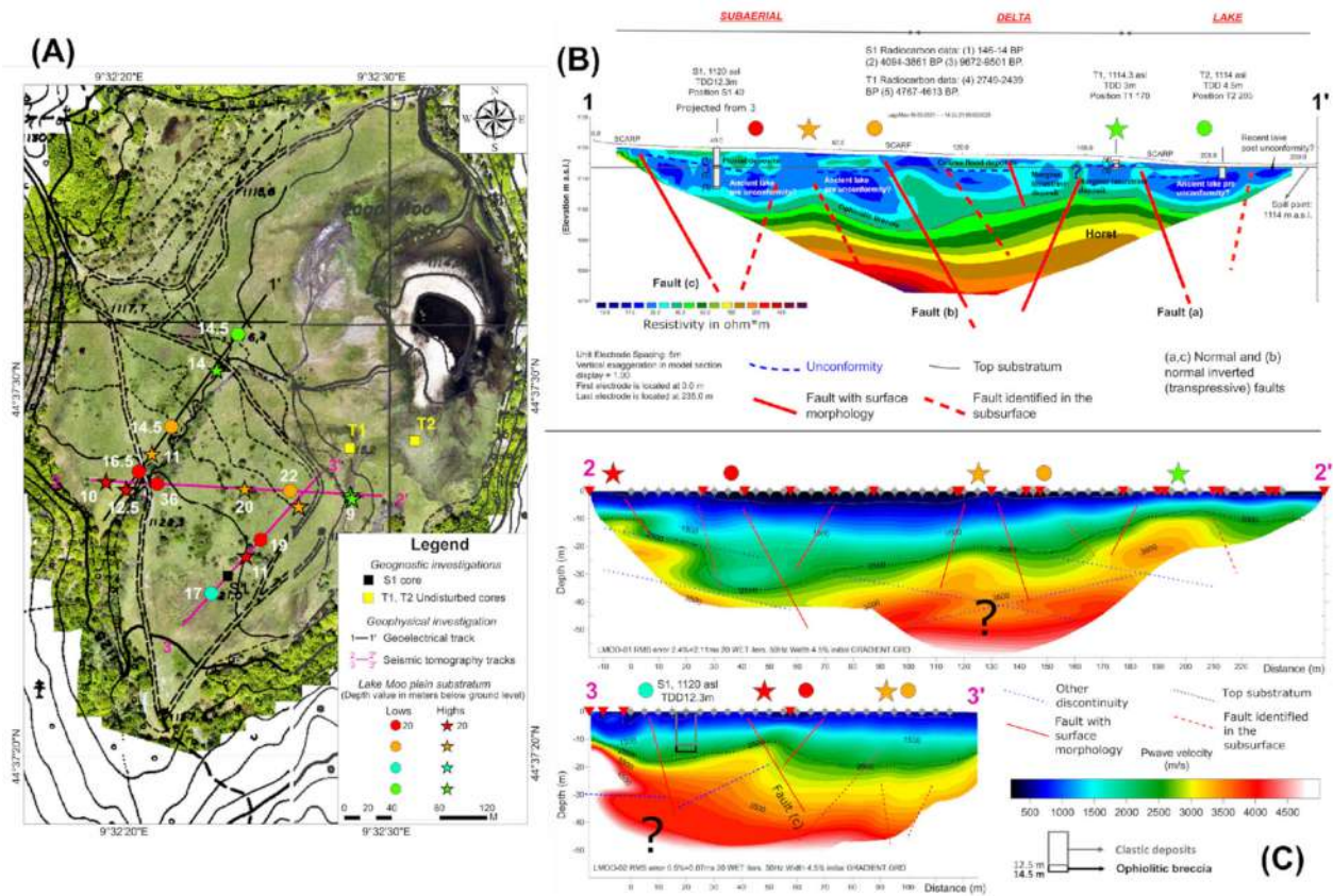
Figure 8. (A) Location of the geophysical profiles shown in (B,C) with labeling of the correlated structural highs and lows of the ophiolitic substrate. (B) Geoelectrical resistivity tomography and interpretation. The depth of the unconformity is in accordance with the spill point altitude of Lake Moo (1114 m a.s.l.). (C) Vp seismic tomography profiles (modified from [10], © Author(s) 2020, Creative Commons Attribution 4.0 License; https://cp.copernicus.org/articles/16/1547/2020/cp-16-1547-2020-supplement.pdf , accessed on 11 April 2022), and interpretation. Question marks outline areas with ambiguous and/or unclear results.
