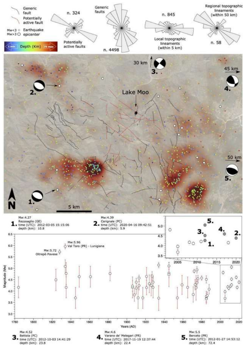
Figure 12. Heatmap overlay of earthquake epicenters, color coded by depth (time interval 1541–2021; [24]), on Google Earth satellite imagery of the area surrounding the Lake Moo basin, with rose diagrams summarizing the main structural orientations. Generic fault and potentially active fault data from [1] and [23], respectively. In the bottom diagram, chronological distribution of historical M > 3 seismic events occurred in an area of 50 km radius around Lake Moo. Data from [24]. The main M > 4 earthquakes with available reconstructed focal mechanisms are labeled.
