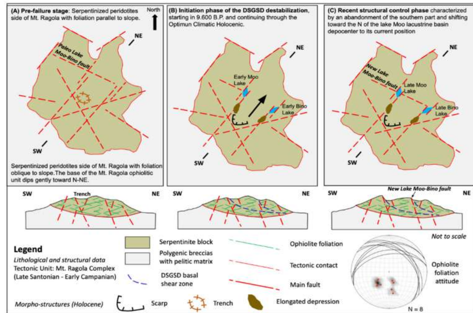
Figure 11. Synthetic conceptual model showing the origin and subsequent evolution of the Moo and Bino lakes. (A) Pre-failure stage: Serpentinized peridotites side of Mt. Ragola with foliation parallel to slope; (B) Initiation phase of the DSGSD destabilization, starting in 9.600 B.P. and continuing through the Holocene Climatic Optimum; (C) Recent structural control phase characterized by an abandonment of the southern part and shifting toward the N of the lake Moo lacustrine basin depocenter to its current position.
