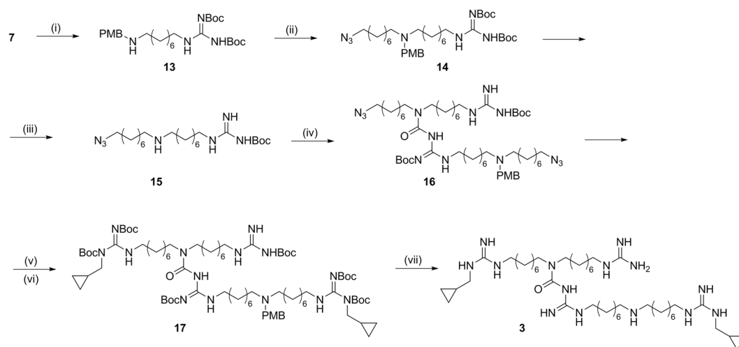
Figure 7. Synthesis of asymmetric dimer (3). Reagents and conditions: (i) 1) p -Anisaldehyde, CH 3 OH, r.t., 3 h; 2) NaBH 4 , 0 °C, 1 h; (ii) 6, NaI, DMF, r.t., 48 h; (iii) CAN, t -BuOH/CH 3 OH, 55 °C, 5 h; (iv) 14, TEA, dry THF, ref., 2 h; (v) H 2 , Pd/C, i -PrOH, r.t., 16 h; (vi) N,N' -Di-Boc- N -methylcyclopropyl-pyrazole-1-carboxamide, DIPEA, THF, r.t., 16 h; (vii) TFA 10%, dry DCM, r.t., 7 h.
