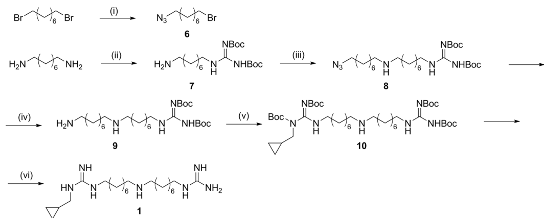
Figure 5. Synthesis of monomer ( 1 ). Reagents and conditions: (i) \text{NaN}_3 , DMF, 50 °C, 16 h; (ii) 1,3-Bis(tert-butoxycarbonyl)-2-methyl-2-thioisourea, DIPEA, \text{CH}_3\text{CN}/\text{CH}_3\text{OH} , 40 °C, 16 h; (iii) \text{CsOH}\cdot\text{H}_2\text{O} , molecular sieves, 6 , dry DMF, r.t., 24 h; (iv) \text{H}_2 , Pd/C, i -PrOH, r.t., 4 h; (v) N,N' -Di-Boc- N -methylcyclopropyl-pyrazole-1-carboxamide, DIPEA, THF, 16 h, r.t.; (vi) TFA 10%, dry DCM, r.t., 7 h.
