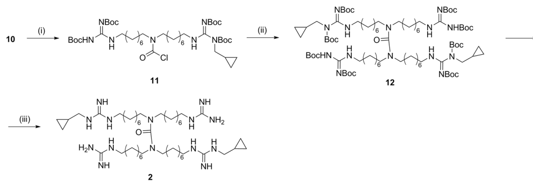
Figure 6. Synthesis of symmetric dimer (2). Reagents and conditions: (i) Triphosgene, DIPEA, dry THF, 0 °C to r.t., 10 min; (ii) 10, DIPEA, NaI, dry DCM, 40 °C, 48 h; (iii) TFA 10%, dry DCM, r.t., 7 h.
