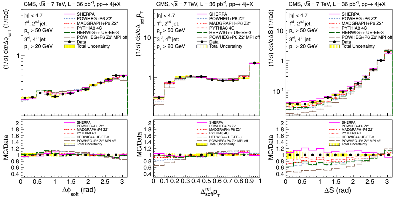
FIG. 3 (color online). Normalized differential cross sections as a function of the difference in azimuthal angle \Delta\phi_{\text{soft}} (left), \Delta_{\text{soft}}^{\text{rel}} p_T (middle), and \Delta S (right) compared to the predictions of POWHEG, MADGRAPH, SHERPA, PYTHIA 8 and HERWIG++. A comparison with the POWHEG predictions interfaced with the parton shower PYTHIA 6 tune ZZ' without MPI is also shown. The lower panel shows the ratios of the predictions to the data. The yellow band represents the total uncertainty, including the statistical and systematic components added in quadrature. Systematic uncertainties in the normalized cross sections are smaller than the ones in the absolute cross sections, since they are not affected by the migration effects from outside the selected phase space.
