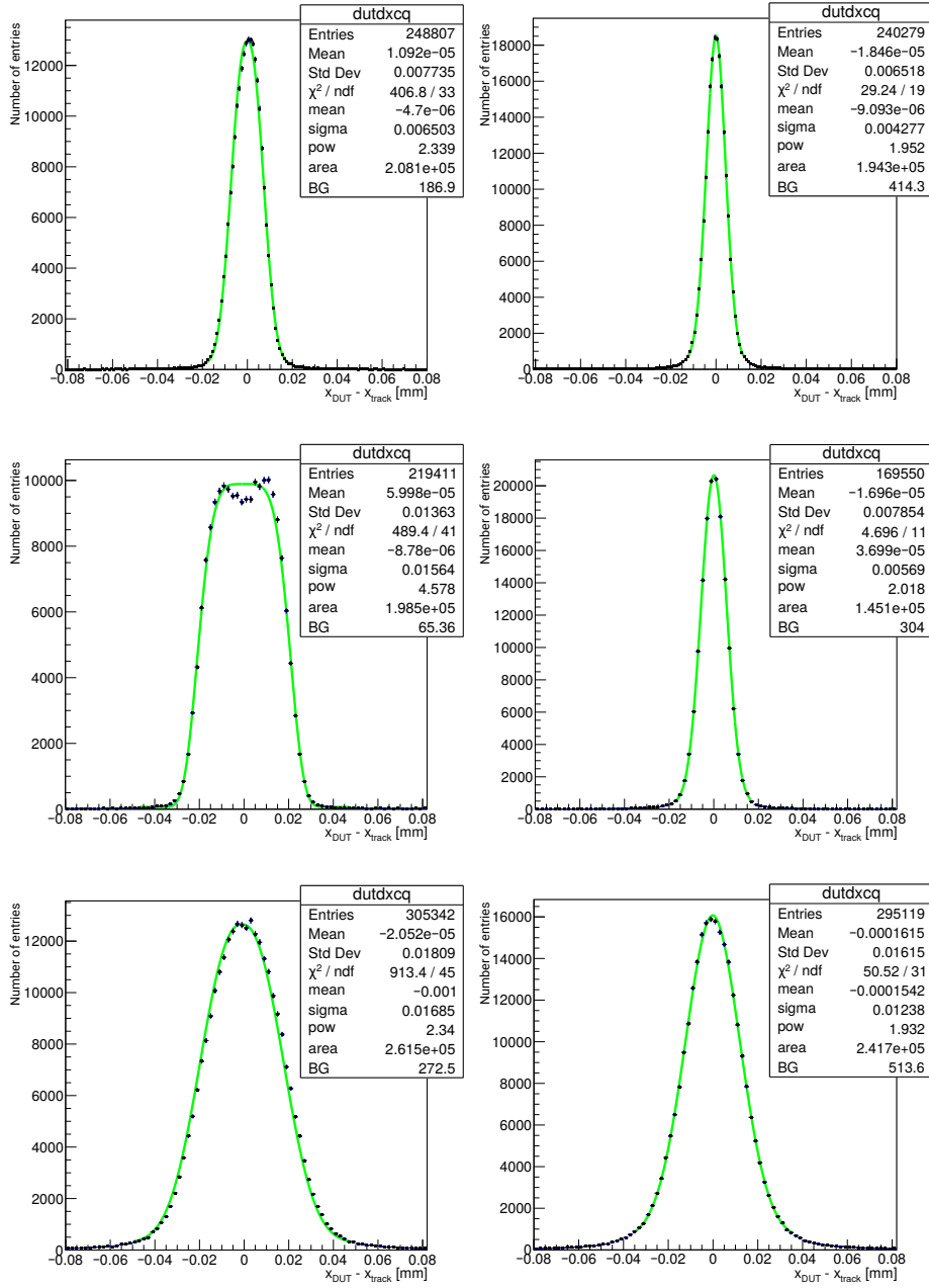
Figure 11. Residual distributions fitted with generalized error functions at vertical incidence (left) and at the optimal angle (right) for modules M563 ( 100 \mu\text{m} \times 25 \mu\text{m} sensor, non-irradiated) (top), M564 ( 50 \mu\text{m} \times 50 \mu\text{m} sensor, non-irradiated) (center), and M521 ( 50 \mu\text{m} \times 50 \mu\text{m} sensor, \Phi_{\text{eq}} = 5.3 \times 10^{15} \text{ cm}^{-2} ) (bottom). The fit parameters listed under \chi^2/\text{ndf} correspond to the parameters \mu_g, \sigma_g, S_g, A_g and B_g in equation (5.3), respectively.
