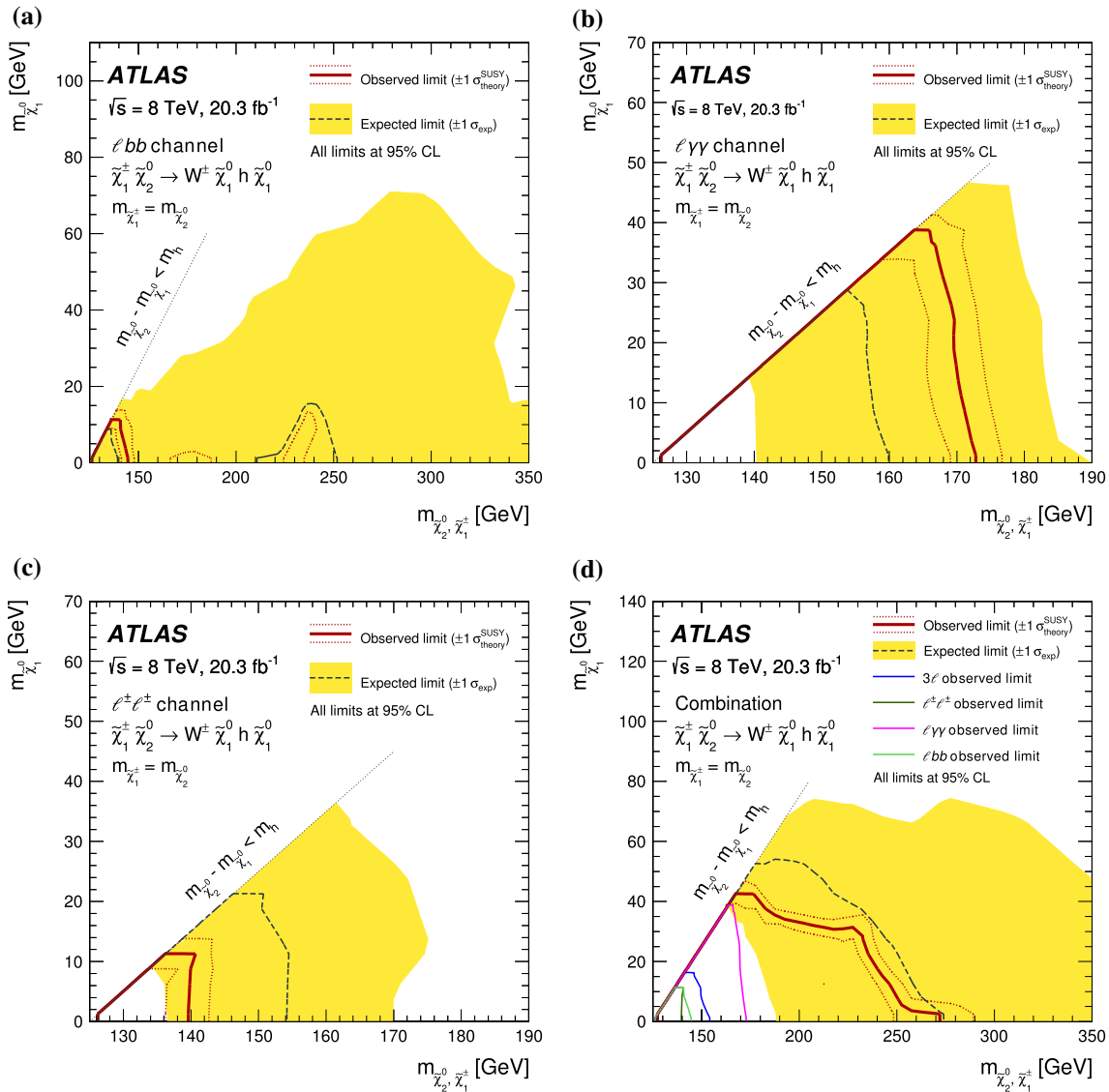
Fig. 8 Observed (solid line) and expected (dashed line) 95 % CL exclusion regions in the mass plane of m_{\tilde{\chi}_1^0} vs. m_{\tilde{\chi}_2^0, \tilde{\chi}_1^\pm} in the simplified model. The combination in d is obtained using the result from the ATLAS three-lepton search [21] in addition to the three channels reported in this paper. The dotted lines around the observed limit represent the results obtained when changing the nominal signal cross
