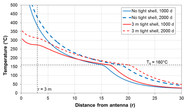
Fig. 3. Comparison between thermal profiles obtained with and without a 3 m diameter tight shell for a lossy reservoir.
