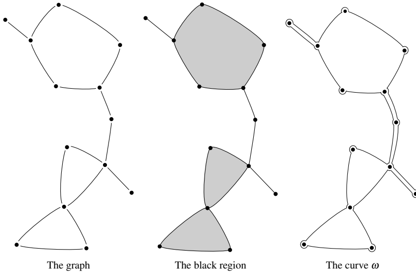
Fig. 5.1: Desingularization of a graph
