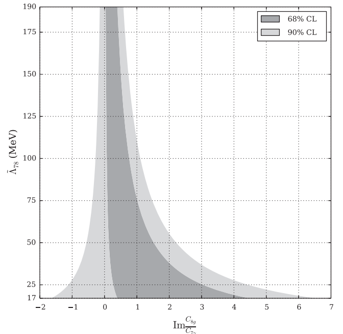
FIG. 4. The 68% and 90% confidence intervals for \text{Im} \frac{C_{8g}}{C_{7\gamma}} and \tilde{\Lambda}_{78} .
