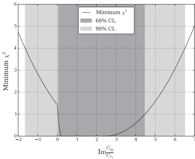
FIG. 3. The minimum \chi^2 for given \text{Im} \frac{C_{8g}}{C_{7\gamma}} from all possible values of \tilde{\Lambda}_{78} . 68% and 90% confidence intervals are shown in dark gray and light gray, respectively.
