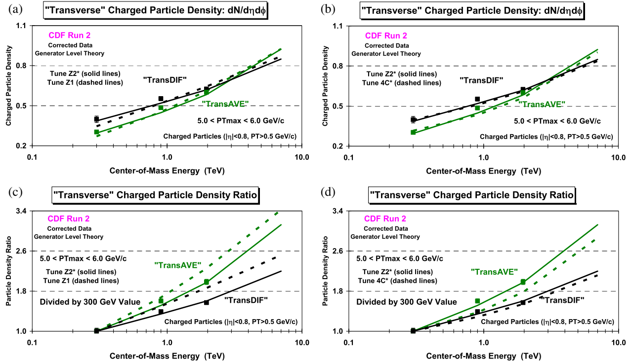
FIG. 16 (color online). (a,b) Data on the transAVE and transDIF charged particle density as defined by the leading charged particle, for 5.0 < PT_{\max} < 6.0 GeV/c plotted versus the center-of-mass energy for charged particles with p_T > 0.5 GeV/c and |\eta| < 0.8 . (c,d) Ratio of the data at 1.96 TeV, 900 GeV, and 300 GeV to the corresponding value at 300 GeV plotted versus the center-of-mass energy. The data are corrected to the particle level with errors that include both the statistical error and the systematic uncertainty, and are compared with PYTHIA Tune Z1 and Z2* (a,c) and PYTHIA Tune Z2* and 4C* (b,d). The theory curves include the predictions of the PYTHIA tunes at 7 TeV.
