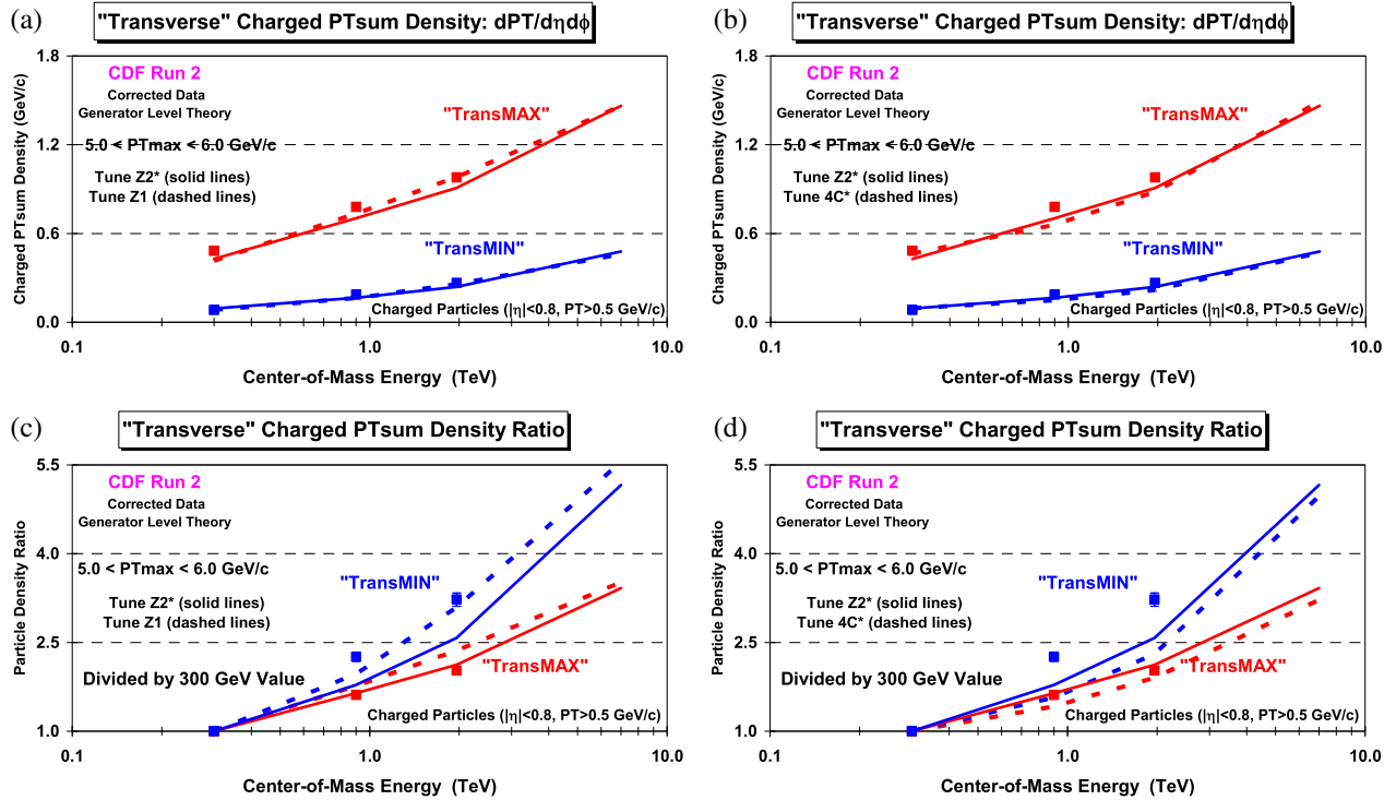
FIG. 15 (color online). (a,b) Data on the transMAX and transMIN charged PTsum density as defined by the leading charged particle, for 5.0 < PT_{\max} < 6.0 GeV/c plotted versus the center-of-mass energy for charged particles with p_T > 0.5 GeV/c and |\eta| < 0.8 . (c,d) Ratio of the data at 1.96 TeV, 900 GeV, and 300 GeV to the corresponding value at 300 GeV plotted versus the center-of-mass energy. The data are corrected to the particle level with errors that include both the statistical error and the systematic uncertainty, and are compared with PYTHIA Tune Z1 and Z2* (a,c) and PYTHIA Tune Z2* and 4C* (b,d). The theory curves include the predictions of the PYTHIA tunes at 7 TeV.
