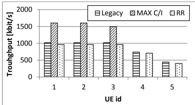
Fig. 9. Average user throughput with three scheduling algorithms and CBR traffic with a payload size of 150 Bytes.
