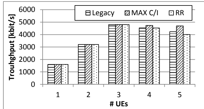
Fig. 10. Average cell throughput with three scheduling algorithms, 1 to 5 UEs, and CBR traffic with a payload size of 150 Bytes.
