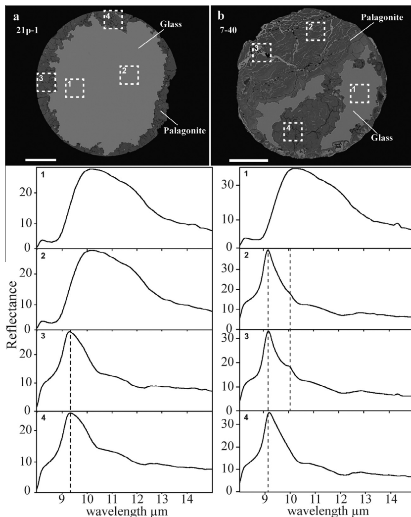
Fig. 7. Mid-infrared reflectance spectra on 50 \times 50 \mu\text{m} areas of V-type cosmic spherules s #21p.1 (a) and #7.40 (b). Spectra were acquired over pristine glass (a1–2 and b1) and altered glass (a3–4 and b2–3). In the spectra b2 and b3 sharp band is observed at \sim 10 \mu\text{m} (dashed line), which can be attributed to sulphate (Bishop and Murad, 2005).
