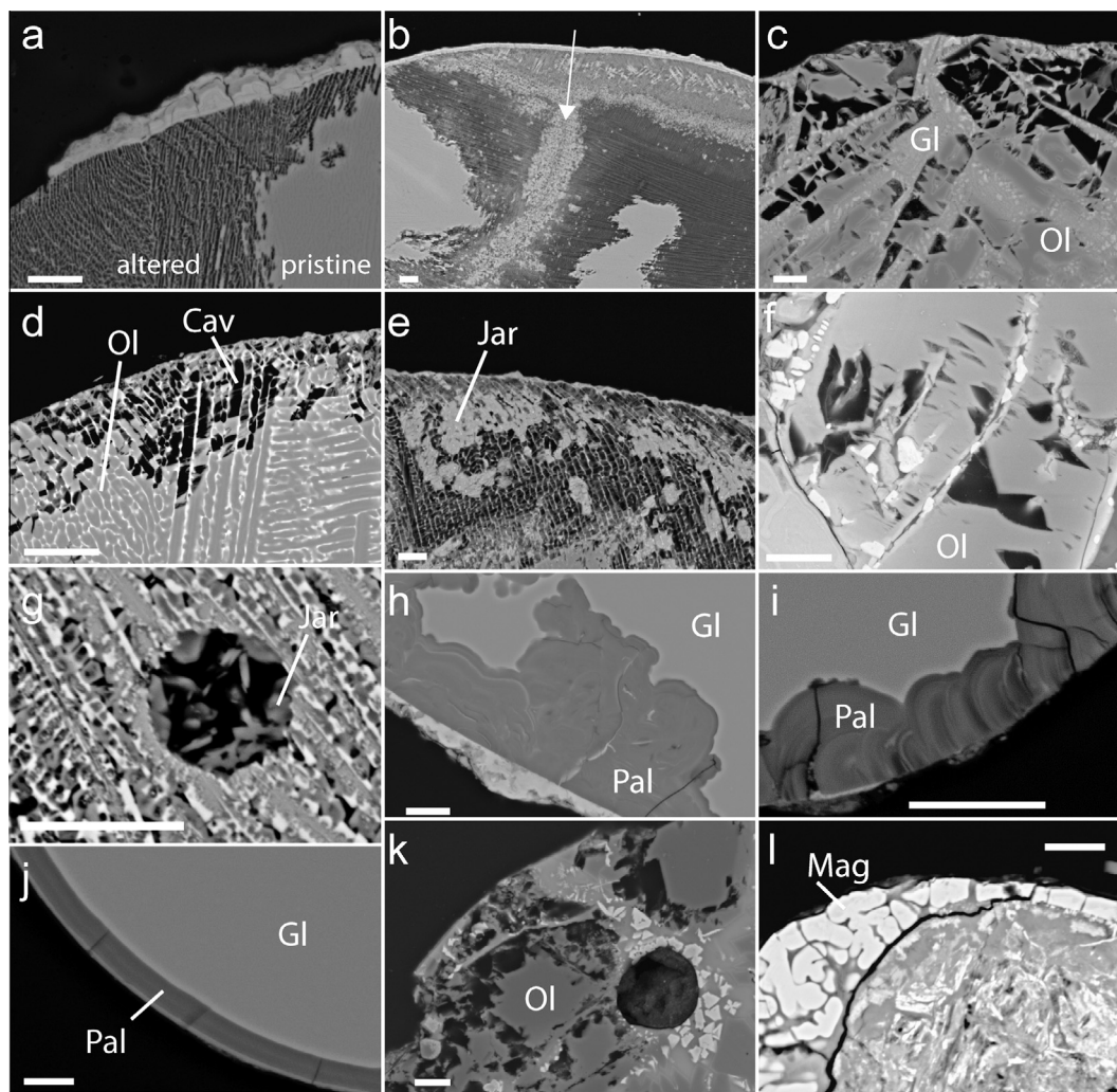
Fig. 3. Scanning electron microscope backscattered electrons images of details of weathering features in cosmic spherules. (a) and (b) Dissolution features of olivine crystals in CC cosmic spherules. The arrow in (b) indicates a crack along which weathering has progressed. (c) Dissolution features in olivine crystals of Po CSs. (d) and (e) Areas where olivine has been dissolved in BO cosmic spherules. Note that in (e) jarosite has partially replaced dissolved olivine crystals. (f) Details of wedge and diamond-shaped etch pits in a Po cosmic spherule. (g) Jarosite crystals encrusting a vesicle in BO cosmic spherule #LK06-0526. (h) An isolated corrosion pit in a V-type cosmic spherule. (i) Discontinuous laminated layer in a V-type cosmic spherule. (j) Continuous leached layer in a V-type cosmic spherule. (k) Dissolution features in olivine crystals in a coarse-grained cosmic spherule. (l) Close-up of an altered FeNi metal in G-type cosmic spherule #LK06-0027 that is enclosed in magnetite. The scale bars are 20 \mu\text{m} . Abbreviations: Ol = olivine; Gl = glass; Pal = palagonite-like gel; Mag = magnetite; Met = FeNi metal; Cav = cavity.
