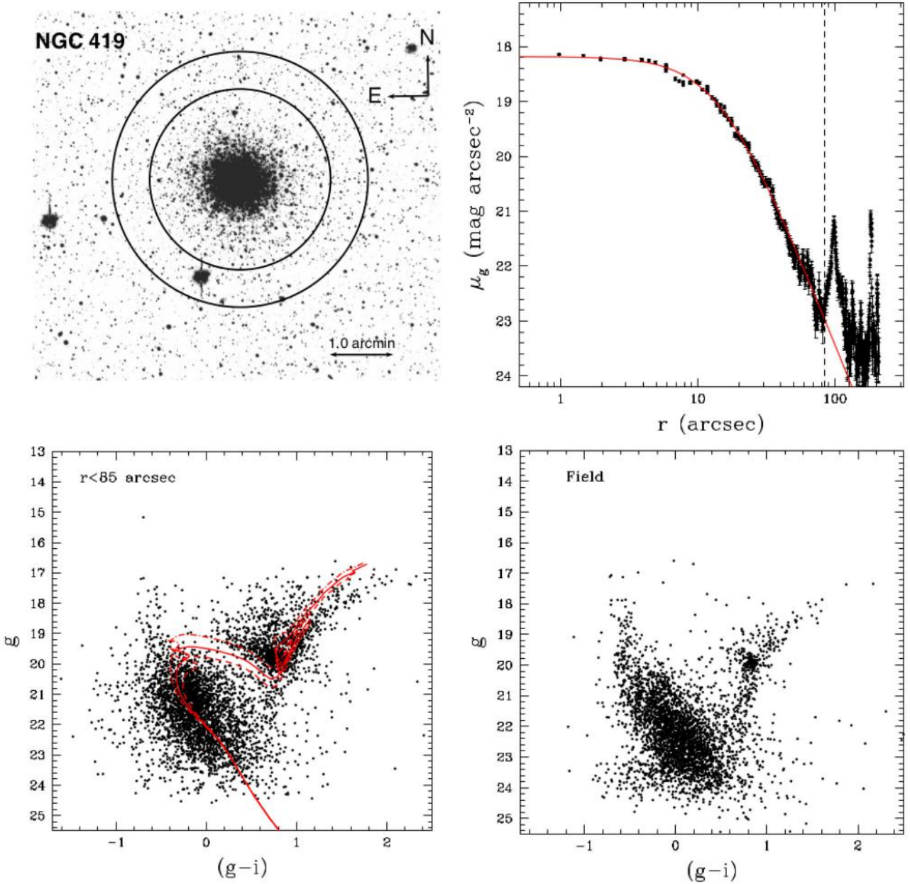
Figure 21. Upper-left panel: cluster map; the two circles have radii of 85 and 120 arcsec, respectively. Upper-right panel: black dots show the observed radial stellar SBP around the NGC 419 centre, whereas the solid red line shows the profile fitting obtained with equation (2), while the dashed line represents the fitting radius (see text). Lower-left panel: CMD of the cluster within the fitting radius (see text). Lower-right panel: field stars in an annulus with inner and outer radii of 85 and 120 arcsec, respectively. This annulus has the same area as the innermost circle.
