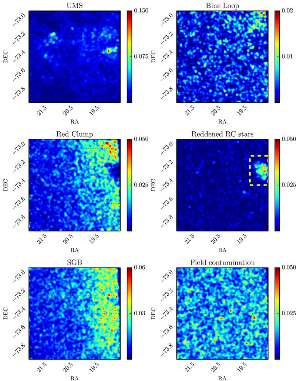
Figure 16. Tile 3_7. Spatial distributions of labelled CMD selections (see Fig. 15). Maps are produced by calculating a 2D histogram of stellar positions and then smoothing the result with a Gaussian kernel. The yellow dashed box (in the middle-right panel) highlights a sub-region where reddening is above the average (see Fig. 17).
