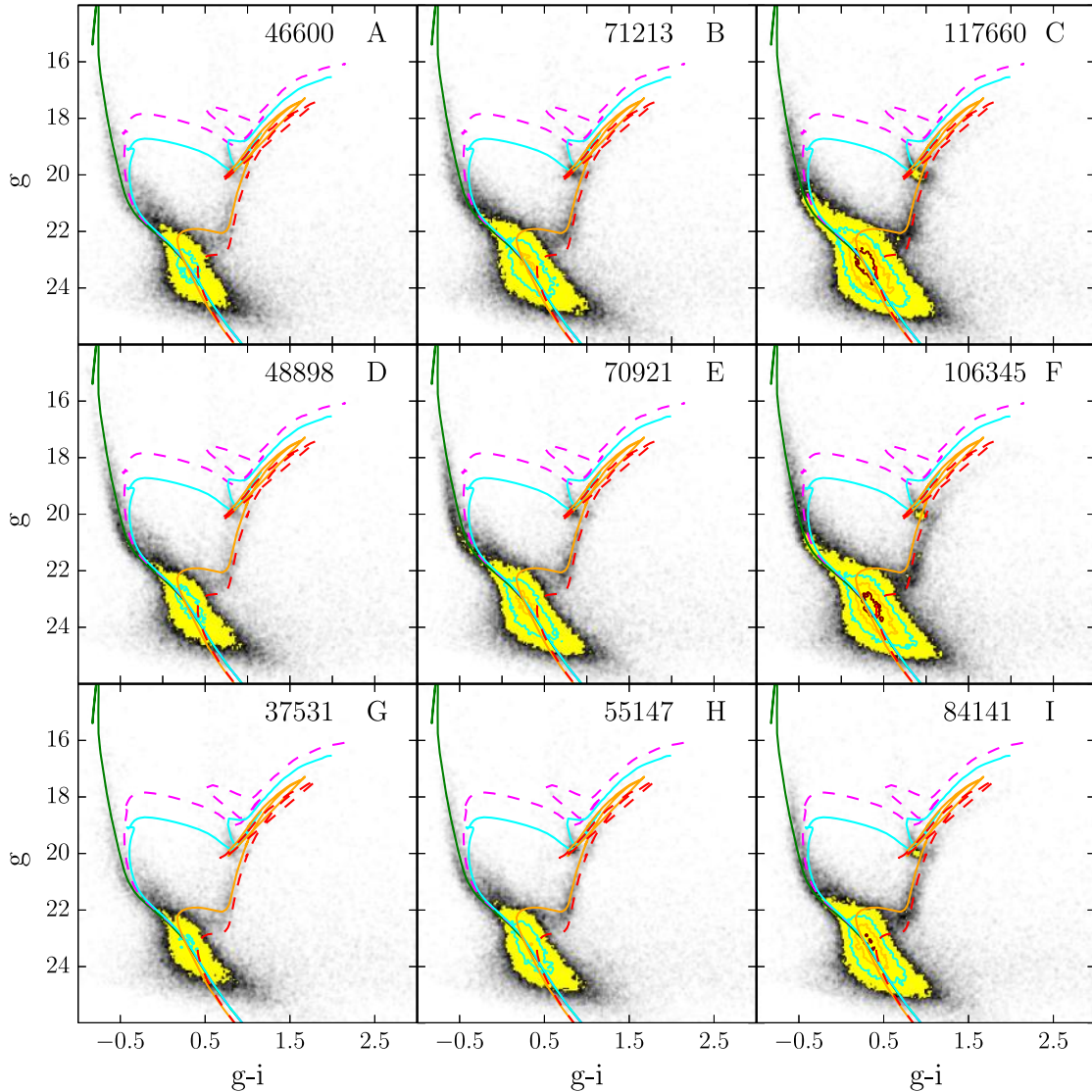
Figure 14. CMDs for nine 20 arcmin \times 21 arcmin sub-regions of tile 3_7. The isochrone ages and metallicities are the same as in Fig. 12. Assumed distance modulus and reddening E(B - V) are 18.9 and 0.08 mag, respectively.
