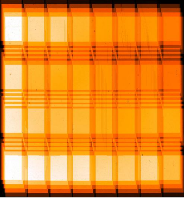
Figure 3. Typical weight map for a VST mosaic ( \sim 1 \text{ deg}^2 ) obtained with the ‘5-point diag’ pattern using steps of \pm 25 arcsec in X and \pm 85 arcsec in Y . The lighter regions are those with higher S/N.
