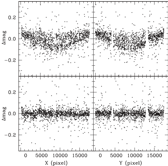
Figure 8. Residuals (VST-SDSS) versus x and y position before (top panels) and after (bottom panels) the IC correction.
