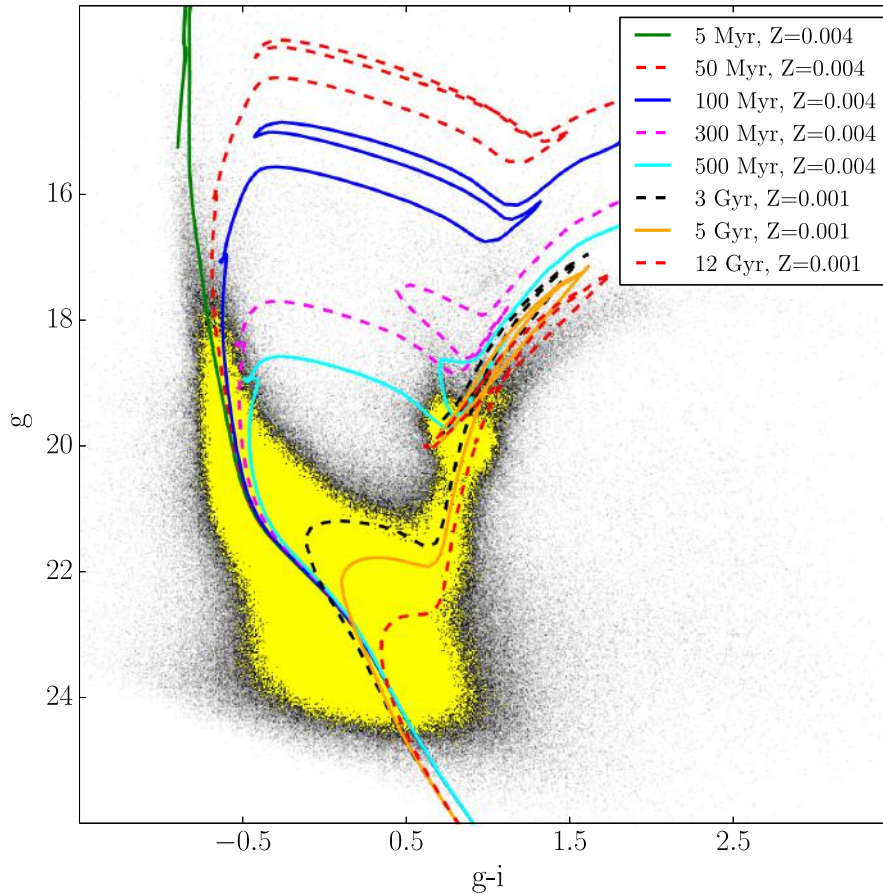
Figure 18. CMD of tile 4_6. The isochrone ages and metallicities are the same as in Fig. 12. Assumed distance modulus and reddening E(B - V) are 18.9 and 0.04 mag, respectively.
