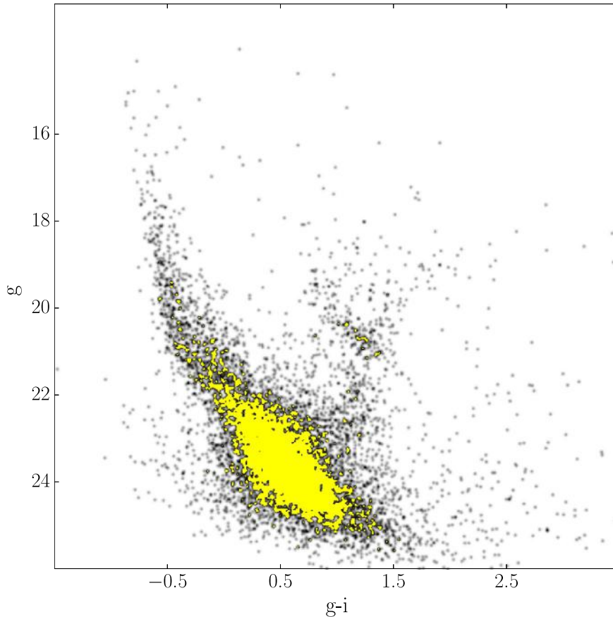
Figure 17. CMD for reddened stars in the tile 3_7 (yellow-dashed box in the middle-right panel of Fig. 16.)
