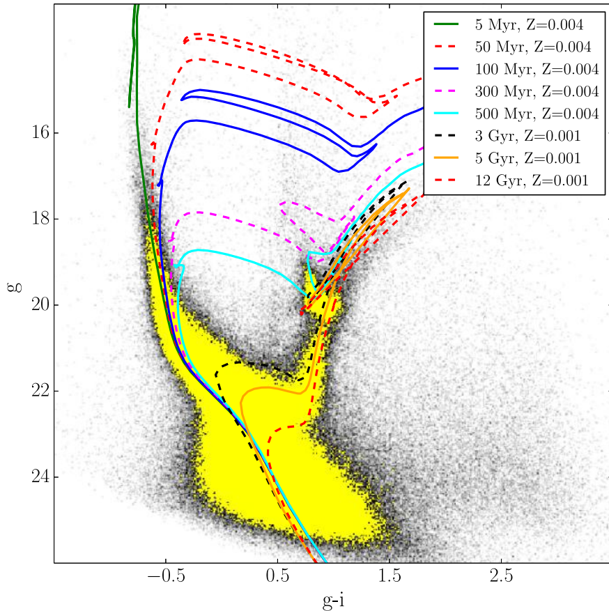
Figure 12. CMD of tile 3_7 with overlaid Marigo et al. (2008) stellar isochrones for metal abundance Z = 0.004 , ages 5 Myr (green continuous line), 50 Myr (red dashed line), 100 Myr (blue continuous line), 300 Myr (pink dashed line) and 500 Myr (cyan continuous line); Z = 0.001 , ages 3 Gyr (black dashed line), 5 Gyr (orange continuous line) and 12 Gyr (dashed red line). Assumed distance modulus and reddening E(B - V) are 18.9 and 0.08 mag, respectively.
