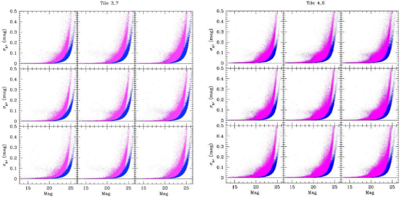
Figure 10. Photometric errors in g (blue) and i (magenta) for tiles 3_7 and 4_6. To verify the presence of possible differences within each image, the tiles were divided into nine sub-frames 20 arcmin \times 21 arcmin each. North is up and east is to the left.
