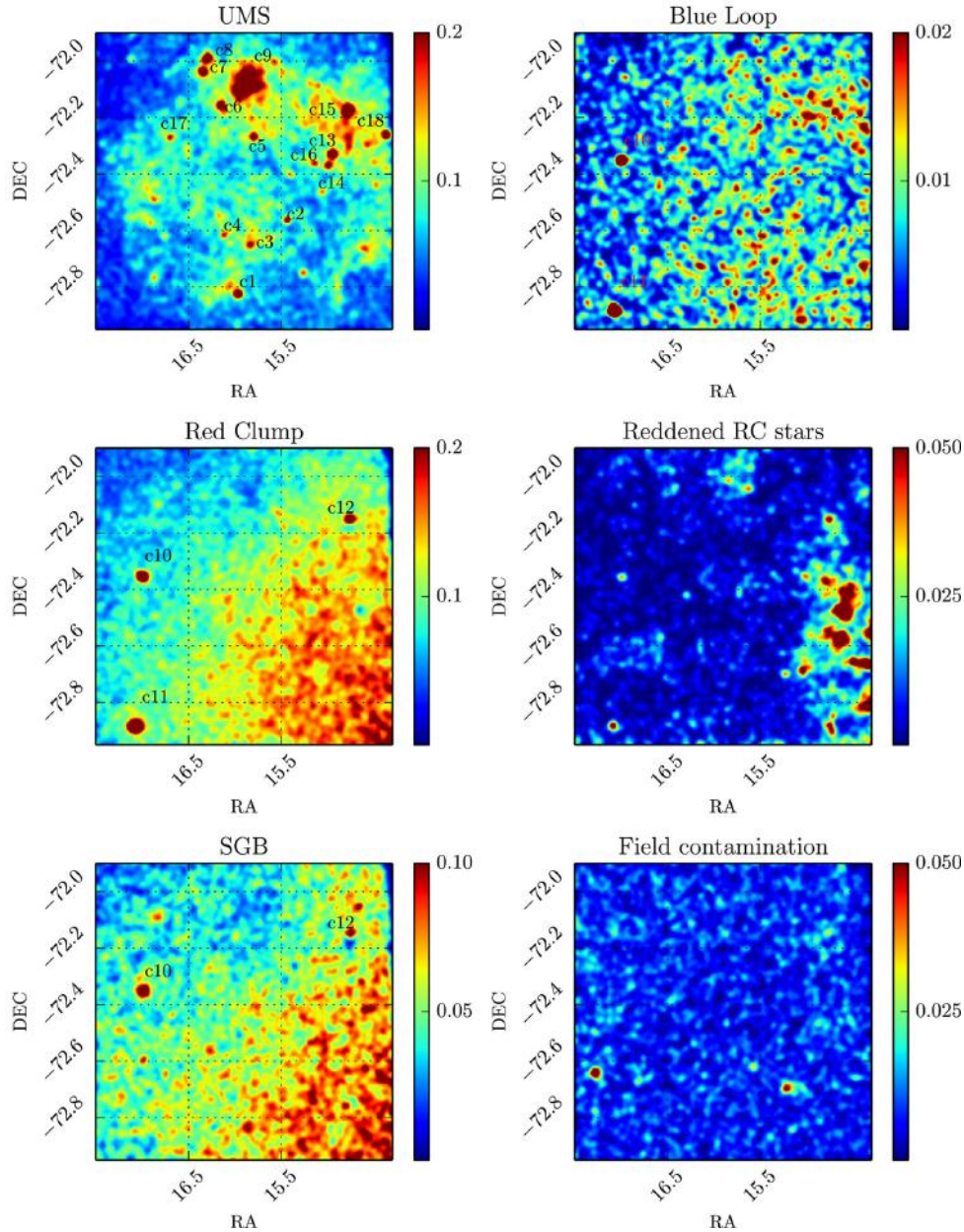
Figure 20. Tile 4_6. Spatial distributions of labelled CMD selections. Labels c1 to c18 indicate clusters identified by eye.
