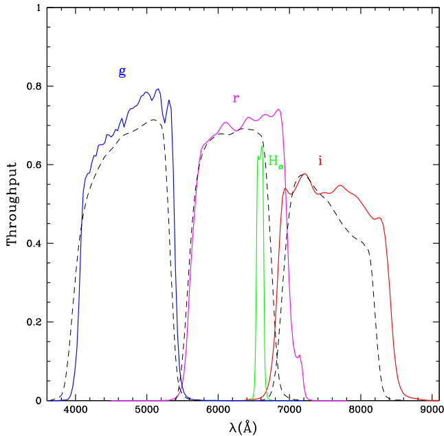
Figure 1. Transmittance of the filters used in STEP (solid lines). The contribution of the CCD is included. The dashed curves represent the transmission curves for the corresponding SDSS filters (properly rescaled to favour the comparison).
