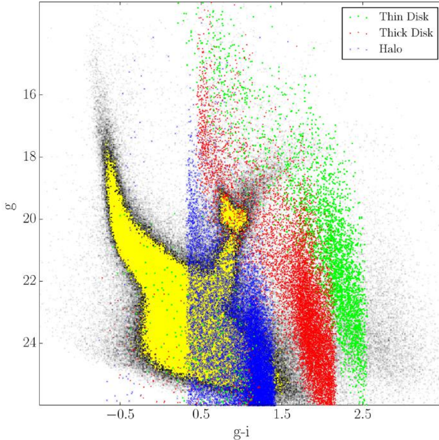
Figure 13. CMD of tile 3_7 with overlaid a simulation of MW contamination expected in the FoV. Halo stars are in blue, thick disc stars in red and thin disc stars in green.
