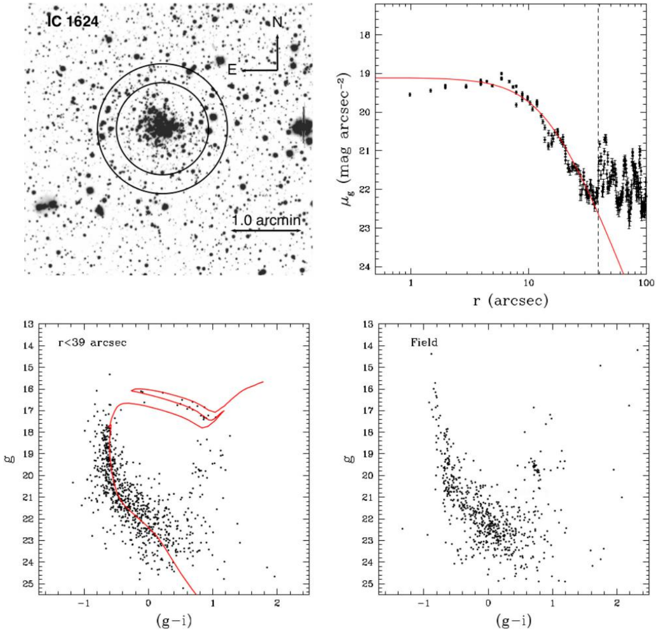
Figure 22. Same as in Fig. 21, but for cluster IC 1624. In this case, inner and outer circles have radii of 39 and 55 arcsec, respectively.
