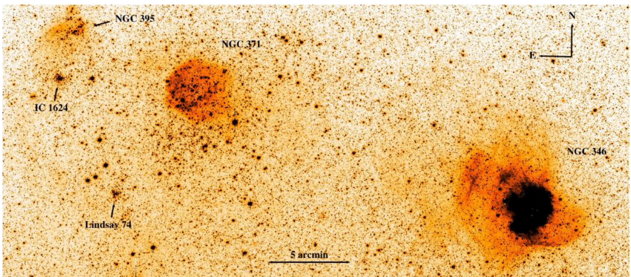
Figure 6. Enlargement of Fig. 5 showing the northern part of tile 4_6, including the well-known star-forming region NGC 346 and several other interesting clusters and associations which are labelled in the figure.
