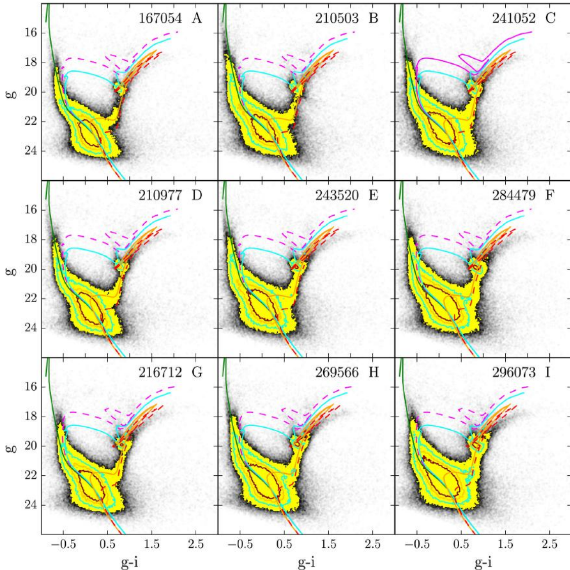
Figure 19. CMDs for nine 20 arcmin \times 21 arcmin sub-regions of tile 4_6. The isochrone ages and metallicities are the same as in Fig. 12. Assumed distance modulus and reddening E(B - V) are 18.9 and 0.04, respectively.
