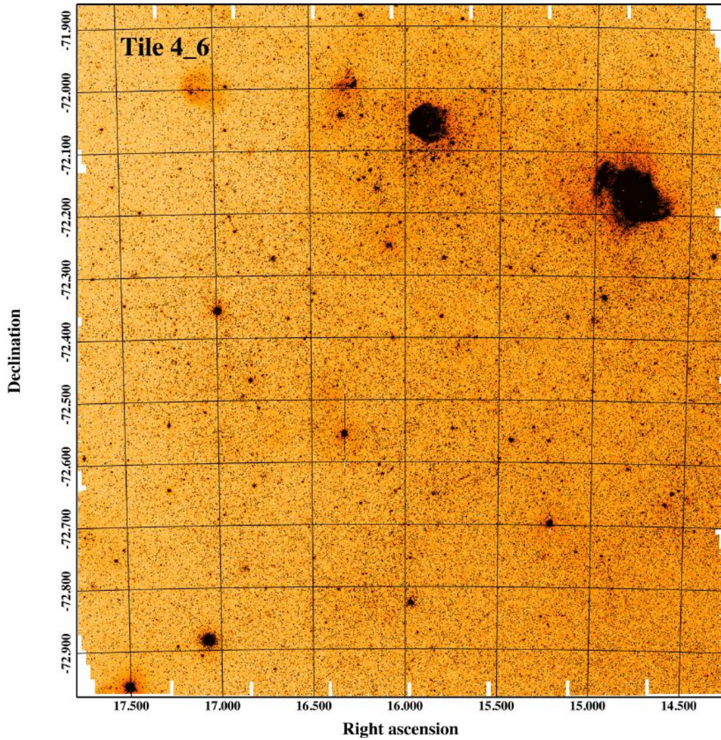
Figure 5. g -band VST plate of tile 4_6. North is up and east is to the left.
