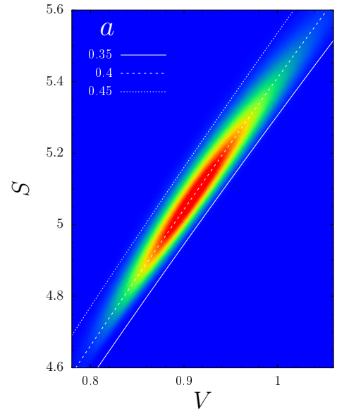
FIG. 6: Correlation plot of the surface and the volume of VPs of the melt of trimers at T = 1 (Pearson correlation coefficient r = 0.973 ). The lines are Eq.11 with the indicated values of the asphericity. The best-fit value of the asphericity ( a = 0.404 ) compares well with the average asphericity of the VPs ( \langle a \rangle = 0.405 ).
