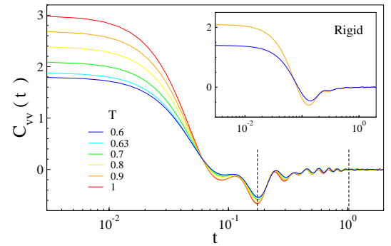
FIG. 1: Velocity correlation function of the monomers at selected temperatures. The left dashed line marks the minimum of the correlation function at time t_m = 0.175 . The position of the right dashed line is the time t^* = 1.023 defined in Fig.2 and marks the end of the exploration of the cage by the trapped particle. During the selected time window ( t_m \lesssim t \lesssim t^* ) the coupling with the solid-like collective motion of the surroundings develops, see Sec.III D. The fast oscillations superimposed to the slower decay are largely due to the bond vibrations and are mostly suppressed by replacing the semirigid bond with a rigid one (see inset). The residual oscillations observed after the minimum in the presence of rigid bonds are ascribed to collective density waves in analogy with atomic liquids like rubidium [1].
