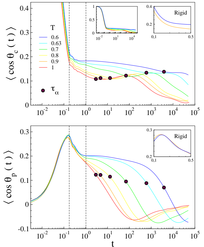
FIG. 4: Local anisotropies of the cage rattling. Top: \langle \cos \theta_c(t) \rangle , Eq.8, at different temperatures. The unlabeled inset shows the complete decay. Bottom: \langle \cos \theta_p(t) \rangle , Eq.9. The dots mark the structural relaxation time \tau_\alpha . The left dashed line marks the minimum of the velocity correlation function at t = t_m , see Fig.1. The right dashed line marks the time needed by the trapped particle to explore the cage t^* , see Fig.2. Up to t \sim 0.65 \langle \cos \theta_p(t) \rangle is nearly temperature-independent. The maximum of \langle \cos \theta_p(t) \rangle signals that the particle, as in atomic systems [90], tends initially to move to the centroid. The insets labelled as "Rigid" plot the anisotropies for T = 0.6, 0.9 having replaced the semirigid bond with a rigid one and leaving any other parameter unchanged. They evidence that the oscillations in the time window t_m \lesssim t \lesssim t^* of the main panels are due to the finite stiffness of the bond.
