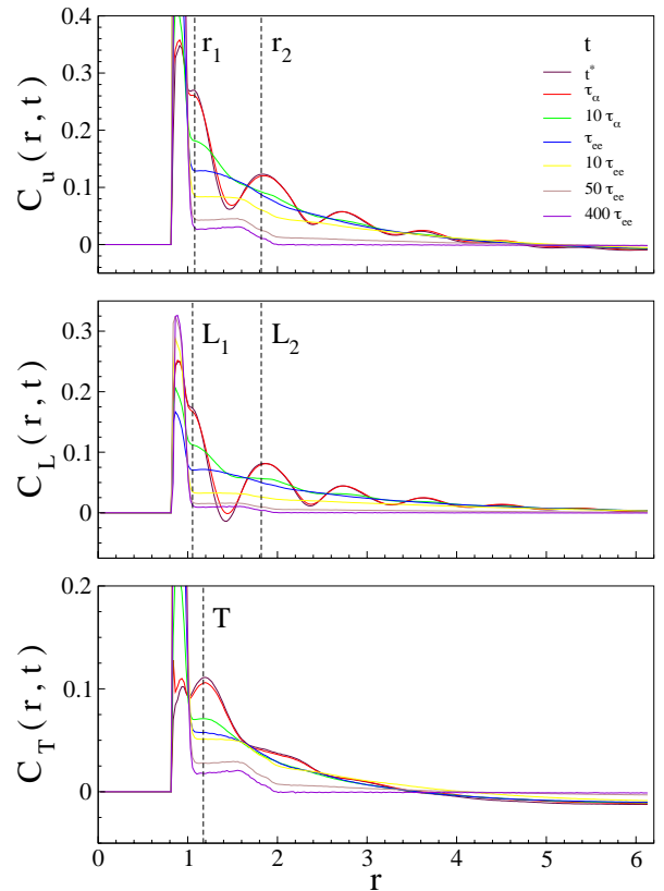
FIG. 11: Spatial distribution of the correlations between the simultaneous overall (top), Eq.14, longitudinal (middle), Eq.18, and transverse (bottom), Eq.19, components of the displacements of the central particle and the surrounding particles at distance r for different times t \geq t^* = 1.023 and T = 1 . At the selected temperature \tau_\alpha = 3 and the average molecular reorientation time \tau_{ee} = 126 [16].
