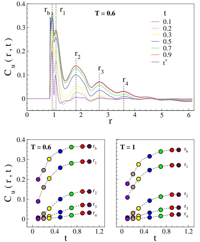
FIG. 9: Top panel: spatial distribution C_u(r, t) of the correlations between the simultaneous displacements of the central particle and the surrounding particles at distance r for different times t and T = 0.6 . The time window starts at t = 0.1 < t_m = 0.175 and ends at t^* = 1.023 . The peak positions correspond nearly to the ones of the radial distribution function [44, 45]. At constant density they do not depend on the temperature. Bottom panels: onset of the correlations at the peak positions at T = 0.6 (left) and T = 1 (right). r_b = b equals the bond length distance.
