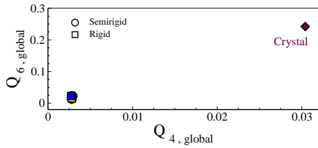
FIG. 13: Global order parameters Q_{6,global} and Q_{4,global} . The crystalline state is the same considered in Fig.2 and is the only state exhibiting global order.
