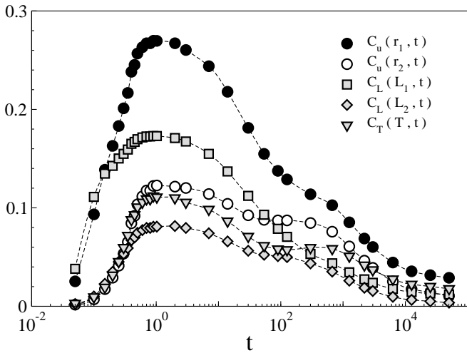
FIG. 12: Time dependence of the overall, longitudinal and transverse correlations at the indicated positions in Fig.11. At the selected temperature \tau_\alpha = 3 and the average molecular reorientation time \tau_{ee} = 126 [16]. The time window starts before t_m = 0.175 . Note the maximum at about t^* = 1.023 .
