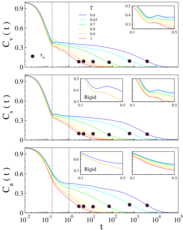
FIG. 8: Correlation functions, Eq.12, of volume (top), surface (middle) and asphericity (bottom) of VPs at different temperatures. The dashed lines mark the region t_m \leq t \leq t^* as in Fig. 1 and Fig. 4. Insets: magnification of the oscillatory behavior at intermediate times. The insets labelled as "Rigid" plot the correlation function for T = 0.6, 0.9 having replaced the semirigid bond with a rigid one and leaving any other parameter unchanged. They evidence that the oscillations are not due to the finite stiffness of the bond but to the elastic response of the local structure.
