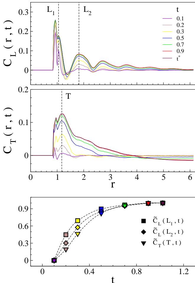
FIG. 10: Spatial distribution of the correlations between the simultaneous longitudinal (top), Eq.18, and transverse (middle), Eq.19, components of the displacements of the central particle and the surrounding particles at distance r for different times t and T = 0.6 . The time window starts at t = 0.1 < t_m = 0.175 and ends at t^* = 1.023 . The lower panel plots the growth of the correlation, Eq.21, at selected positions. The longitudinal correlations increase faster than the transverse ones.
