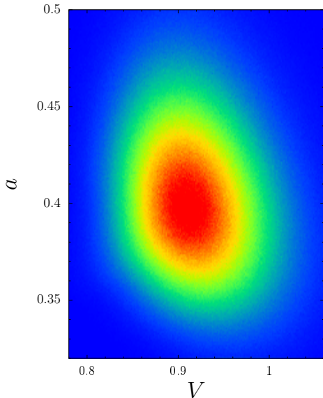
FIG. 5: Correlation plot of the asphericity and the volume of VPs of the melt of trimers at T = 1 . No correlation is apparent.
