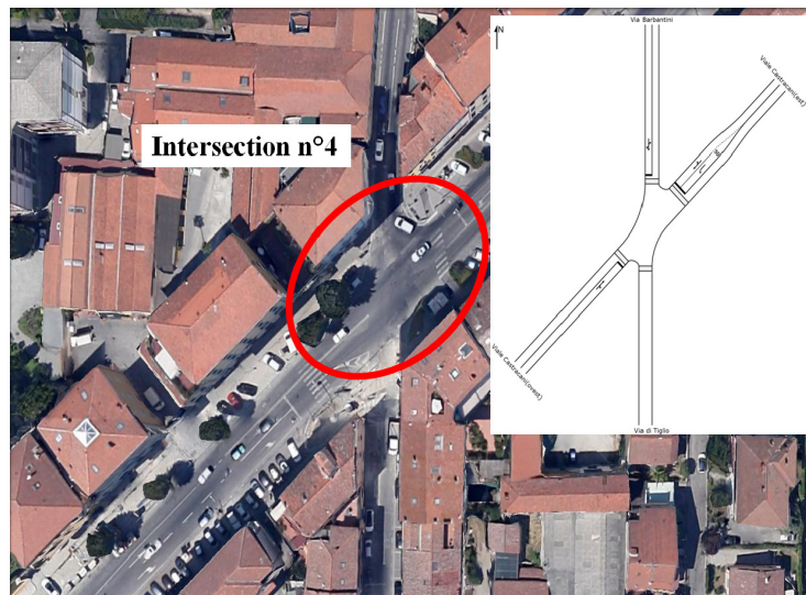
Figure 4: Intersection n°4 and the SIDRA layout picture.
