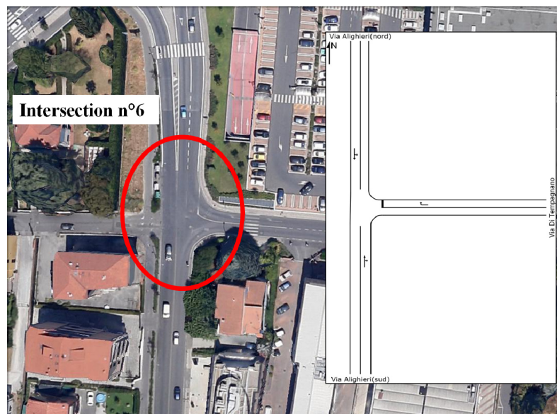
Figure 6: Intersection n°6 and the SIDRA layout picture.
