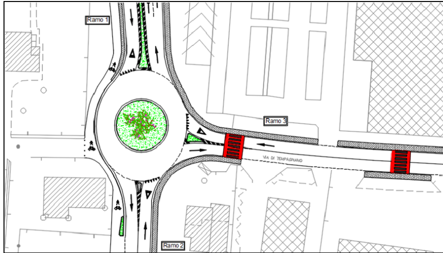
Figure 10: Roundabout at intersection n°6.
