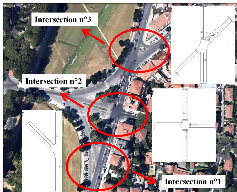
Figure 3: Intersections n°1-2-3 and the SIDRA layout pictures.
