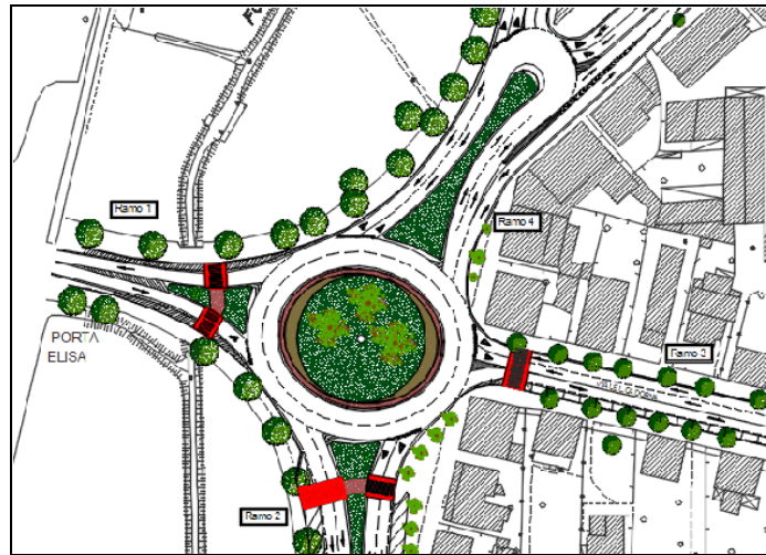
Figure 8: Porta Elisa's roundabout.
