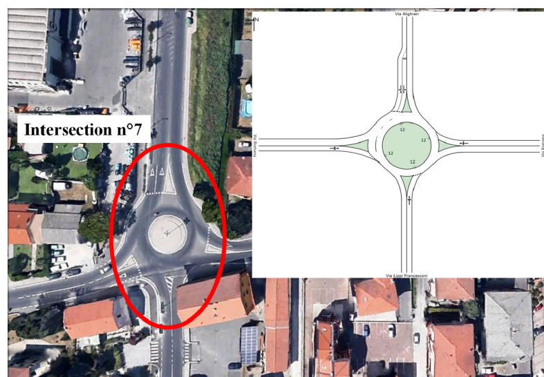
Figure 7: Intersection n°7 and the SIDRA layout picture.
