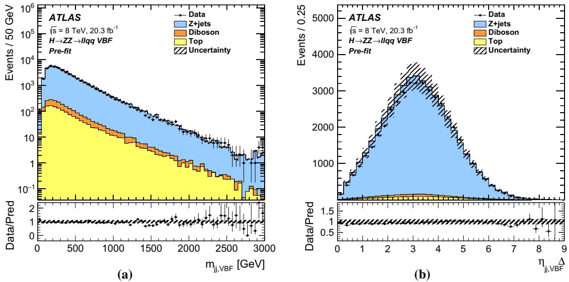
Fig. 5 Distribution of a invariant mass and b pseudorapidity gap for the VBF-jet pair in the VBF channel of the H \rightarrow ZZ \rightarrow \ell^+\ell^-q\bar{q} search before applying the requirements on these variables (and prior
