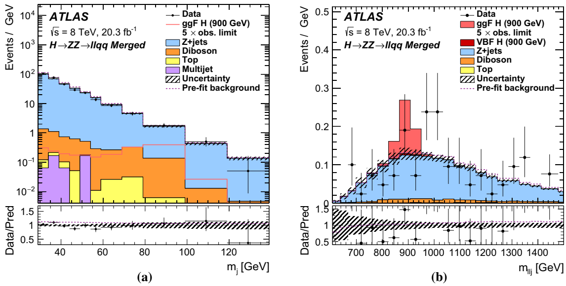
Fig. 4 Distributions for the merged-jet channel of the H \rightarrow ZZ \rightarrow \ell^+\ell^-q\bar{q} search after the mass calibration. a The invariant mass of the leading jet, m_j , after the kinematic selection for the \ell\ell q\bar{q} merged-jet channel. b The distribution used in the likelihood fit of the invariant mass of the two leptons and the leading jet m_{\ell\ell j} in the signal region. It is obtained requiring 70 < m_j < 105 GeV. The dashed line shows
