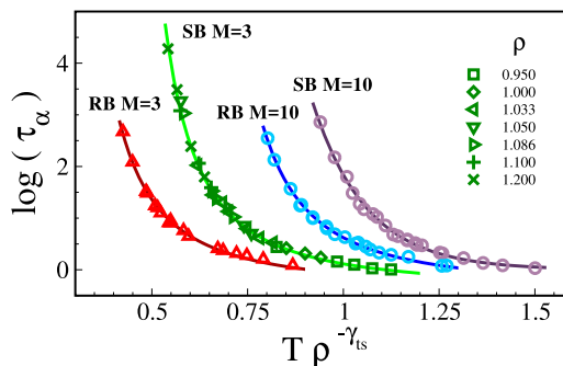
FIG. 10. TS of the structural relaxation time \tau_\alpha from MD simulations of chains with length M = 3, 10 , LJ non-bonding potential, and rigid bonds (RB) or semi-rigid bonds (SB). The states span the ranges 0.95 \leq \rho \leq 1.2 , 0.5 \leq T \leq 1.0 . Details are found in Appendix A2 of Ref. 27. For illustrative purpose, the density of the states of the trimers with SB is shown. For clarity reasons, data are horizontally shifted: RB M = 3 (shift = +0.0), SB M = 3 (shift = +0.2), RB M = 10 (shift = +0.4) and SB M = 10 (shift = +0.6). The continuous line is Eq. (17) with parameters from Table I and \alpha = -0.424(1) , \beta = 2.7(1) \cdot 10^{-2} , \gamma = 3.41(3) \cdot 10^{-3} . 72 No adjustment is done. The TS exponent \gamma_{ts} is equal to the corresponding one of the fast mobility. All the quantities are in reduced MD units.
