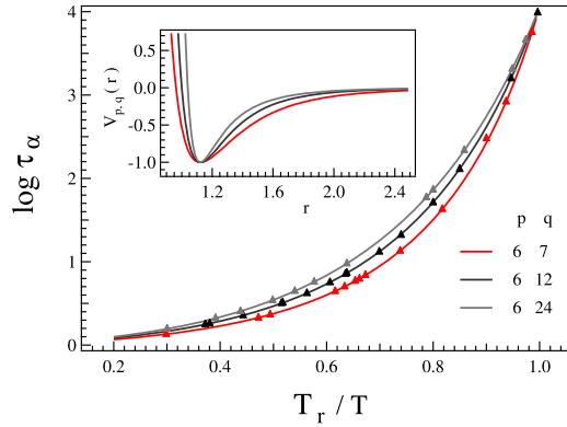
FIG. 2. Reduced temperature dependence of the relaxation time from MD simulations of SB trimers ( M = 3 ) with different forms of the interaction potential between non-bonded monomers, Eq. (4) (insert). T_r is the temperature where \tau_\alpha = 10^4 . The number density is \rho = 1.033 . The fragility increases by decreasing the steepness of the potential around the minimum. The lines are Eq. (17) with parameters as given in Table I and \alpha = -0.424(1) , \beta = 2.7(1) \cdot 10^{-2} , \gamma = 3.41(3) \cdot 10^{-3} . 72 All the quantities are in reduced MD units.
