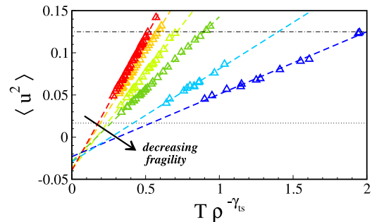
FIG. 6. TS of the fast mobility from MD simulations of SB trimers with different non-bonding potential, Eq. (4) ( p = 6, q = 7, 8, 10, 12, 18, 24 ). They exhibit decreasing fragilities with increasing q values, see Fig. 2. The dashed lines are the master curves Eq. (14) with parameters listed in Table I. The dotted line marks \langle u_g^2 \rangle \approx 0.0166 , the fast mobility at the glass transition. 72 The dotted-dashed line marks the maximum fast mobility in the presence of caging, \langle u_m^2 \rangle = 0.125 , see Sec. III A 1. The extrapolated master curves intersect approximately at (0.08, -0.02) . All the quantities are in reduced MD units.
