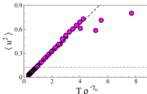
FIG. 9. TS of the fast mobility from MD simulations of the trimer with SB and LJ non-bonding potential for high T \rho^{-\gamma_{ts}} values. For \langle u^2 \rangle > \langle u_m^2 \rangle = 0.125 the cage effect disappears, see Sec. III A 1. The linear TS master curve, Eq. (14), is also drawn (dashed line) with parameters as in Table I. Note that Eq. (14) approximates the TS master curve also in part of the region with no cage effect. All the quantities are in reduced MD units.
