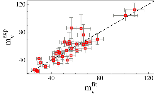
FIG. 15. Correlation plot between the best-fit value of the isochoric fragilities evaluated according to Eq. (22) and the experimental one (Pearson correlation coefficient R = 0.89 ). The dashed line is the bisectrix.
