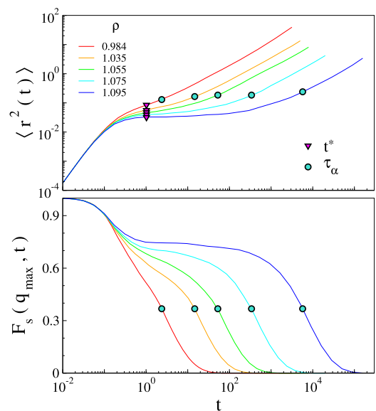
FIG. 1. Monomer MSD, Eq. (6) (top) and corresponding ISF, Eq. (7) (bottom) from MD simulations of the SB trimers with LJ non-bonding potential at T = 0.6 and different densities. The triangles and dots mark the positions of the inflection point in the MSD ( t^* ) and the relaxation time ( \tau_\alpha ), respectively. All the quantities are in reduced MD units.
