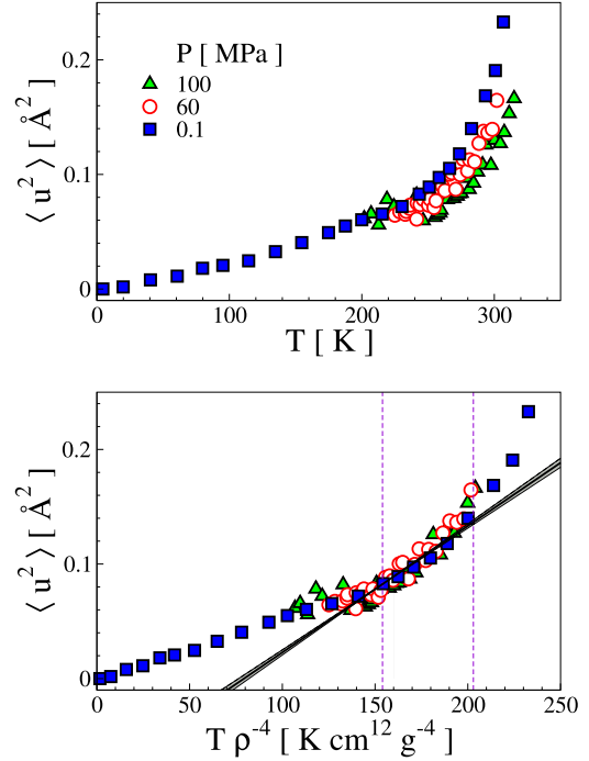
FIG. 16. Top: Fast mobility of OTP from incoherent elastic scattering intensity S(Q, 0) as a function of temperature for different pressures. 135 Bottom: TS of the data with \gamma_{ts} = 4 (equation of state from Ref. 132). The vertical dashed lines mark the glass transition ( \tau_\alpha = 10^2 s, T_g \rho_g^{-\gamma_{ts}} = 154 K cm 12 g -4 , \langle u_g^2 \rangle = 0.0829 Å 2 ), and the critical value T_c \rho_c^{-\gamma_{ts}} above which the quasielastic broadening from structural relaxation contribution, being \tau_\alpha = 20 ns, has to be taken into account 135 and the measured \langle u^2 \rangle cannot be longer interpreted as the fast mobility within the cage. The thick solid line is Eq. (18) with \kappa evaluated from Eq. (22) with \tilde{m}_v = m_v^{exp} , as taken from Table II. The two thin black lines bound the uncertainty on the slope due to the one on m_v^{exp} .
