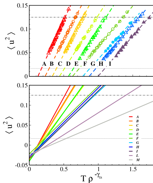
FIG. 7. Top: TS of the fast mobility from MD simulations of SB and RB polymer chains with different chain length M and non-bonding potential U_{q,p} , Eq. (4). For clarity reasons, data are horizontally shifted. A: SB M = 3 , p, q = 6, 7 (shift: +0.0); B: SB M = 10 , p, q = 6, 8 (+0.1); C: SB M = 3 , p, q = 6, 8 (+0.2); D: SB M = 10 , p, q = 6, 10 (+0.3); E: SB M = 3 , p, q = 6, 10 (+0.4); F: SB M = 10 , p, q = 6, 12 (+0.5); G: RB M = 10 , p, q = 6, 12 (+0.6); H: SB M = 3 , p, q = 6, 12 (+0.7); I: RB M = 3 , p, q = 6, 12 (+0.8). The dashed lines are the master curves Eq. (14) with parameters listed in Table I. The dotted line marks \langle u_g^2 \rangle \approx 0.0166 , the fast mobility at the glass transition. 72 The dotted-dashed line marks the maximum fast mobility in the presence of caging, \langle u_m^2 \rangle = 0.125 , see Sec. III A 1. Bottom: Approximated common intersection of all the TS master curves. For clarity reasons, MD points are removed. Details about the L and M lines, the two lines with smaller slope in Fig. 6, are given in Table I. All the quantities are in reduced MD units.
