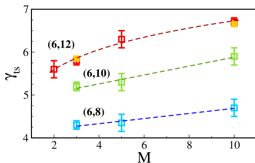
FIG. 8. Scaling exponent \gamma_{ts} versus chain length M from MD simulations of polymer systems with either SB (open symbols) or RB (full symbols) and different non-bonding potential, Eq. (4), as indicated by the (p, q) pairs in parenthesis. The dashed lines are guides for the eyes. The exponent \gamma_{ts} increases with: (i) the chain length and (ii) the steepness of the non-bonding potential around the minimum, see Fig. 2.
