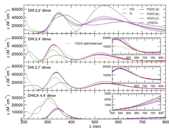
Figure 8. Computed absorption spectra for the HQ (green), Q (red) and HQ/Q (indigo, averaged over three conformers) species of the investigated dimers. The absorption of each HQ/Q stacked conformer at short (a), minimum (b) and large (c) distance, is reported separately. In the insets, the visible region between 500 and 800 nm is highlighted.
