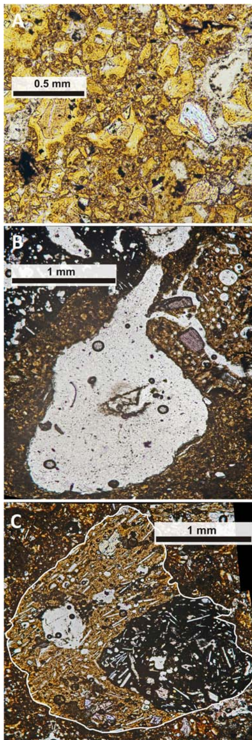
Fig. 5 Photomicrographs of Harrow Peaks lapilli tuffs. a Fine–medium ash matrix to lapilli tuff showing blocky sideromelane shapes. b Matrix vesicle in fine ash matrix of lapilli tuff. c Abraded tachylite clast within sideromelane lapillus
