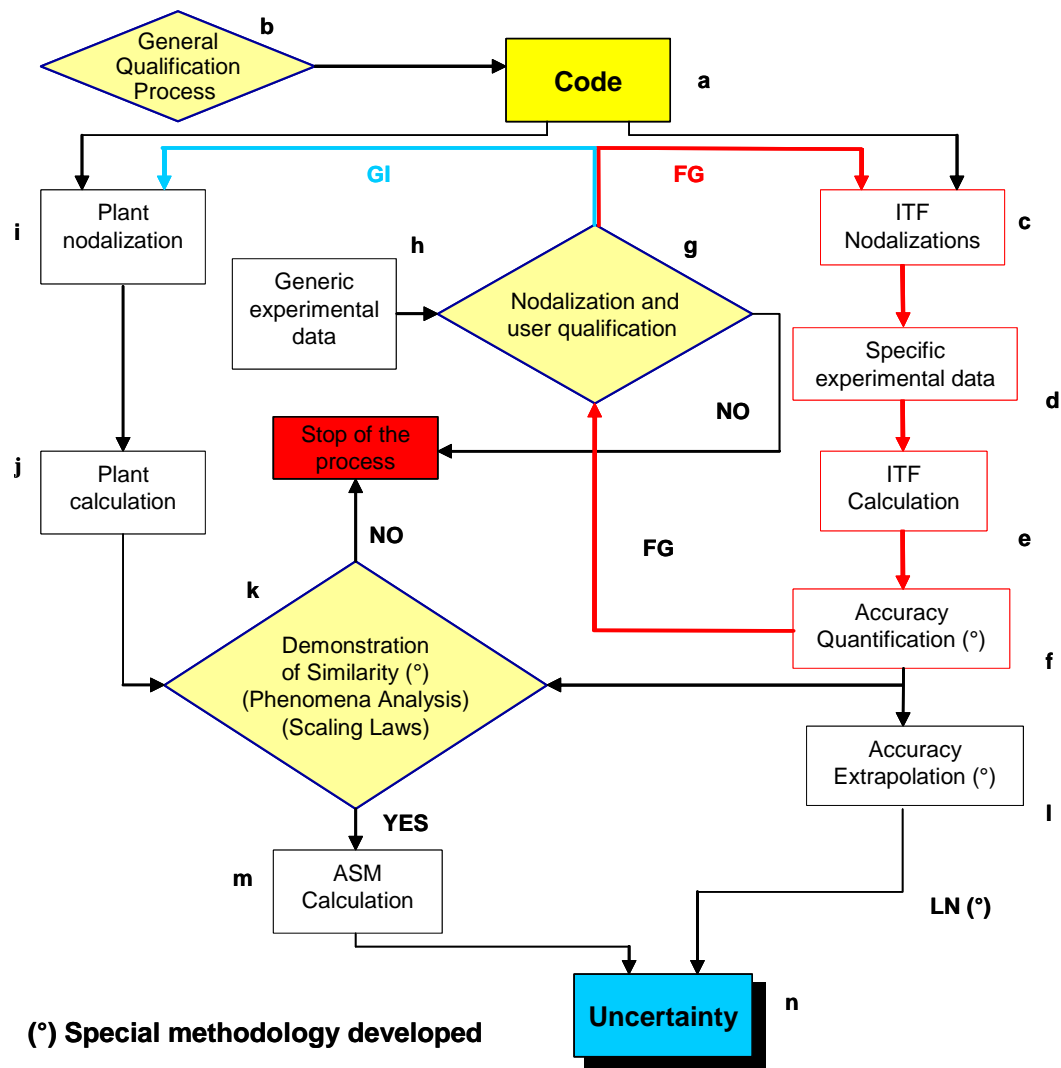
Figure 3. The flow-diagram of UMAE.
