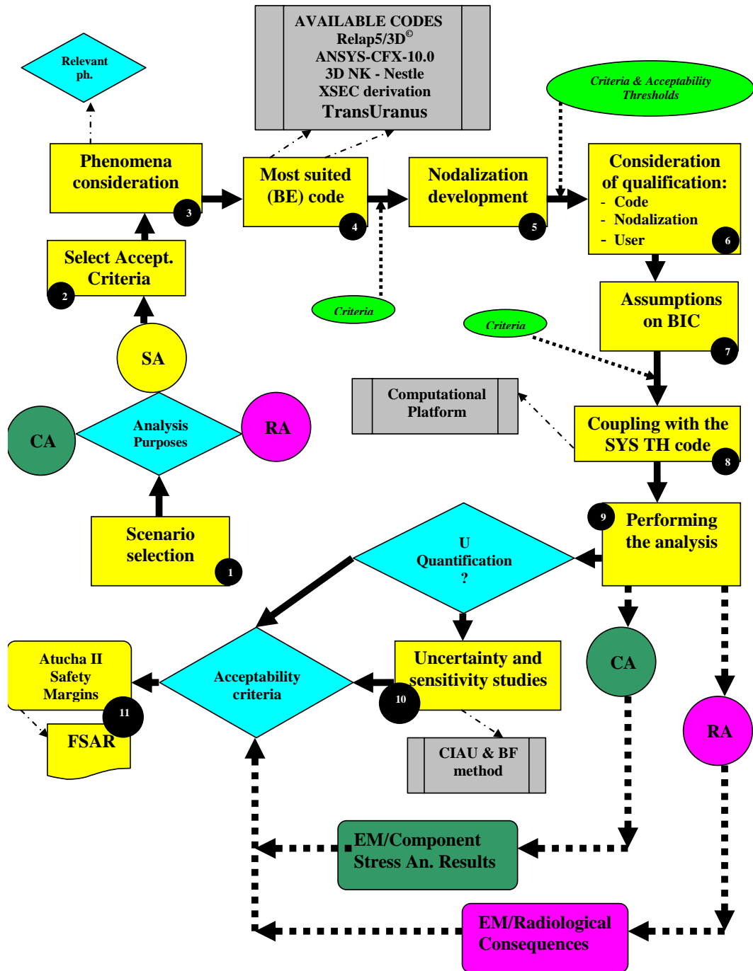
Figure 1 – The BEPU flow-diagram.
