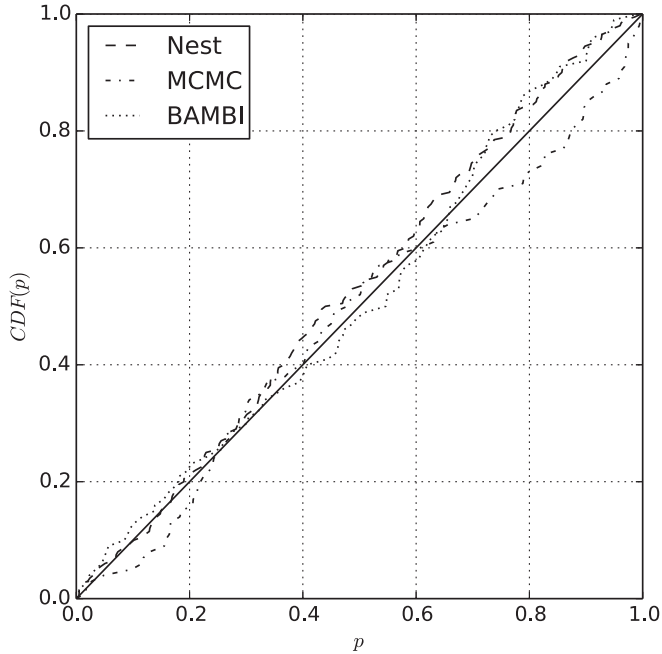
FIG. 10. P versus P plot for the distance parameter. On the x axis is the probability p contained in a credible interval, and on the y axis the fraction of true values which lay inside that interval. The diagonal line indicates the ideal distribution where credible intervals perfectly reflect the frequency of recovered injections. For all three sampling algorithms the results are statistically consistent with the diagonal line, with the lowest KS statistic being 0.25.
