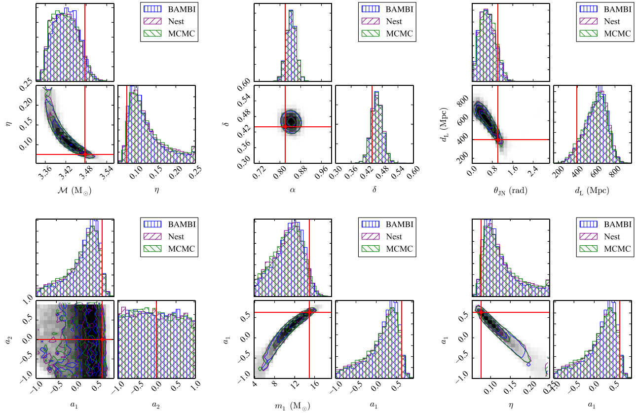
FIG. 8 (color online). Comparison of probability density functions for the NSBH signal (Table II), with the same color scheme as Fig. 7. (First row left) The mass posterior distribution parametrized by chirp mass and symmetric mass ratio. (First row center) The location of the source on the sky. (First row right) The distance d_L and inclination \theta_{JN} of the source. In this case the V-shaped degeneracy is broken, but the large correlation between d_L and \theta_{JN} remains. (Second row left) The spin magnitudes posterior distribution. (Second row center) The spin and mass of the most massive member of the binary illustrating the degeneracy between mass and spin. (Second row right) The spin and symmetric mass ratio.
