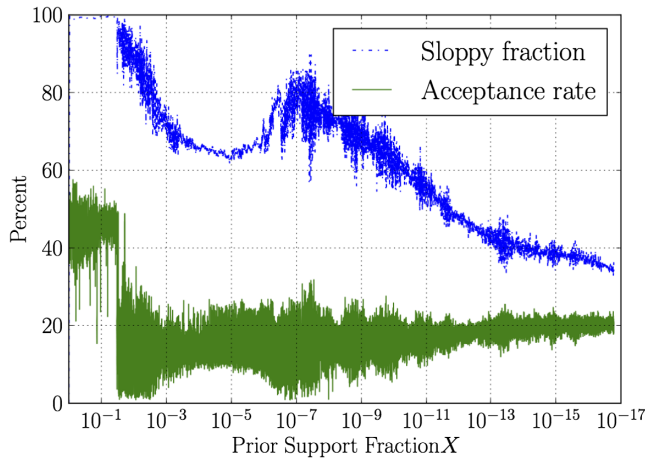
FIG. 4 (color online). Acceptance ratio and fraction of sloppy jumps for nested sampling analysis of a BNS system. The dashed blue line shows the automatically determined fraction of proposals for which the likelihood calculation is skipped. The solid green line shows the overall acceptance rate for new live points, which thanks to the adaptive jumps remains at a healthy level despite the volume of the sampled distribution changing by 17 orders of magnitude throughout the run.
