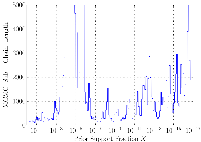
FIG. 3 (color online). Length of MCMC subchain for nested sampling analysis of the BNS system (as in Table II) as a function of prior scale. As the run progresses, the length of the MCMC subchain used to generate the next live point automatically adapts to the current conditions, allowing it to use fewer iterations where possible. The chain is limited to a maximum of 5000 iterations.
