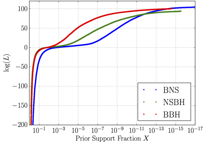
FIG. 2 (color online). The profile of the likelihood function for each of the injections in Table II, mapped onto the fractional prior support parameter X [see Eq. (28)]. The algorithm proceeds from left (sampling entire prior) to right (sampling a tiny restricted part of the prior). The values of \log(L) are normalized to the likelihood of the noise model.
