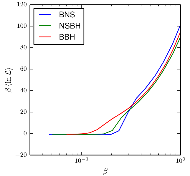
FIG. 5 (color online). The integrand of the evidence integral [Eq. (41)] versus \beta for the analyses of synthetic GW signals in § VB. The evidence is given by the area under each curve. Table I gives the results of the integration together with the estimated error in the quadrature, following the procedure described in § IV C. The jaggedness of the curves illustrates that the temperature spacing required for convergent MCMC simulations is larger than that required for accurate quadrature to compute the evidence; the flatness at small \beta illustrates that, for these simulations, the high-temperature limit is sufficient for convergence of the evidence integral.
