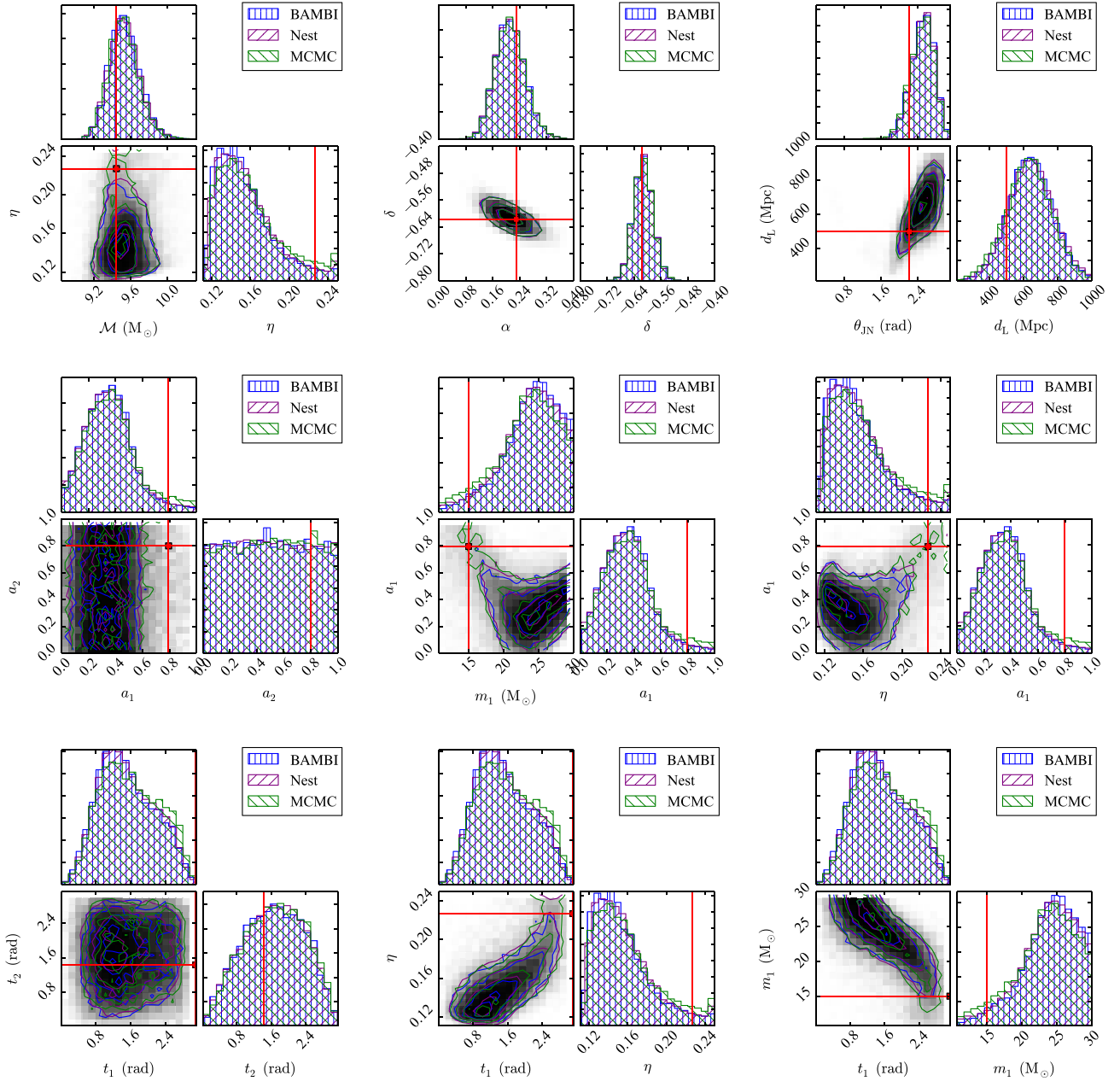
FIG. 9 (color online). Comparison of probability density functions for the BBH signal (Table II), with the same color scheme as Fig. 7. (First row left) The mass posterior distribution parametrized by chirp mass and symmetric mass ratio. (First row center) The location of the source on the sky. (First row right) The distance d_L and inclination \theta_{JN} of the source where the degeneracy is broken, as in the NSBH case. (Second row left) The spins magnitude posterior distribution. (Second row center) The spin and mass of the most massive member of the binary illustrating the degeneracy between mass and spin. (Second row right) The spin and symmetric mass ratio. (Third row left) The spins tilt posterior distribution. (Third row center) The spin tilt of the more massive member of the binary and the symmetric mass ratio. (Third row right) The spin tilt and mass of the most massive member of the binary.
