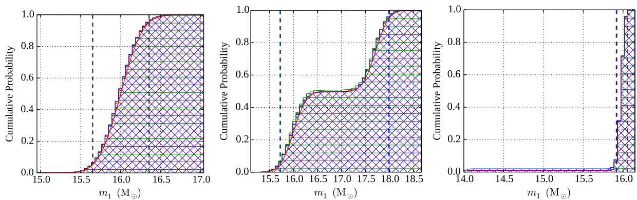
FIG. 6 (color online). Example comparing cumulative distributions for the analytic likelihood functions for each sampler for the (arbitrary) m_1 parameter for the three test likelihood functions. The samplers are shown as Nest: purple left hatches; MCMC: green horizontal hatches; BAMBI: blue right hatches, with the true cumulative distributions shown in red where available. (Left) Unimodal multivariate Gaussian distribution. (Middle) Bimodal distribution. (Right) Rosenbrock distribution. The different methods show good agreement with each other, and with the known analytic distributions. Vertical dashed lines indicate the 5–95% credibility interval for each method.
