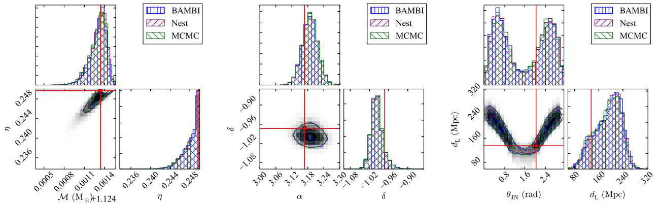
FIG. 7 (color online). Comparison of probability density functions for the BNS signal (Table II) as determined by each sampler. Shown are selected two-dimensional posterior density functions in greyscale, with red cross hairs indicating the true parameter values, and contours indicating the 90% credible region as estimated by each sampler. On the axes are superimposed the one-dimensional marginal distributions for each parameter, as estimated by each sampler, and the true value indicated by a vertical red line. The colors correspond to BAMBI (blue), NEST (magenta), MCMC (green). (Left) The mass posterior distribution parametrized by chirp mass and symmetric mass ratio. (Center) The location of the source on the sky. (Right) The distance d_L and inclination \theta_{JN} of the source showing the characteristic V-shaped degeneracy.
