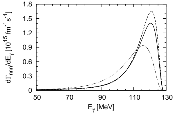
FIG. 13. The same as in Fig. 8 for the differential capture rate d\Gamma_{nnn}/dE_\gamma in the case of the \pi^- + {}^3\text{H} \rightarrow \gamma + n + n + n process.
