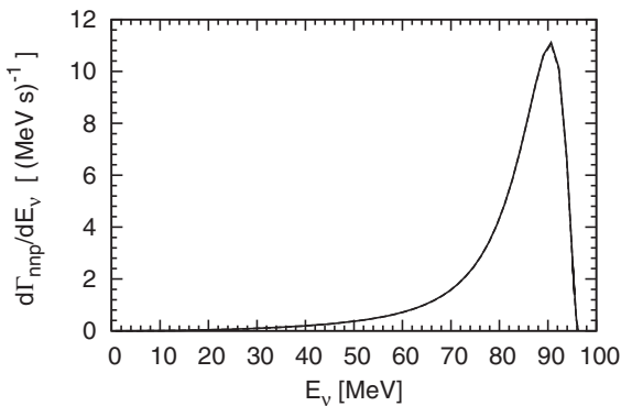
FIG. 10. The differential capture rates d\Gamma_{nnp}/dE_\nu for the \mu^- + {}^3\text{He} \rightarrow \nu_\mu + n + n + p process calculated with the AV18 potential [13] and using a full solution of Eq. (5.9) with V_4^{(1)} = 0 . The curves representing results of the calculations employing all partial-wave states with j \leq 3 ( j \leq 4 ) in the 2N subsystem are depicted with dashed (solid) curves. The maximal total 3N angular momentum is J_{\max} = \frac{9}{2} .
