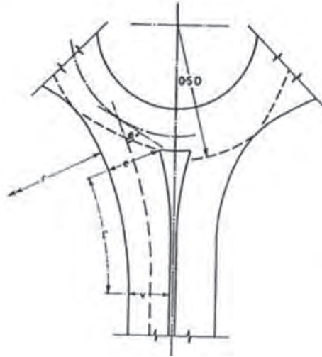
Figure 5: Geometric features for Kimber's model.
