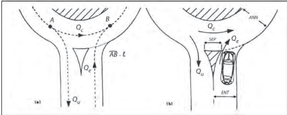
Figure 6: Notations and symbols for CERTU (a) and SETRA (b) models.
