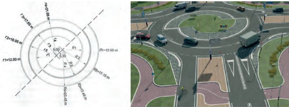
Figure 3: A geometric turbo block (left) and a rendering of a turbo roundabout (right).
