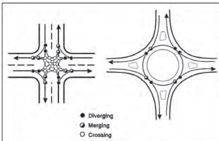
Figure 1: Conflict points in a single-lane roundabout vs. a yield-controlled intersection [1].
