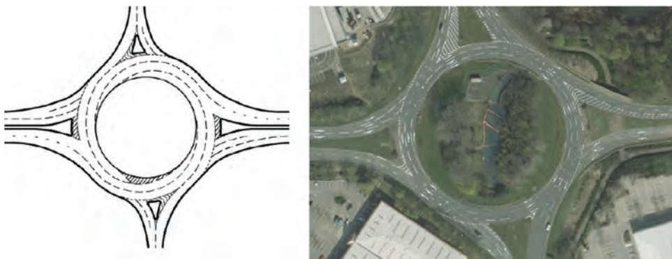
Figure 2: Spiral roundabout layout (left) and the spiral roundabout (right) at the junction of H10 and V7 in Milton Keynes (UK) (left hand circulation).
