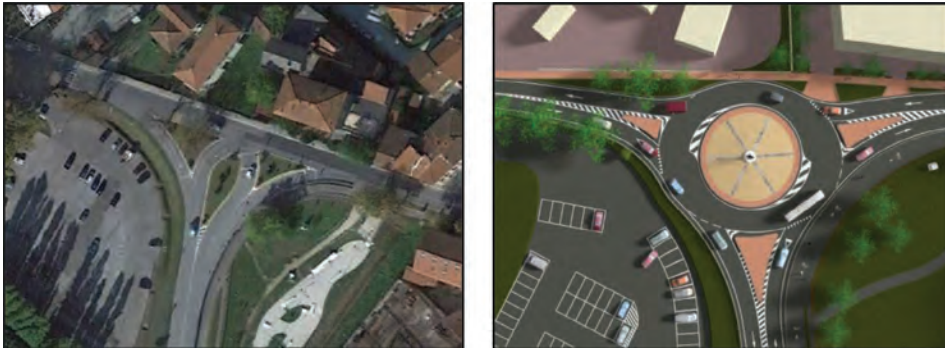
Figure 4: Example of conversion of a ‘T’ intersection (left) into a two-geometry roundabout. Left: the ‘T’ junction. Right: the designed 2-G roundabout layout: major axis (a) = 38 m (125 ft); minor axis (b) = 31 m (102 ft); b/a ratio = 0.82; central island radius = 8.5 m (28 ft); circulating carriageway width = minimum 5.0 m (16 ft)–maximum 8.5 m (28 ft).
